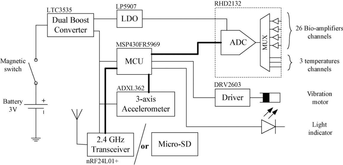
Fig. 4. Functional diagram of the complete instrumentation
