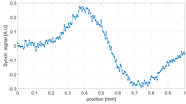
Figure 4.8: Error signal obtained for the phase scan.
