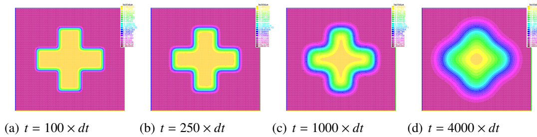
FIGURE 5.4 – k = 1, dt = 10^{-6} .
