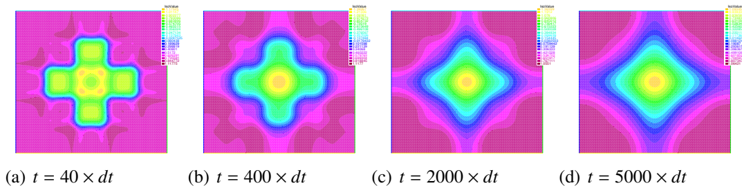
FIGURE 5.11 – k = 2 , dt = 10^{-7} .
