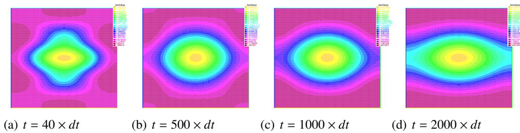
FIGURE 5.10 – k = 3 , dt = 10^{-8} .
