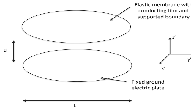
FIGURE 9.1 – An idealized MEMS capacitor.
