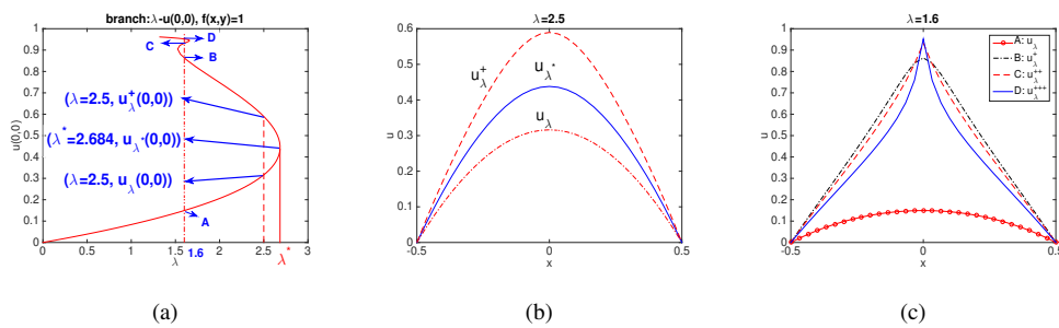
FIGURE 9.4 – The branch of solutions u(0, 0) as a function of \lambda : (a) f(x, y) \equiv 1 ; (b) \lambda = 2.5 , u_\lambda , u_{\lambda^*} and u_\lambda^+ ; (c) \lambda = 1.6 , four corresponding solutions.
