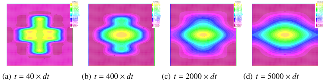
FIGURE 5.9 – k = 2 , dt = 10^{-7} .
