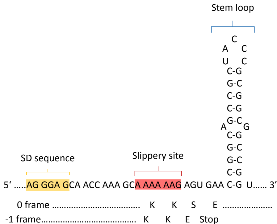
Figure 3: Signals of dnaX programmed frameshifting. The sequence of dnaX mRNA is represented with the SD-like sequence in the yellow box, the slippery sequence in the red box and the stem loop. The protein sequence in the canonical frame (0 frame) is indicated below as well as the sequence in the -1 frame following frameshifting (adapted from Caliskan et al. , 2015).
