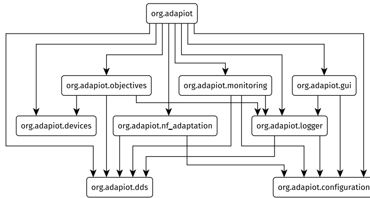
Figure 6.3 – Implementation dependency graph
