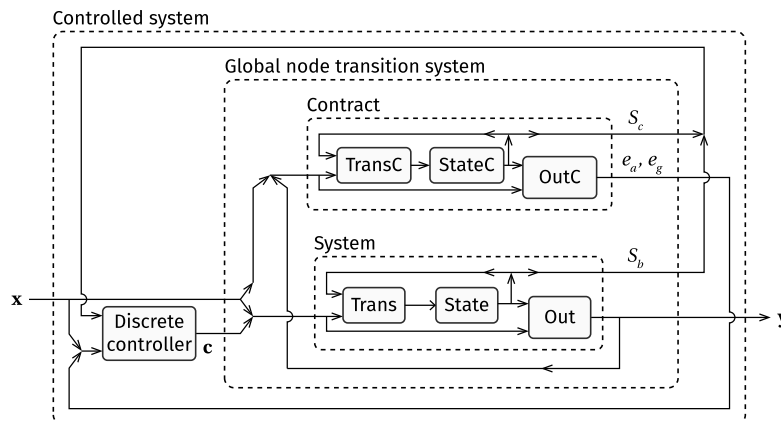
Figure 5.7 – Discrete controller synthesis workflow, adapted from [DMR10]
