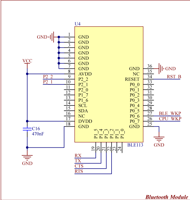
Figure B.4 – BLE113 interfacing
