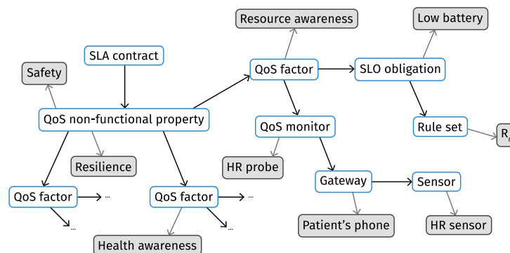
Figure 5.2 – SLA ontology
