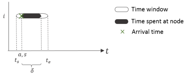
Figure 6.3.4: Illustration of parameters used in ILS. The following notations are used: a - arrival time, s - service start time, t_s - opening of the time window, t_e - closing of the time window,
