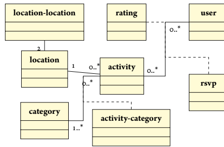
Figure 9.3.1: Conceptual diagram of Fantasy_db.
