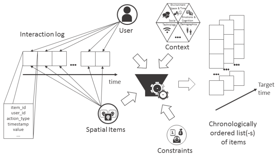
Figure 3.3.2: High-level overview of problems of recommendation of sequences of spatial items.
