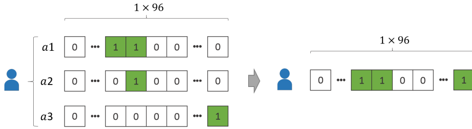
Figure 7.2.2: User's temporal profile.
