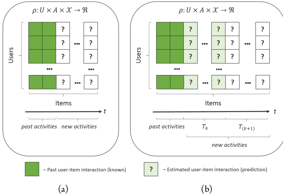
Figure 7.2.4: Computational strategies: (a) Strategy 1 - All-at-once, (b) Strategy 2 - Day-after-Day.
