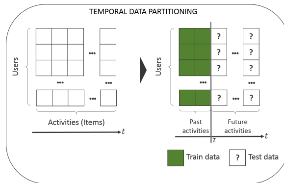
Figure 11.1.1: Data partitioning.
