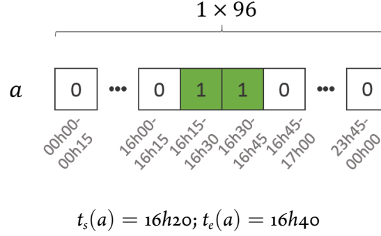
Figure 7.2.1: Representation of an activity as a binary time vector. The activity starts at 16h20 and ends at 16h40.
