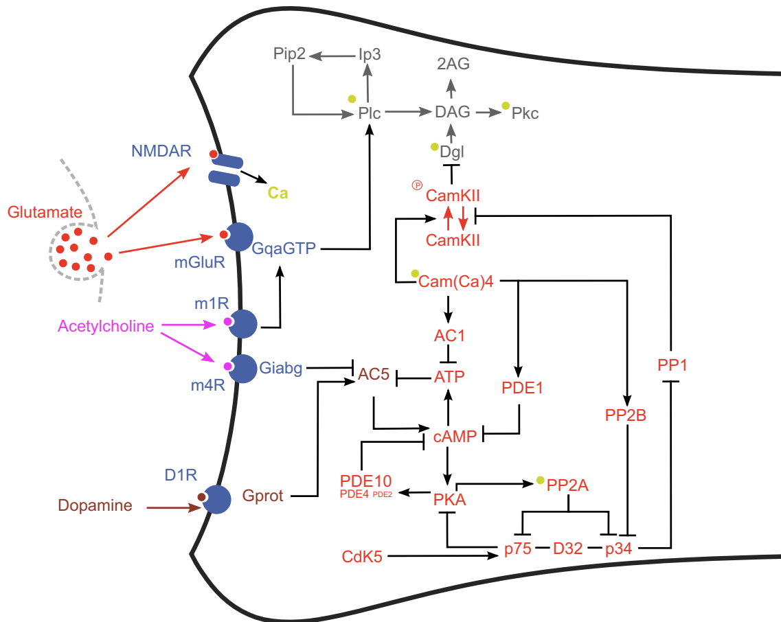
Figure 5.2: Scheme of the modelled signaling network of Blackwell's team. Color code: receptors: dark blue; PLC and IP3 pathways: gray; calcium pathways: green (green disks indicate calcium-dependent steps). Abbreviations: PKc: protein kinase C; PDE: phosphodiesterase; PP2A: protein phosphatase 2A; PP2B: protein phosphatase 2B or calcineurine; Cdk5: Cyclin-dependent kinase 5; D32p34: DARPP32 phosphorylated at Thr34; D32p75: DARPP32 phosphorylated at Thr75; see figure 5.1 for other abbreviations.
