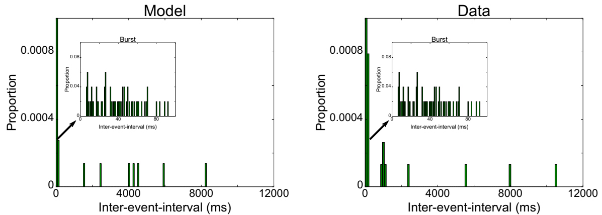
Figure 4.9: Irregular bursting cells model (left) and data (right). The inter-burst interval timing, t_{inter-burst} , follows a Rayleigh distribution, with parameters \alpha = -1660 and \beta = 4598 , we discarded all negative output values. The intra-burst interval timing is calculated with an exponential function where parameter a is uniformly distributed (a_{down}, a_{up}) = (7.5, 42.) , and b is set at 0.15 and where the number of spikes is an integer uniformly distributed in [1, 13] .
