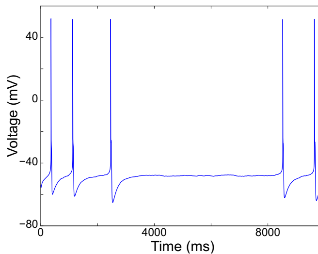
Figure 4.19: DA neuron in irregular spiking mode at around 0.5 Hz where there is no NMDA current and GABA current is irregular with conductance set at 4 \mu S.cm^{-2} .
