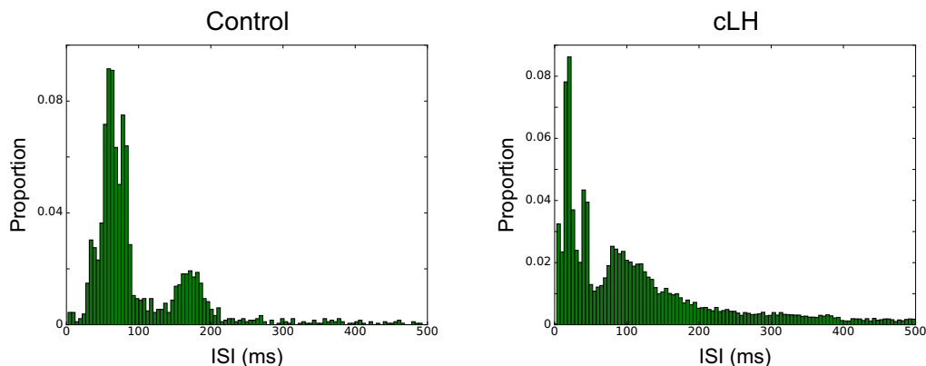
Figure 4.17: ISI histograms of experimental data. Control condition (left panel) and cLH condition (right panel).
