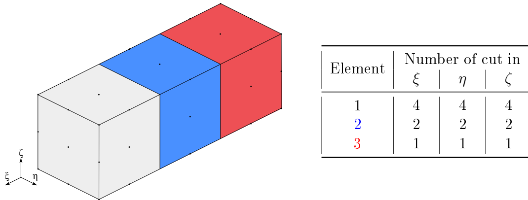
Fig. 3.19: Initial mesh and refinement instructions.
