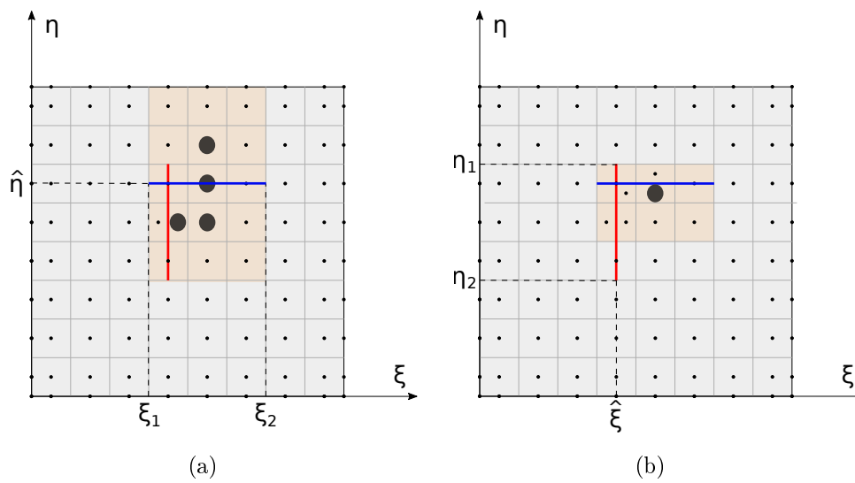
Fig. 3.8: Crossed refinement: a) The blue mesh line traverses entirely the support of 4 functions at \hat{\eta} b) One of the resulting functions of the blue mesh line is cut by the existing red mesh line of Figure 3.7(a)
