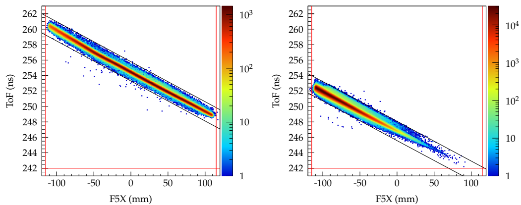
(B) ^{41}\text{Al}
