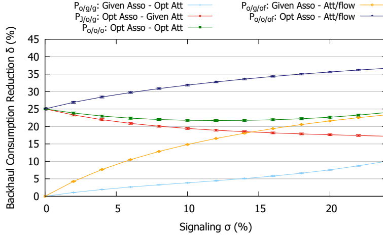
Figure 5.11: The average relative backhaul bandwidth consumption reduction \delta function of \sigma , in P_{o/g/o} , P_{J/o/g} , P_{o/o/o} , P_{o/g/of} , and P_{o/o/of} , for different network topologies.
