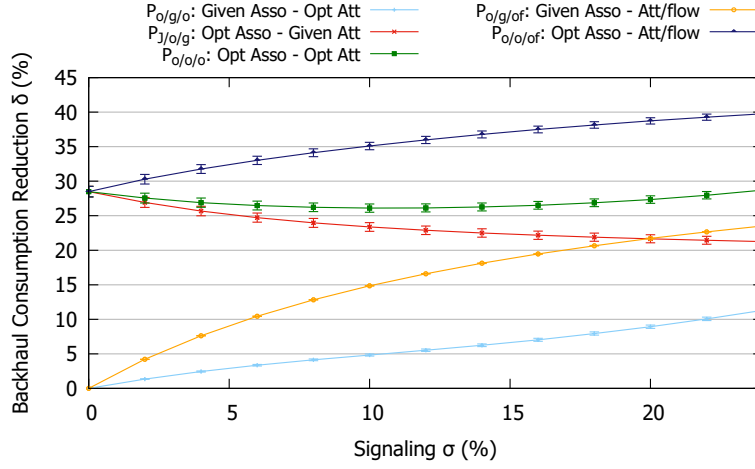
Figure 5.10: The relative backhaul bandwidth consumption reduction \delta function of \sigma , in P_{o/g/o} , P_{J/o/g} , P_{o/o/o} , P_{o/g/of} , and P_{o/o/of} .
