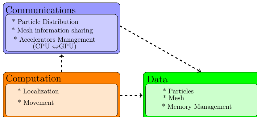
Figure 3.2: Component Graph of the library.
