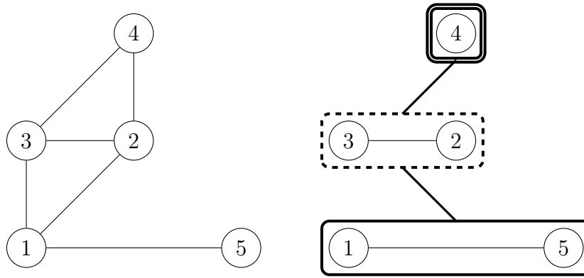
Figure 2.3: A graph and the associated tree
