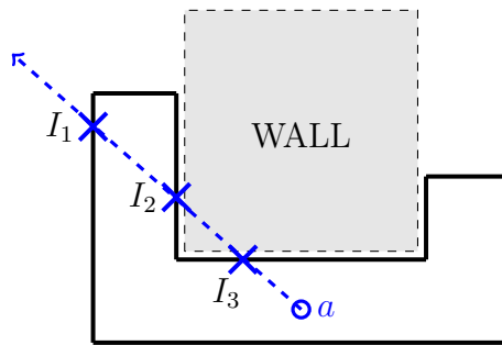
Figure 2.2: Particle intersecting multiple faces of its current cell. Faces are checked in this order : I_1 , I_2 and I_3 .
