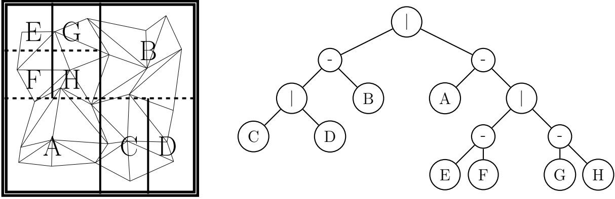
Figure 2.4: Spatial decomposition by Kd-tree.
