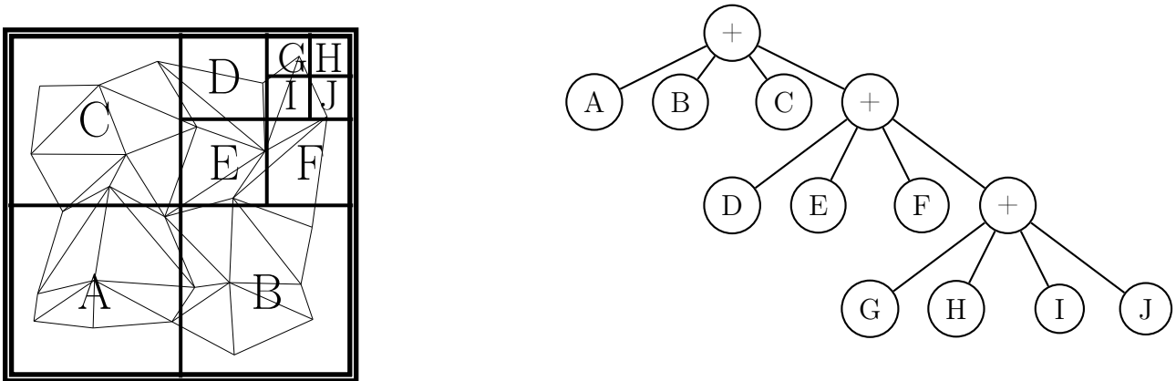
Figure 2.5: Spatial decomposition with Quad-tree.
