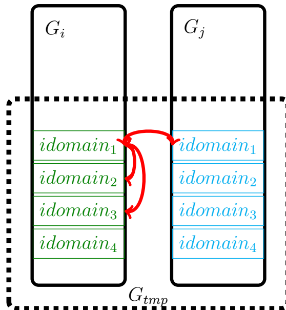
Figure 7.2: G_{tmp} is the temporary group composed with 2 groups G_i and G_j . G_i and G_j are formed with 4 processes each, so G_{tmp} allows these processes to communicate.
