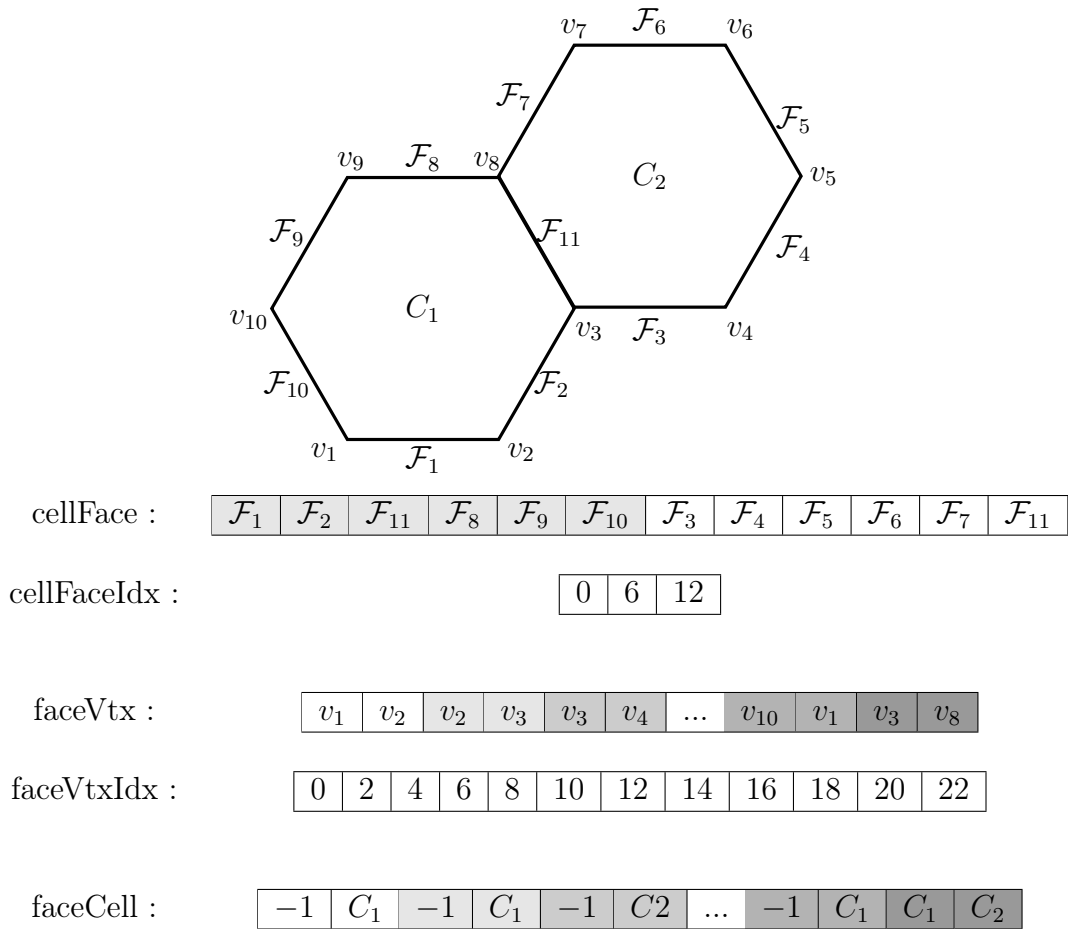
Figure 3.3: Representation and storage method of mesh data.
