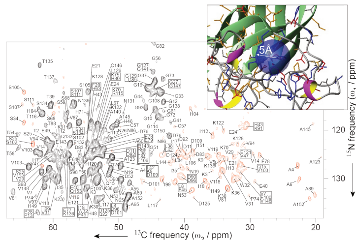
Figure 4. NCACB spectrum of \text{Cu}^{\text{II}},\text{Zn}^{\text{II}} -SOD acquired at 15 kHz MAS rate, and a pictorial representation of the NMR inaccessible region around the Cu ion. Reproduced from reference 13.
