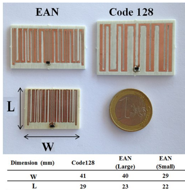
Fig. 14. The realized prototypes on Rogers RO4003™ substrate, Code128 (right) two different sizes of EAN (left).
