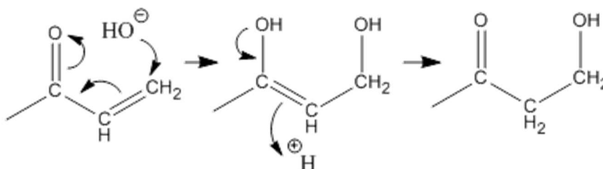
Figure 3-9 Nucleophilic attack on beta unsaturated carbonyl.
