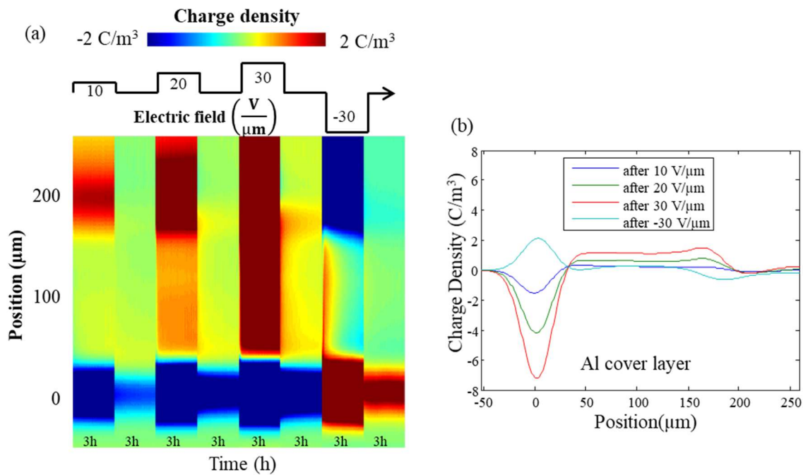
Figure 3-18 Space charge profiles obtained with LDPE realized with Al protecting layer. (a) colour map of time dependence of the profile along the cycle; (b) charge density profiles just after voltage removal.
