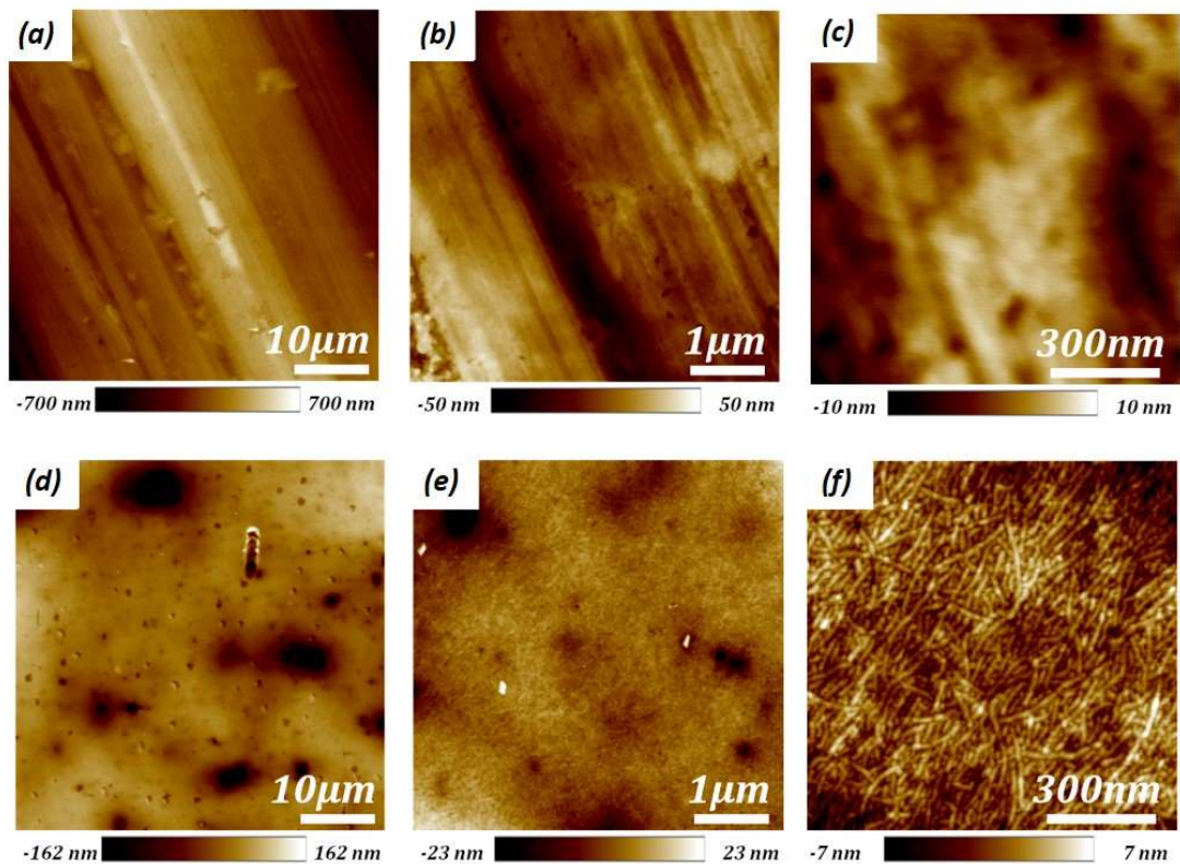
Figure 3-13 Comparison of surface topography measured in PF-QNM of samples processed at ABB site using Al (a-c) or PET (d-f) protecting layers at different scales: (a, d) 50µm x 50µm, (b, e) 5µm x 5µm and (c, f) 1µm x 1µm.
