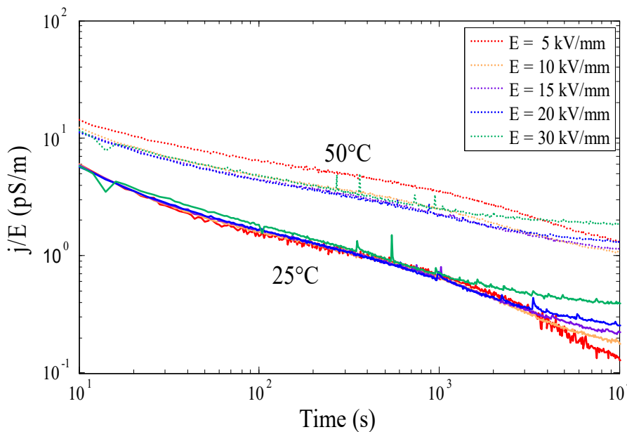
Figure 3-26; Normalized current transients obtained on LDPE processed with PI protecting layers.
