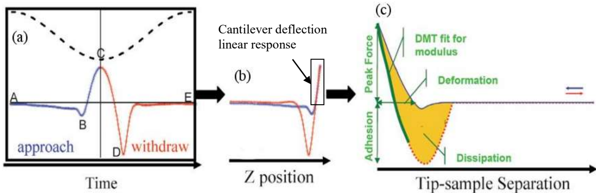
Figure 2-13 Characteristic peak force signals in function of time (a), piezoelectric Z position (b) and force vs. tip-sample separation (c). In Figure (a) the dashed line represents a single time period of the piezoelectric Z position oscillation synchronized to the solid line of the heartbeat signal. In (b) the cantilever deflection signal is correlated to the piezoelectric Z position. In (c), after the calibration process, the force vs. tip-sample separation shows how parameters as DMT modulus, deformation, dissipation, adhesion and peak forces can be determined [Pitt10].
