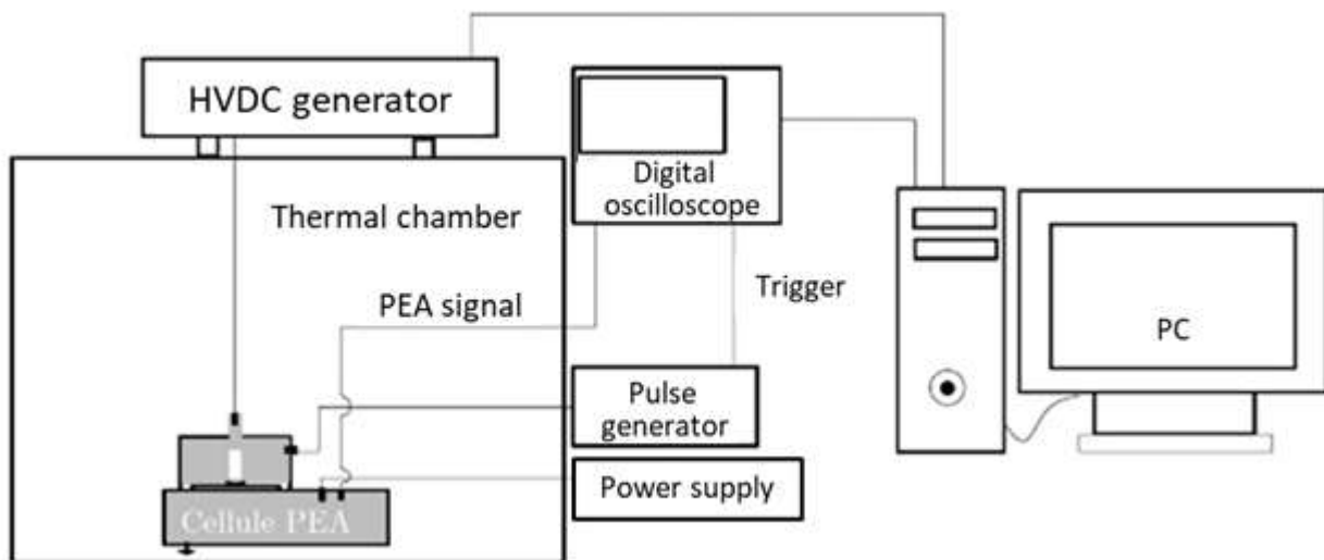
Figure 2-12 Schematic of the PEA setup [Viss11].
