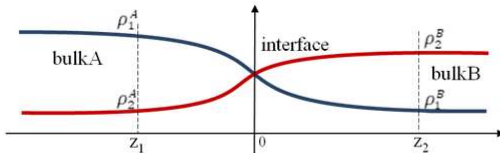
Figure 1-12: Example of interface ( z_2-z_1 ) between the phases A and B, defined by the properties \rho_1 and \rho_2 [Lewi94].
