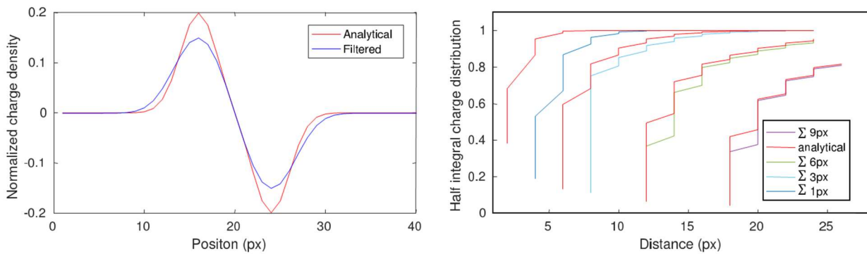
Figure 4-14 Effect of the SG-2D filter on two opposite Gaussian charge density distributions. (a) filter effect on two normal distributions with \Sigma 2 \text{ px} , distance 8 \text{ px} and patch image size 9 \text{ px} . (b) half integral density charge distribution vs peak distance for different standard deviation and patch image size 9 \text{ px} .
