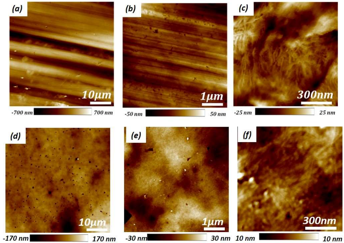
Figure 3-12 Comparison of surface topography measured in PF-QNM of sample processed at Laplace using Al (a-c) or PET (d-f) protecting layers at different scales: (a, d) 50µm x 50µm, (b, e) 5µm x 5µm and (c, f) 1µm x 1µm.
