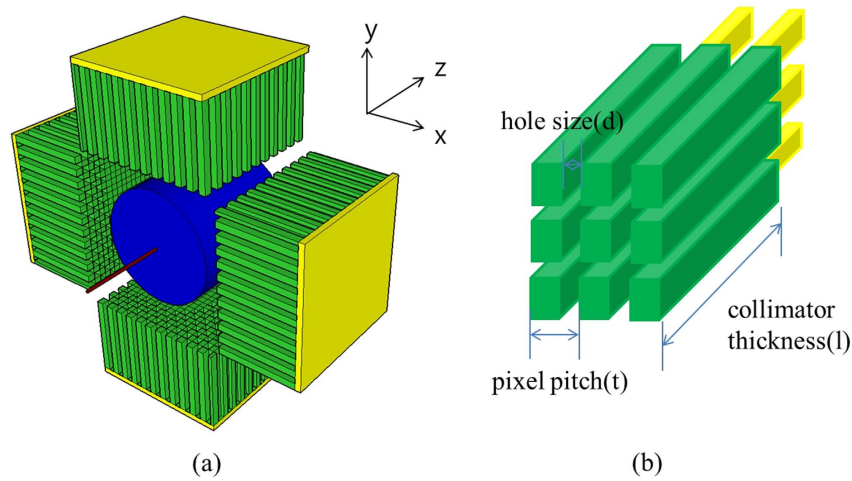
Figure 3.11: An ambitious design proposal: pillar grid collimation with the aim of enabling 3D dose reconstruction through PG imaging. Optimal parameters were found at l = 7 cm, t = 5.5 mm and d = 3 mm. Source: Kim et al. (2016).
