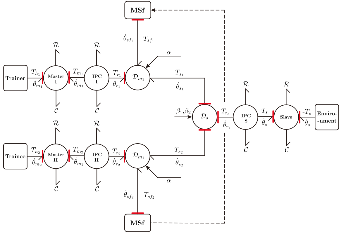
Figure A-10: Port-Hamiltonian representation of ESC dual-user system using bond graphs
