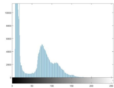
BF histogram
