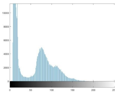
MeF histogram
