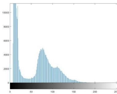
GMF histogram
