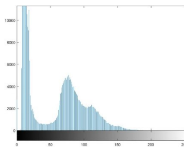
HMF histogram
