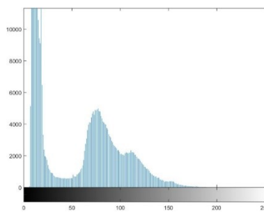
DWT histogram
