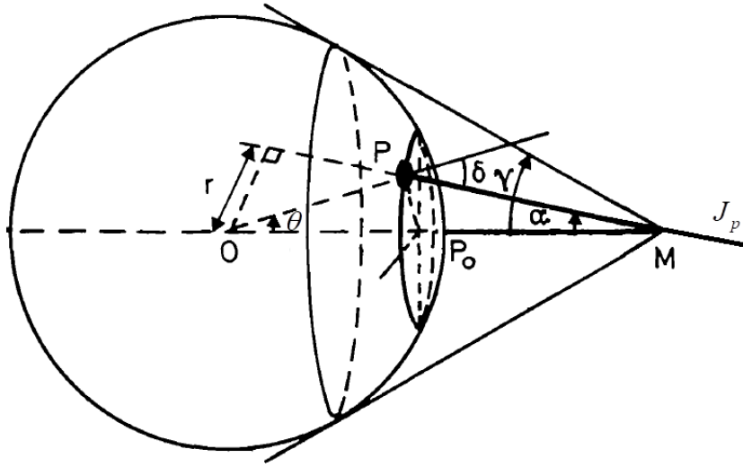
Figure 3.29 Coordinates of the region on the solar surface. P_o is the center of the observed region, M is the scattering point which is located in the prominence. P_oM is the height over the limb (Sahal-Brechot et al., 1986).
