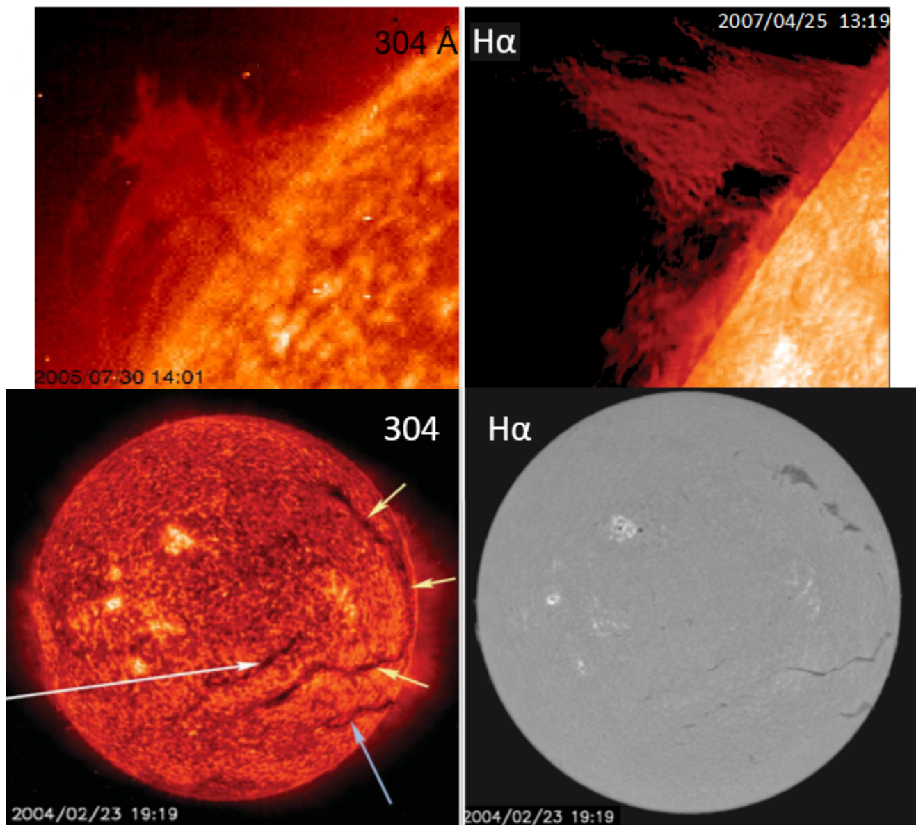
Figure 1.1 Example of prominences and filaments observed in H \alpha and He II 304 Å by SOHO/EIT (top-left panel and bottom-left panel), Hinode/SOT (top-right panel) and Catania Astrophysical Observatory (bottom-right panel). The filaments are pointed with arrows in the bottom-left panel (Lin et al., 2008a; Heinzel et al., 2008; Parenti, 2014).
