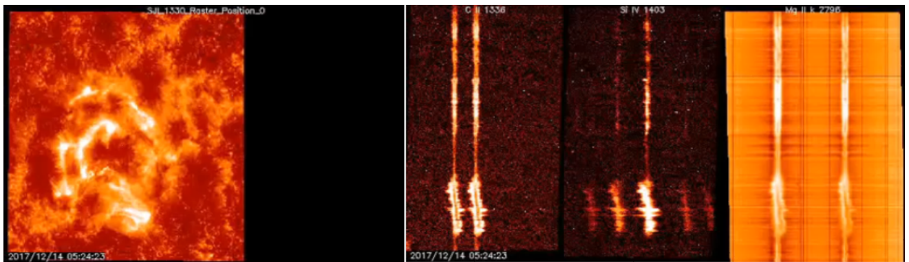
Figure 2.2 IRIS SJI image observed at 05:24 UT on Dec 14 in 1330 Å is shown in the left panel. The slit at the center of the image is crossing the flare region at this time, and the corresponding spectra of C II, Si IV and Mg II k lines are shown in the right panel.
