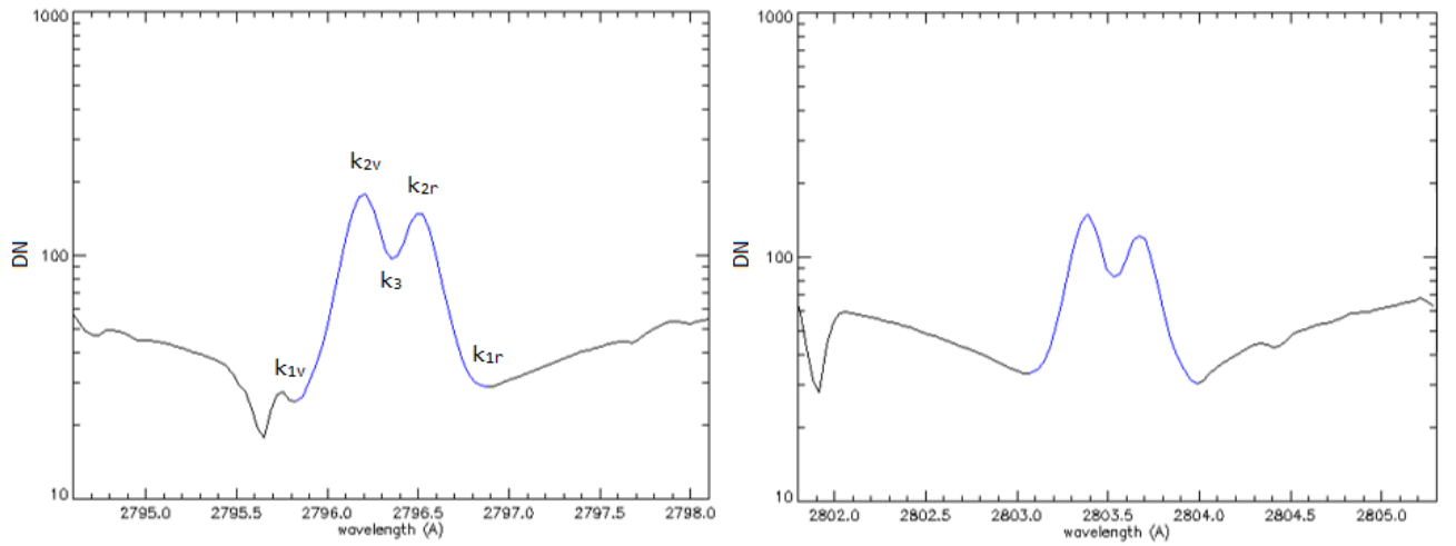
Figure 2.12 Averaged Mg II k (left) and h (right) profiles over a region of 100"×100" at the center of the Sun which corresponds to the region inside the red box in Figure 2.11, with the k_1 , k_2 and k_3 components shown in the left panel.
