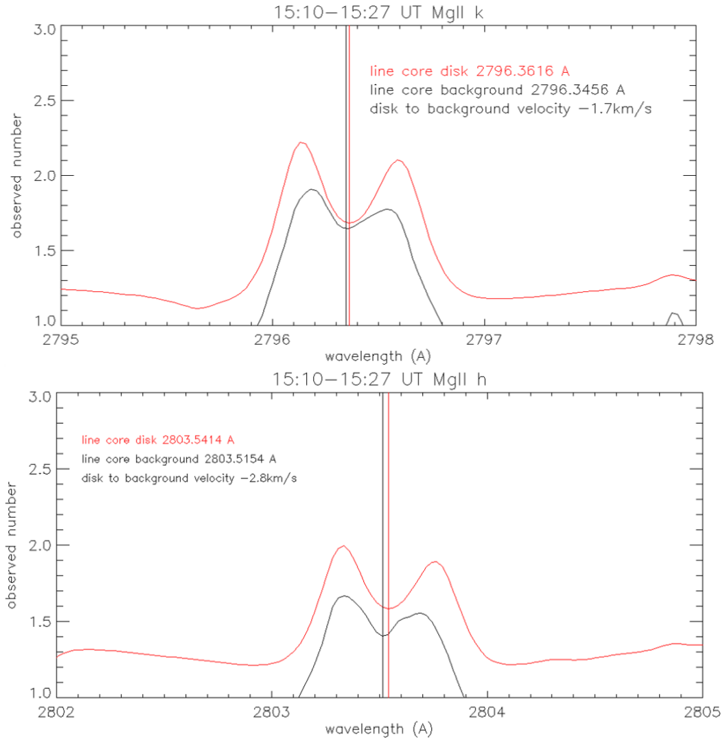
Figure 3.23 Upper and lower panels are the averaged spectra of Mg II k and h lines respectively. The red lines show the profiles averaged over the red box on disk in Figure 3.22. The black lines show the profiles averaged over the white box above limb in Figure 3.22.
