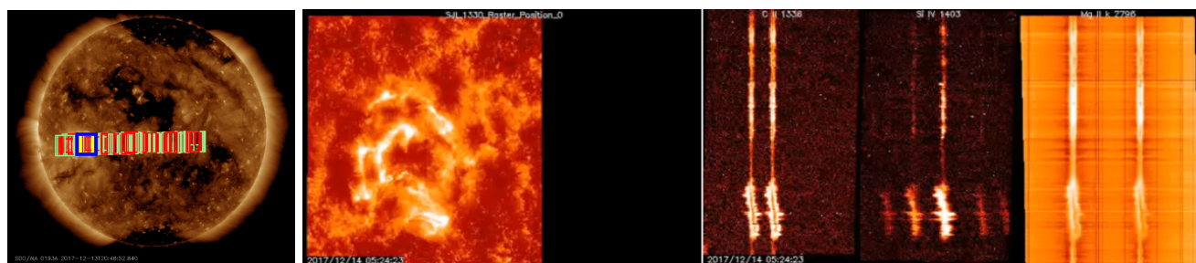
Figure 5.4 Left: An AR tracked as it crosses the disk. The full disk image of the Sun is taken on Dec 13 by AIA in 193 Å. The green boxes correspond to the FOV of the HOP 307 very large dense 320-step raster observations of IRIS, and the red lines show the left and right boundary positions of the slit rasters. Middle: IRIS SJI image whose FOV is marked in blue in the left panel observed at 05:24 UT on Dec 14 in 1330 Å. The slit is crossing the flare region at this time, and the corresponding spectra of C II, Si IV and Mg II lines are shown in the right panel.
