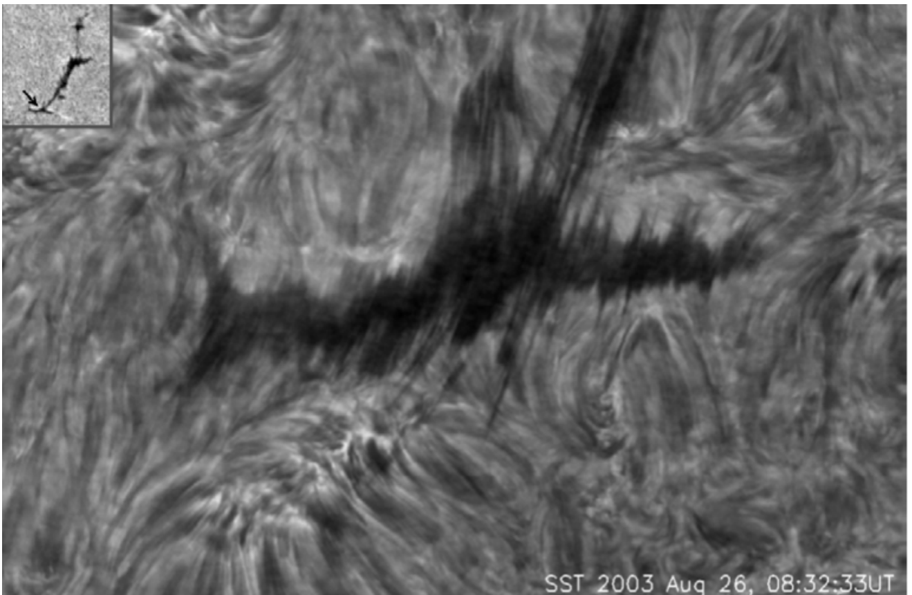
Figure 1.3 High resolution H\alpha image of parts of the southern end of a multi-thread filament observed by the 1-meter Swedish Solar Telescope (SST) on 26 August 2003 (Lin et al., 2008a).
