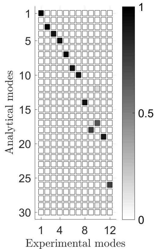
Figure 3.15: MAC matrix.
