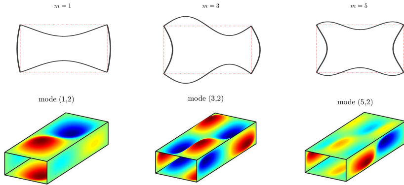
Fig. 3. Section mode shapes \varphi_m ( n = 1 ) and 3D illustration of some global modes of the duct \phi_{mn} .
