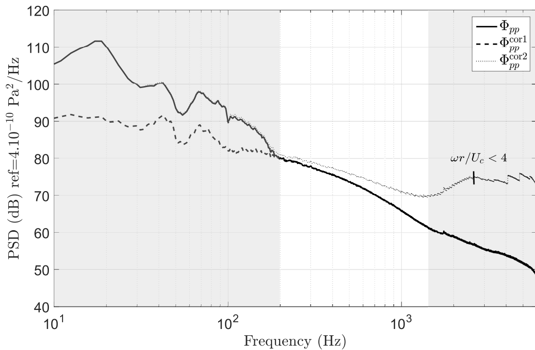
Figure 2.8: Corrected values \Phi_{pp}^{\text{cor1}} (after noise reduction) and \Phi_{pp}^{\text{cor2}} (after taking into account sensor area averaging) at 20 m/s. The grey area indicates the uncertainties about the true low and high frequency spectral components of the point spectrum.
