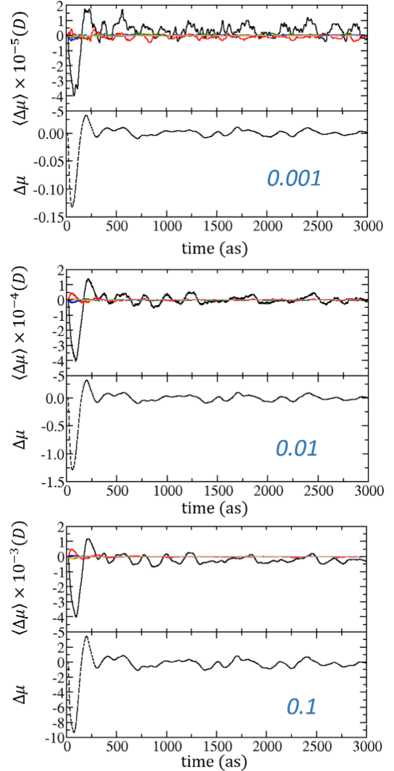
Figure 9. Correlation between the variations of the induced dipole moments on water molecules averaged by hydration shells \langle \Delta\mu(t) \rangle = \langle \mu(t) - \mu(0) \rangle (upper-part of each graph) and the variation of dipole moment of the peptide (Lower-part of each graph). The three main graphs correspond to three perturbing field strengths of 0.001a.u (Top-Lefts), 0.01 (Bottom-Left) and 0.1 a.u. (Top-Right). The colors are defined in the caption of Figure 8.
