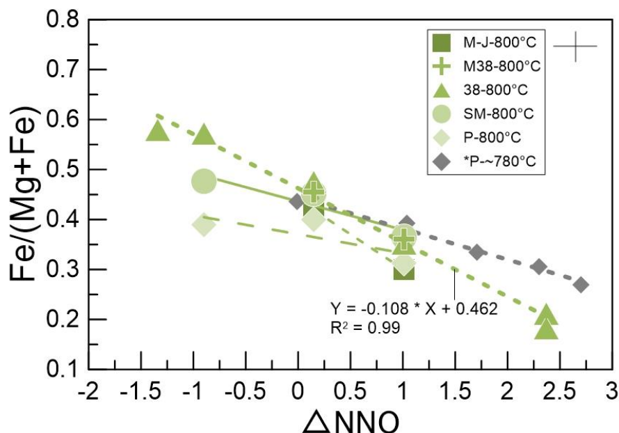
Fig. 6.6 Fe# = Fe_{tot}/(Fe_{tot}+Mg) of experimental amphiboles ( X_{H_2O}=1 ) plotted as a function of oxygen fugacity ( \Delta NNO = \log fO_2^{exp} - \log fO_2^{NNO} ). *P are the data of experimental Amp composition cited from Scaillet and Evans, 1999. Vertical error is the maximum standard deviation of Fe#, and the horizontal bar is the maximum uncertainty of oxygen fugacity ( \Delta NNO ).
