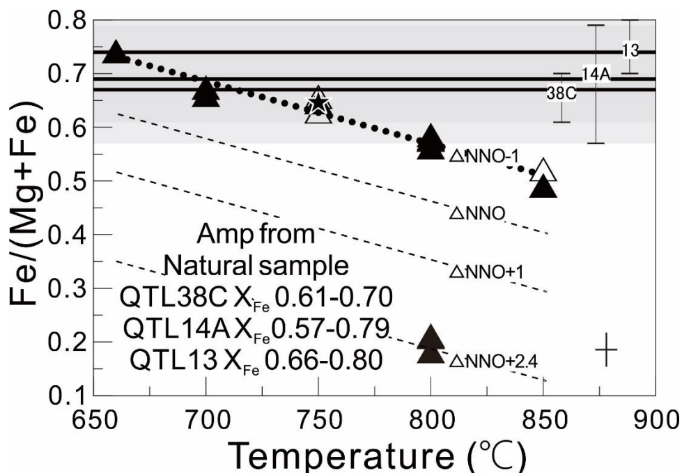
Fig. 5.4 Compositions of experimental amphiboles at water saturation ( \blacktriangle ) and below water saturation ( \triangle ) plotted as a function of temperature with compositions of natural amphibole (shaded area). Triangles represent the experimental amphibole crystallized from composition QTL-38 while the solid star represents those from composition 14A. The grey area are the range of \text{Fe}/(\text{Mg}+\text{Fe}) of natural amphiboles from 3 samples whereas the bold black lines are the average \text{Fe}/(\text{Mg}+\text{Fe}) value. The horizontal bar is the maximum uncertainty of temperature; the vertical bar is the maximum uncertainty of \text{Fe}/(\text{Mg}+\text{Fe}) .
