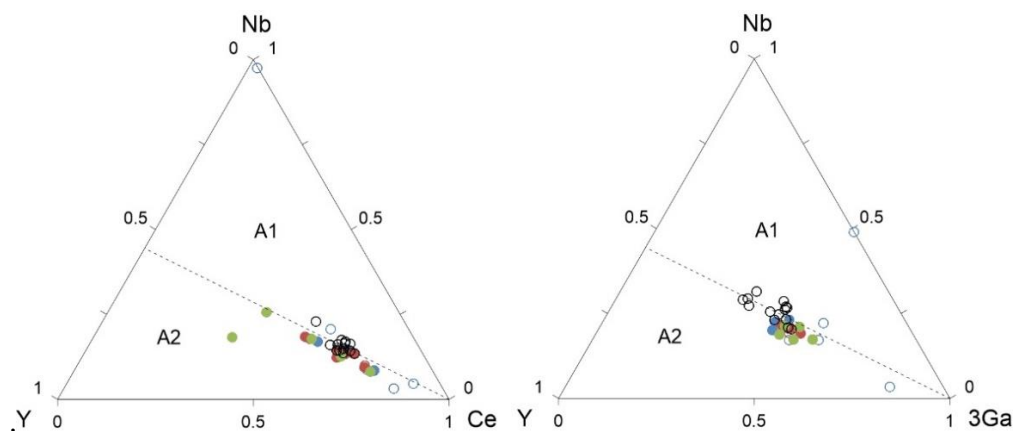
Fig. 4.21 Plot of Qitianling granite and mafic enclave in (a) Ce-Nb-Y and (b) 3 \cdot \text{Ga} -Nb-Y diagrams of Eby (1992) for subdivision of A1-type and A2-type granites.
