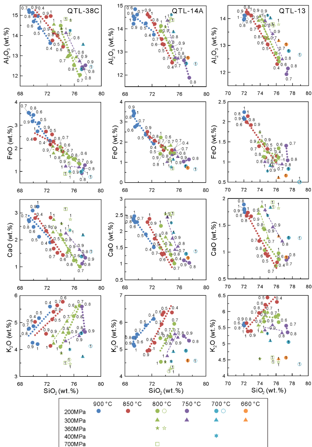
Fig. 5.6 Variation of residual glass compositions (on average) of samples QTL38C, QTL14A, QTL13 at different pressure, temperature, oxygen fugacity and melt H 2 O content conditions. Solid symbols and empty symbols represent those glass from reducing (~NNO-1.3) and oxidizing (~NNO+2.4) charges, respectively. The numbers attached to the symbols are the XH 2 O values from each charge.
