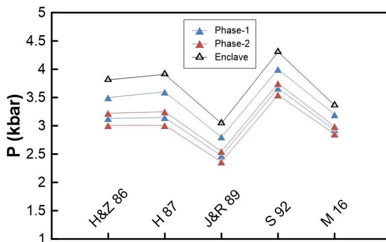
Fig. 4.23 Plot of calculated average pressure results of amphiboles from the Qitianling granites and enclaves by different geobarometers. The amphibole compositional data of enclaves are from Zhao et al., 2012. The information on different barometers is given in Table 4.3.
