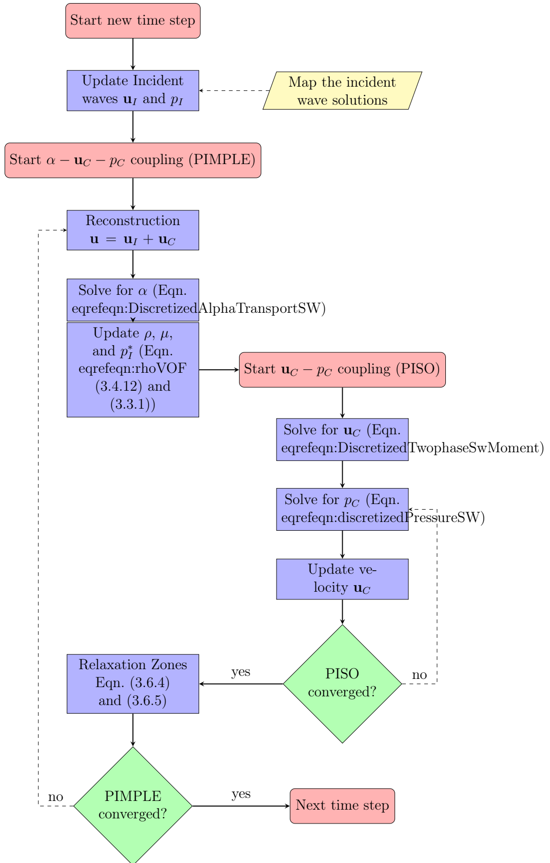
Figure 3.6: Solution Algorithm of the SWENSE method
