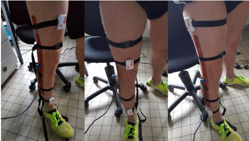
Figure 53. Tested sensor positions (Left: sensor on the thigh directly; Middle: sensor above the kneecap; Right: sensor in the sagittal plane)
