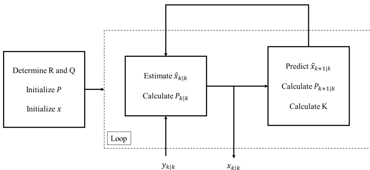
Figure 22. Kalman filter scheme
