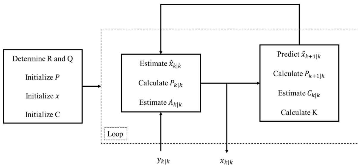
Figure 23. Extended Kalman filter scheme
