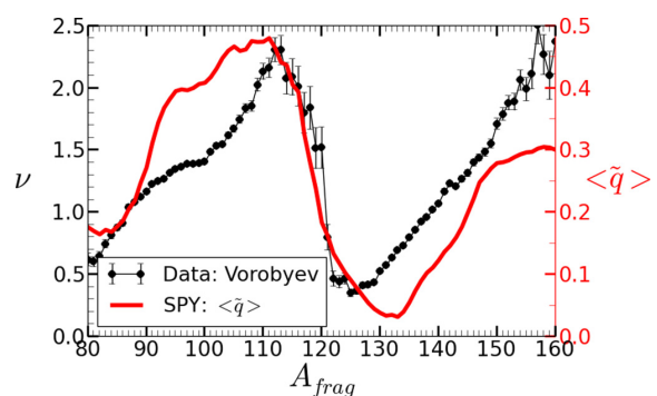
FIG. 10. (Color online) Mean fragment deformation calculated with SPY (red, right scale) in the ^{235}\text{U}(n_{th}, f) reaction, compared to the experimental mean number of evaporated neutrons \nu (black, left scale) from Vorobyev [28].
