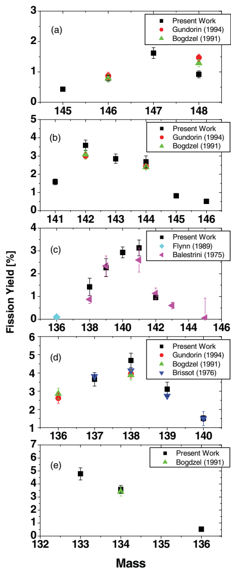
FIG. 7. (Color online) Isotopic yields obtained in this work in the heavy mass region and compared with data from the literature: ^{58}\text{Ce} (a), ^{55}\text{Cs} (b), ^{54}\text{Xe} (c), and ^{52}\text{Te} (e).
