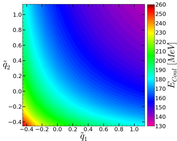
FIG. 3. (Color online) Coulomb energy between two fragments (fragment 1: ^{132}\text{Sn} ; fragment 2: ^{104}\text{Mo} ) as a function of their quadrupole deformation.
