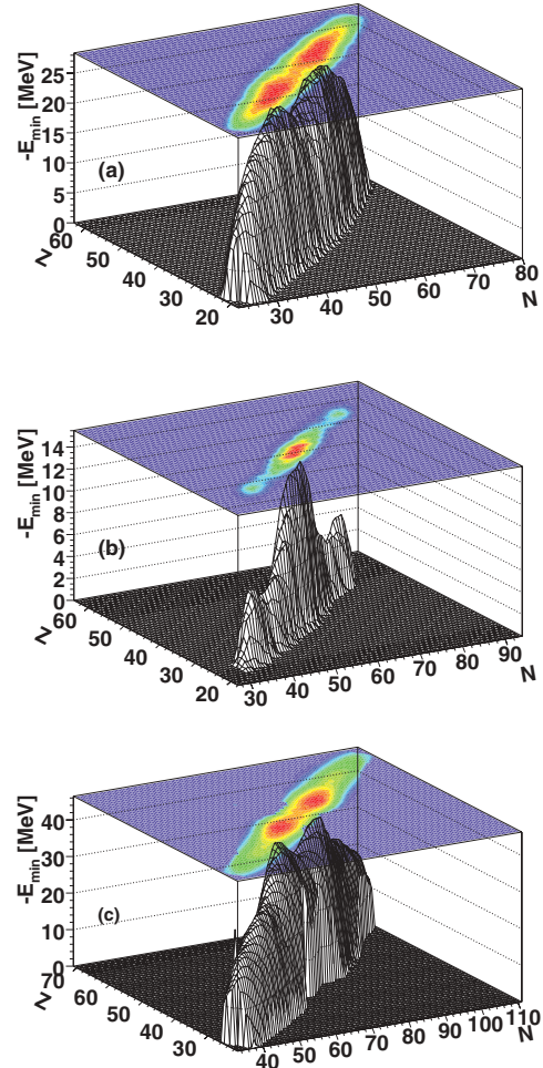
FIG. 2. (Color online) Minimum absolute available energy at scission calculated for all possible fragmentations in (a) ^{180}\text{Hg} and (b) ^{198}\text{Hg} fission at 10 MeV and in (c) the thermal n -induced fission of ^{235}\text{U} .
