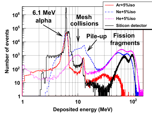
Fig. 10. Reconstructed energy spectrum measured with the FIDIAS-2D prototype irradiated with the ^{252}Cf source in Argon (red line), neon (blue line) and Helium + 5% Isobutene (magenta line). For comparison, the energy spectrum measured with a silicon detector is included (black line) [42]. (For interpretation of the references to color in this figure caption, the reader is referred to the web version of this article.)
