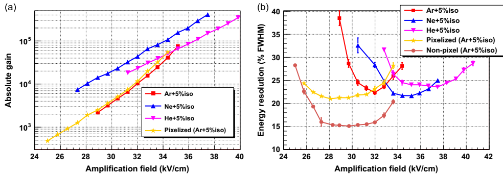
Fig. 7. Absolute gain (left) and energy resolution at 5.9 keV (right) as a function of the amplification field for the FIDIAS-2D prototype in Ar+5% i\text{C}_4\text{H}_{10} (red squares), Ne+5% i\text{C}_4\text{H}_{10} (blue triangles) and He+5% i\text{C}_4\text{H}_{10} (inverted magenta triangles). As a comparison, the measurements obtained with a similar pixelized (orange stars) and non-pixelized (brown points) bulk detectors in Ar+5% i\text{C}_4\text{H}_{10} have been included. (For interpretation of the references to color in this figure caption, the reader is referred to the web version of this article.)
