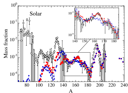
FIG. 4 (color online). Final abundance distribution vs atomic mass for ejecta from 1.35\text{--}1.35 M_\odot NS mergers. The red squares are for the newly derived SPY predictions of the FFDs and the blue circles for essentially symmetric distributions based on the 2013 GEF model [52]. The abundances are compared with the solar ones [56] (dotted circles). The insert zooms on the rare-earth elements.
