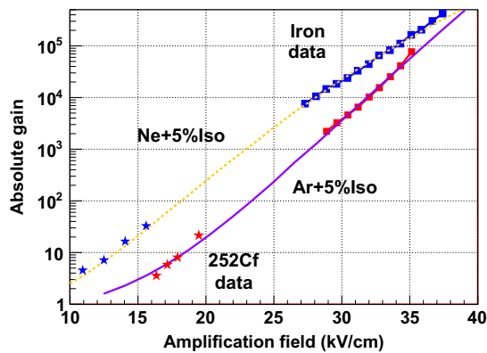
Fig. 8. Absolute gain as a function of the amplification field for the 2D prototype in Ar + 5% iC_4H_{10} and Ne + 5% iC_4H_{10} measured with the iron source (squares) and with 6.1 MeV alphas from Californium (stars). The fitted Rose–Korff model (lines) is also included.
