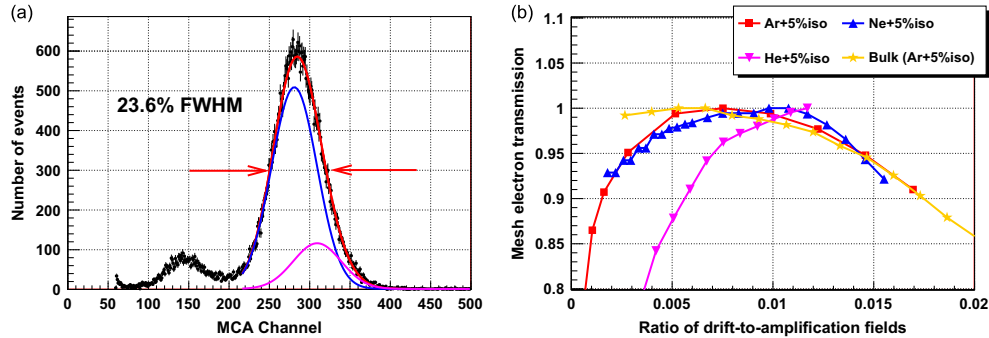
Fig. 6. Left: Example of ^{55}\text{Fe} energy spectrum obtained with the FIDIAS-2D detector in Ar+5% i\text{C}_4\text{H}_{10} . The main peak has been fitted by two Gaussian functions (blue and magenta lines), corresponding to the K_{\alpha} and K_{\beta} lines. The escape peak, generated by X-ray conversion in argon, is situated at around 3 keV. Right: Mesh electron transmission as a function of the drift-to-amplification fields ratio in Ar+5% i\text{C}_4\text{H}_{10} (red squares), Ne+5% i\text{C}_4\text{H}_{10} (blue triangles) and He+5% i\text{C}_4\text{H}_{10} (inverted magenta triangles). As a comparison, the curve by a pixelized bulk detector in Ar+5% i\text{C}_4\text{H}_{10} [7] (orange stars) has been included. (For interpretation of the references to color in this figure caption, the reader is referred to the web version of this article.)
