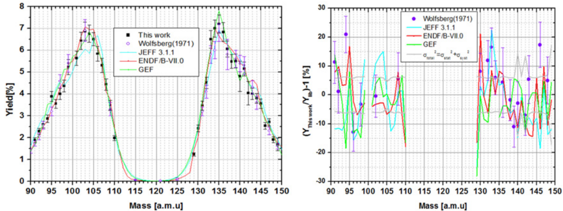
Figure 3. (Left) fission mass yields of ^{242}\text{Am} compared with JEFF-3.1.1 and ENDF/B-VII.0 libraries as well as the experimental data from Wolfsberg [7] and the GEF model. (Right) relative difference between the measured yields and the ones given by JEFF-3.1.1, ENDF/B-VII.0 and Wolfsberg.
