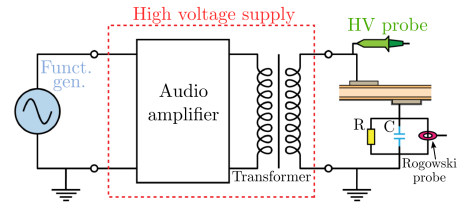
Figure 2.6: Scheme of the electrical set-up (from Jousset [2010])
