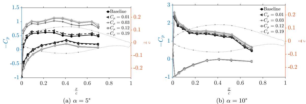
Figure 3.36: Pressure coefficient C_p as a function of the momentum coefficient C_\mu for \alpha = 5^\circ and \alpha = 10^\circ - Re = 130\,000 , T_u = 0.5\% and r = 0.63R
