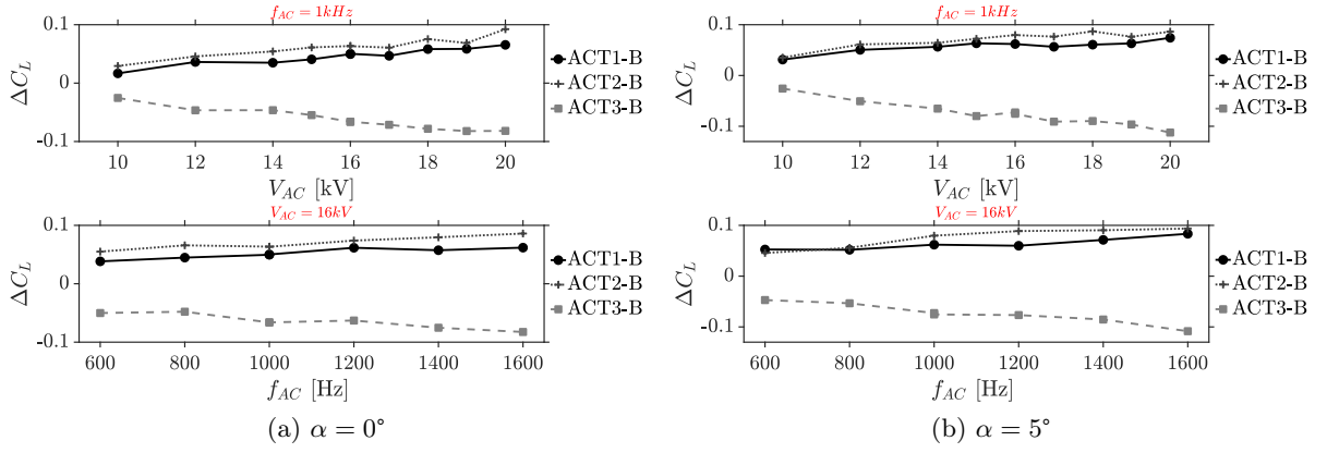
Figure 2.31: Lift coefficient variation \Delta C_L as a function of the applied voltage V_{AC} and frequency f_{AC} for \alpha = 0^\circ and \alpha = 5^\circ - B-series and Re = 200\,000
