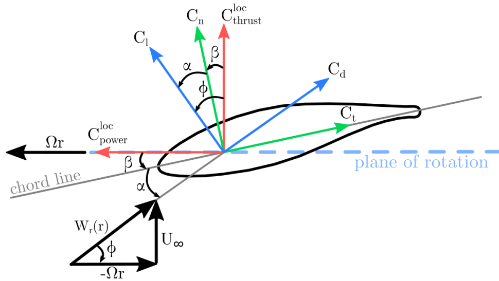
Figure 4.3: Blade airfoil element velocities and forces
