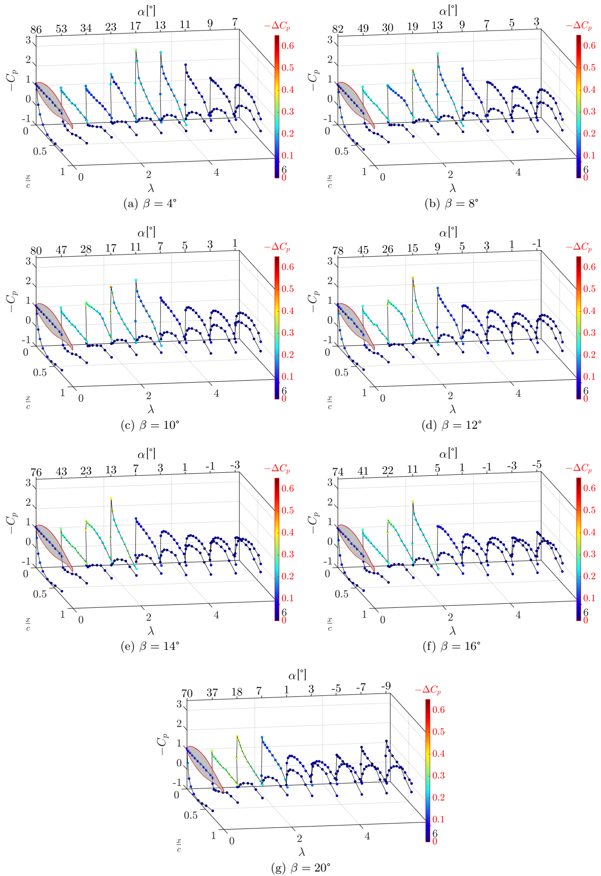
Figure 4.28: C_p distribution along \frac{x}{c} as a function of \lambda for different pitch angles \beta - lines depict the baseline case, dot colors show the \Delta C_p variation for control case P2 - r = 0.88R
