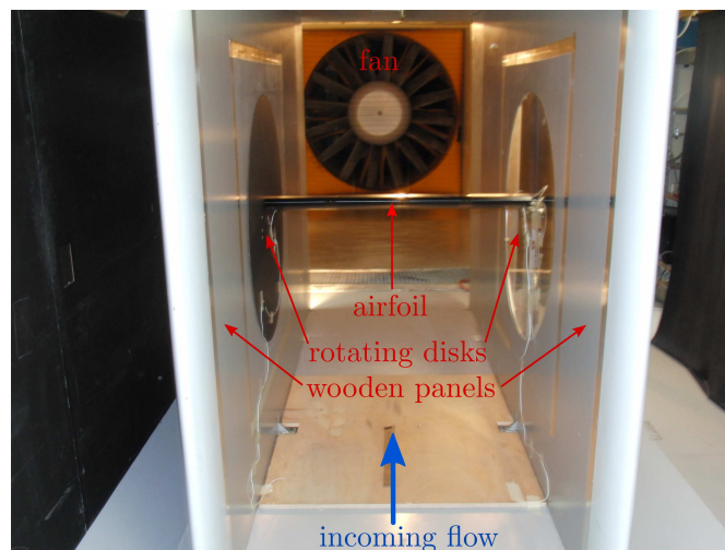
Figure 2.9: Picture of the test-section panels and the 2D-airfoil
