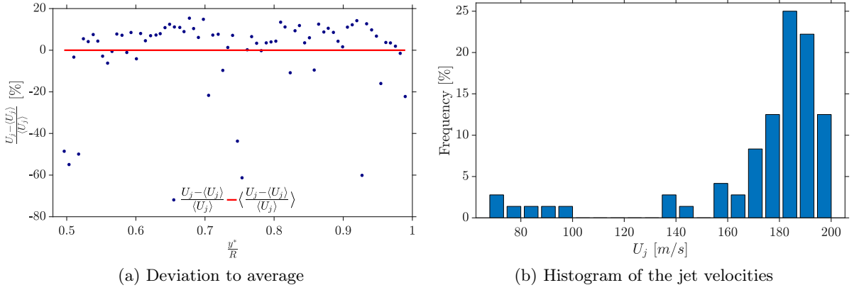
Figure 3.16: Deviation of the jet velocities to the spanwise average and their histogram - C_\mu = 0.022
