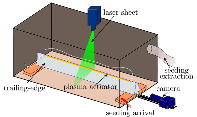
Figure 2.8: Scheme of the PIV set-up used to characterise the plasma actuators in quiescent air conditions
