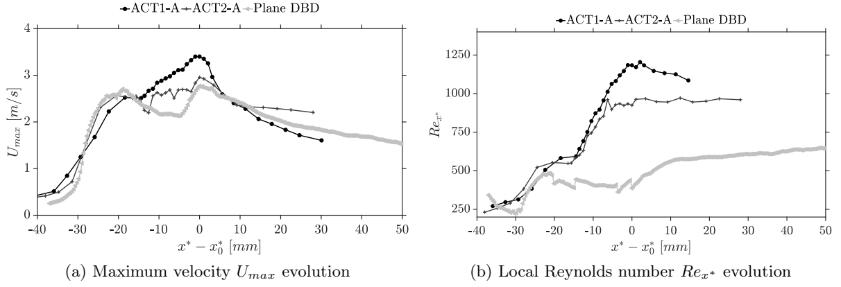
Figure 2.22: Maximum velocity U_{max} and local Reynolds number Re_{x^*} evolution in the flow direction x^*
