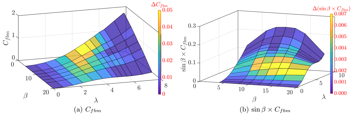
Figure 4.24: Flapwise bending moment coefficient C_{fbm} as a function of the tip-speed ratio \lambda and the pitch angle \beta - surface shape depicts the baseline case, colors show the respective variation for control case P2
