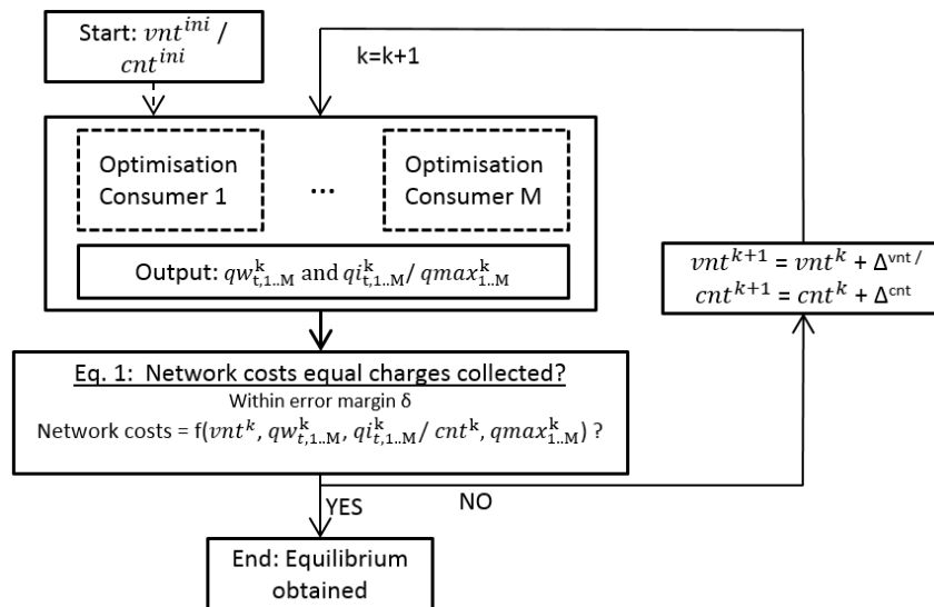
Figure 7: Flow of the calculations to obtain the equilibrium
