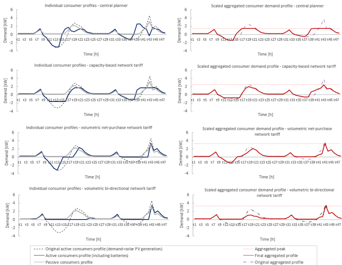
Figure 20: Reactions of active consumers to the different network tariff design and their impact on the aggregated load profile and peak. Assumption: 5 kWp solar PV already installed by the active consumer and battery investment cost of 100 €/kWh.
