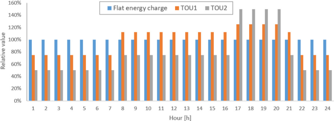
Figure 22: Three energy price schemes.
