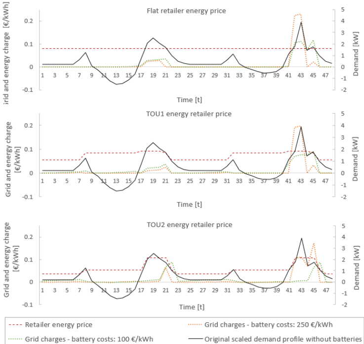
Figure 24: Examples of peak-coincident network prices for the case 5 kWp is installed by the active consumers. Sensitivity for the battery investment costs of 250 and 100 €/kWh.
