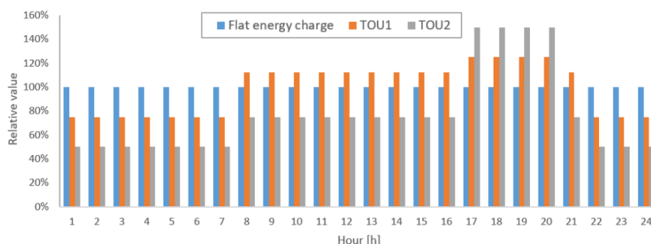
Figure C.3: Three profiles for energy prices
