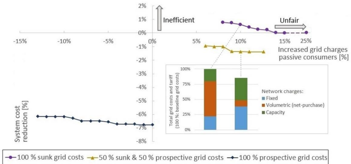
Figure 14: Total system cost increase trade-off with the increase of grid charges of passive consumers for different grid cost structures. Perfect proxy for the grid cost drivers assumed.
