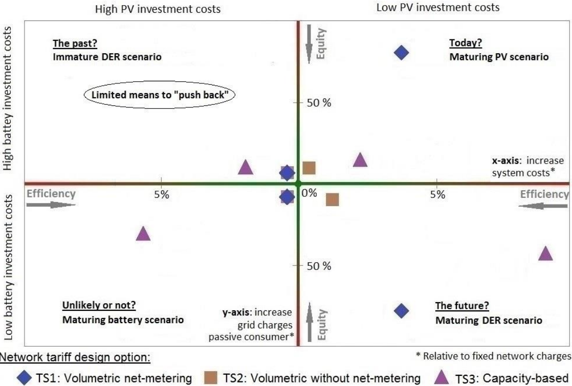
Figure 8: The results for the four scenarios of the technology matrix with 50 % active consumers connected to the grid. Results of the efficiency (horizontal) and equity (vertical) proxy are shown. The more the result of a tariff structure is situated near the origin along one axis, the better its performance for the metric on the other.
