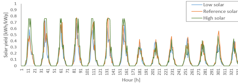
Figure C.2: Three 2-week solar PV yield profiles (including seasonality)
