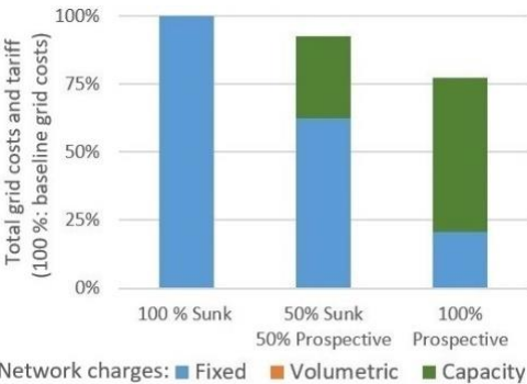
Figure 13: Network tariff components and total grid costs compared to the baseline for the three grid cost structures. Imperfect proxy for the network cost driver assumed (WF=0.75).
