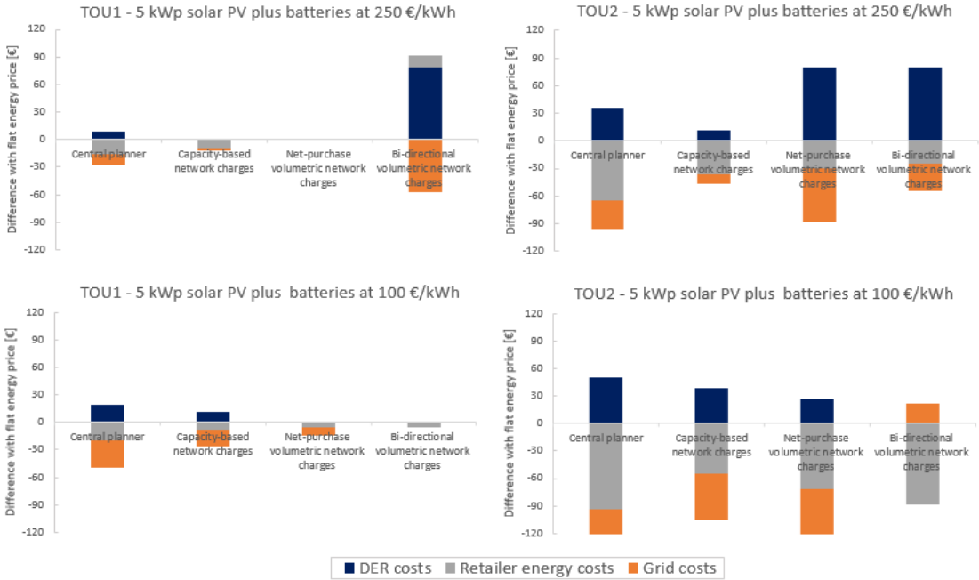
Figure 23: Absolute difference in the different system costs components when comparing a flat energy price with the two time-of-use energy price schemes under different battery investment cost scenarios.
