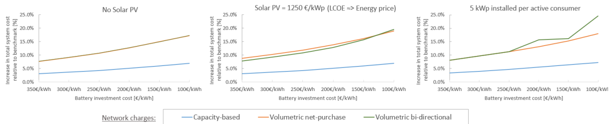
Figure 19: Increase in total system costs for the three network tariff structures when compared with a central planner. Sensitivity for three different assumptions regarding solar PV adoption and the investment cost of storage.
