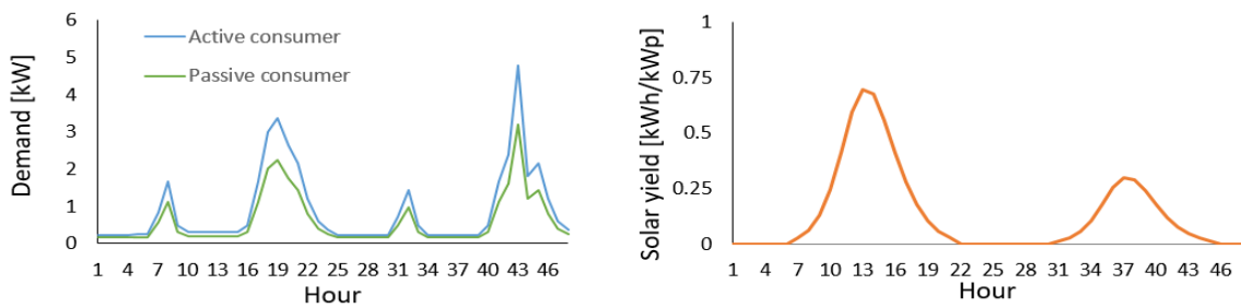
Figure 17: Original 48-hour electricity demand profiles (left) and PV yield profile (right)
