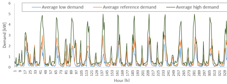
Figure C.1: Three 2-week (average) consumer profiles
