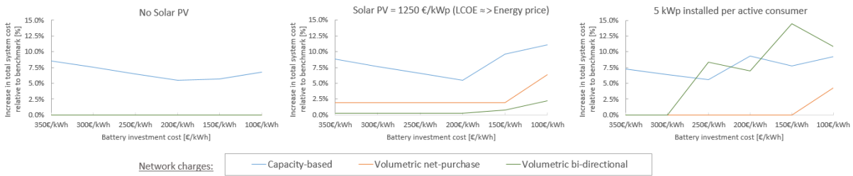
Figure 18: Increase in total system costs for the three network tariff structures when compared with the benchmark. Sensitivity for three different assumptions regarding solar PV adoption and the investment cost of storage.
