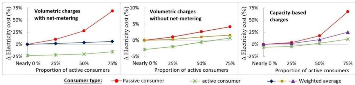
Figure 10: Difference in annual electricity cost per consumer type for the three network tariff structures compared to the application of non-distortive fixed network tariffs. Additionally, the weighted average electricity cost (or system cost) which serves as the proxy for efficiency is shown.
