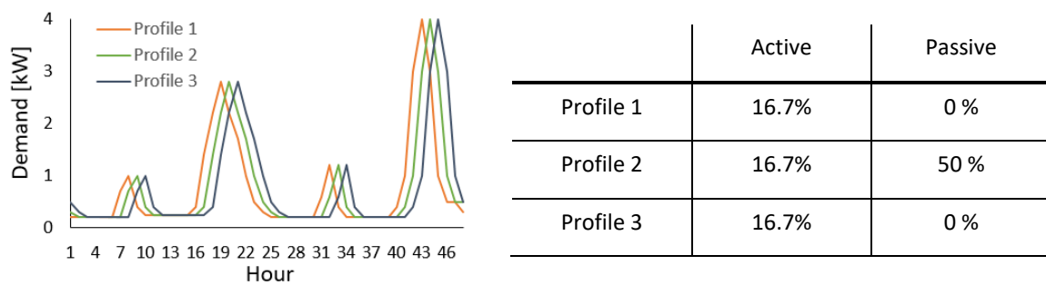
Figure D.1: Profiles and proportions consumers per profile and active/passive
