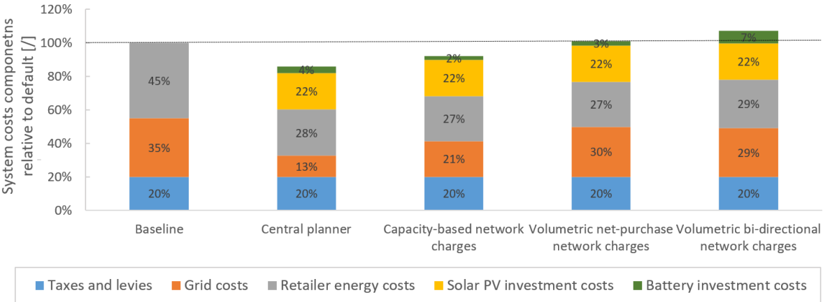
Figure 21: System costs and its components for the different network tariff designs. Assumption: 5 kWp solar PV already installed by the active consumer and battery investment cost of 100 €/kWh.
