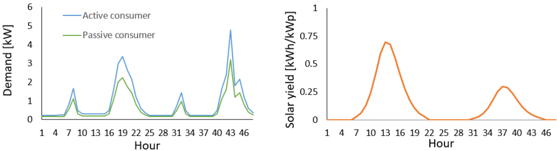
Figure 11: Original 48-hour electricity demand profiles (left) and PV yield profile (right)
