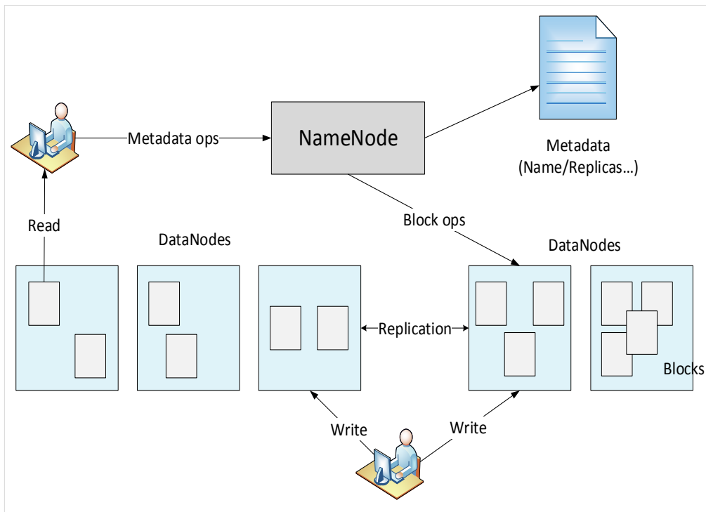
Figure 2.2 HDFS Architecture.
