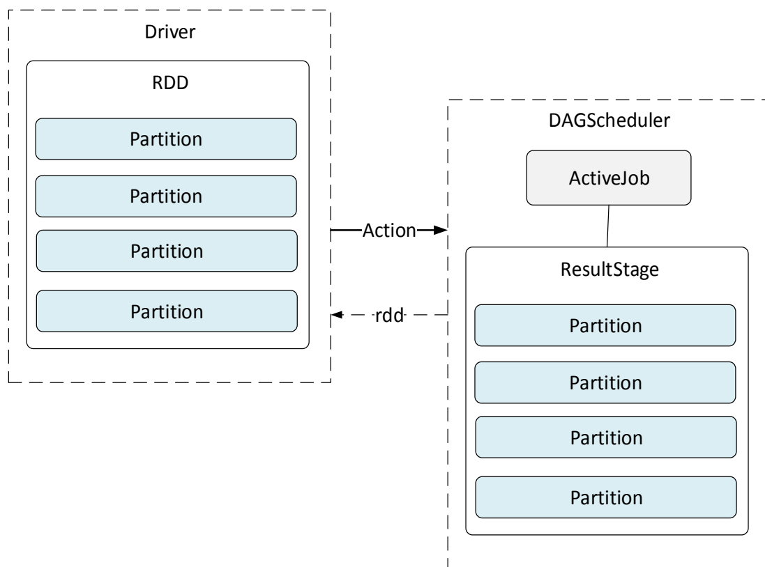
Figure 2.7 DAGScheduler
