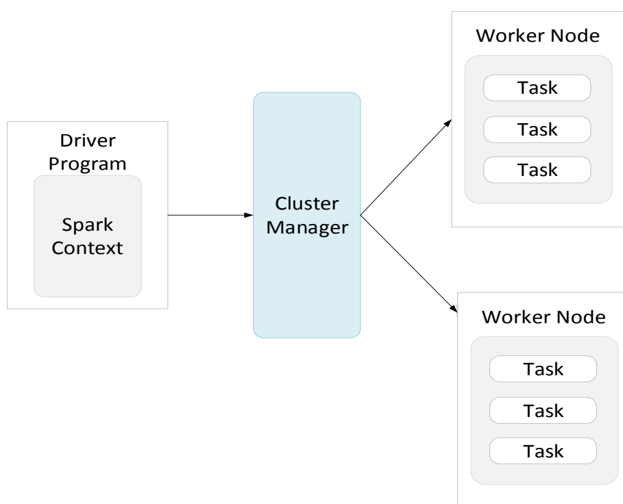
Figure 2.5 Spark Architecture.
