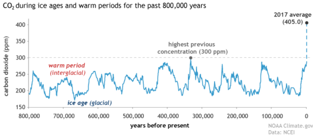
Figure 1.2 Concentration of CO 2 in the atmosphere.
