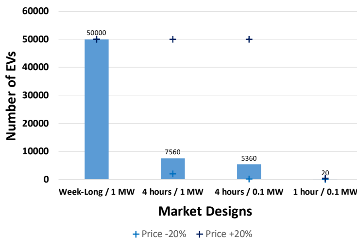
Figure 3.27 Minimum Size of Fleet for Fleet 2a
