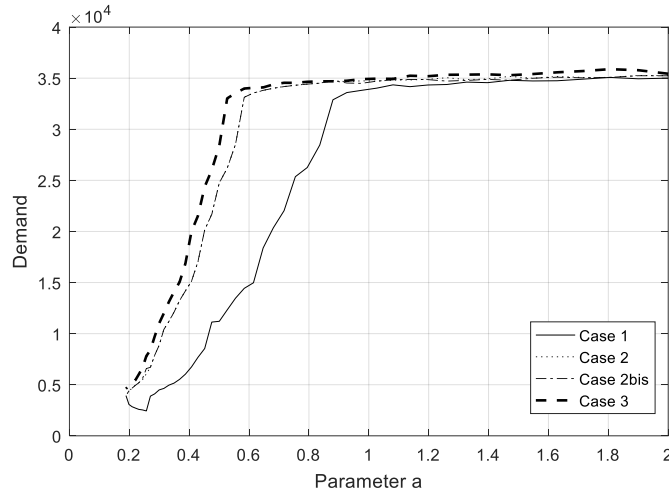
Figure 4.28 Demand for V2G function in Case-Study 3
