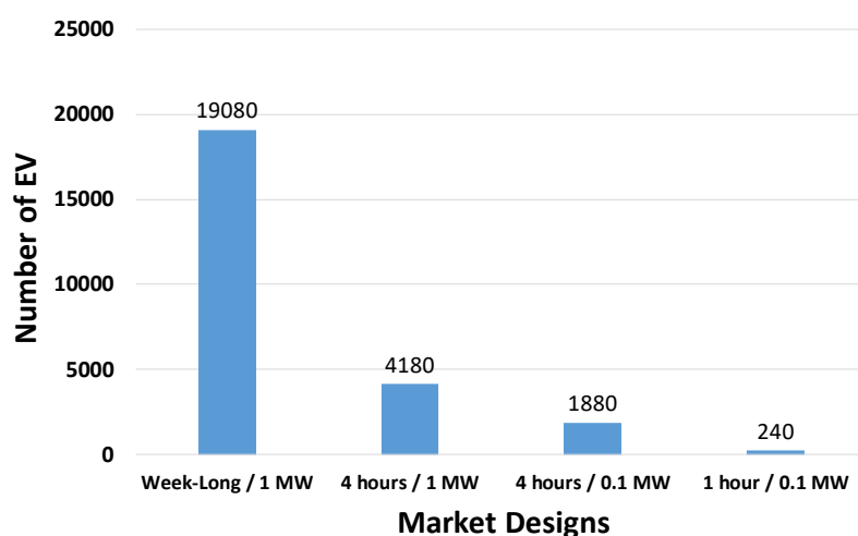
Figure 3.22 Minimum Size of the Fleet for Base-Case Scenario
