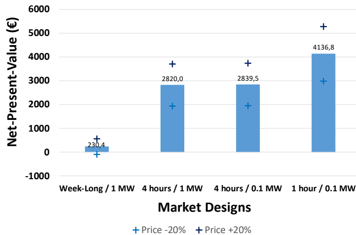
Figure 3.28 Maximum NPV per EV for Fleet 2b
