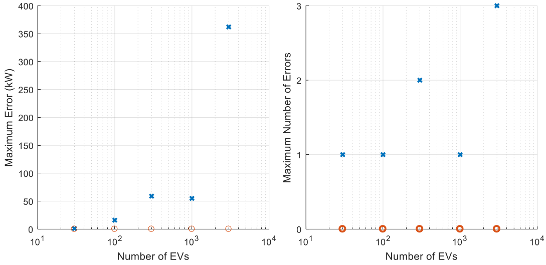
Figure 3.10 Validation test without forecast error and \beta = 0
