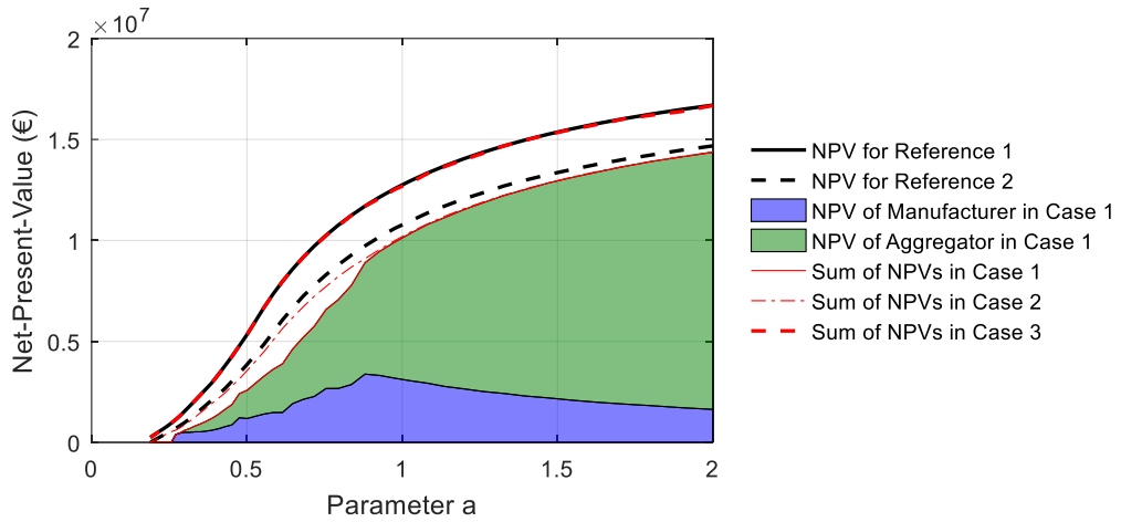
Figure 4.25 Sum of NPVs in Case Study 3
