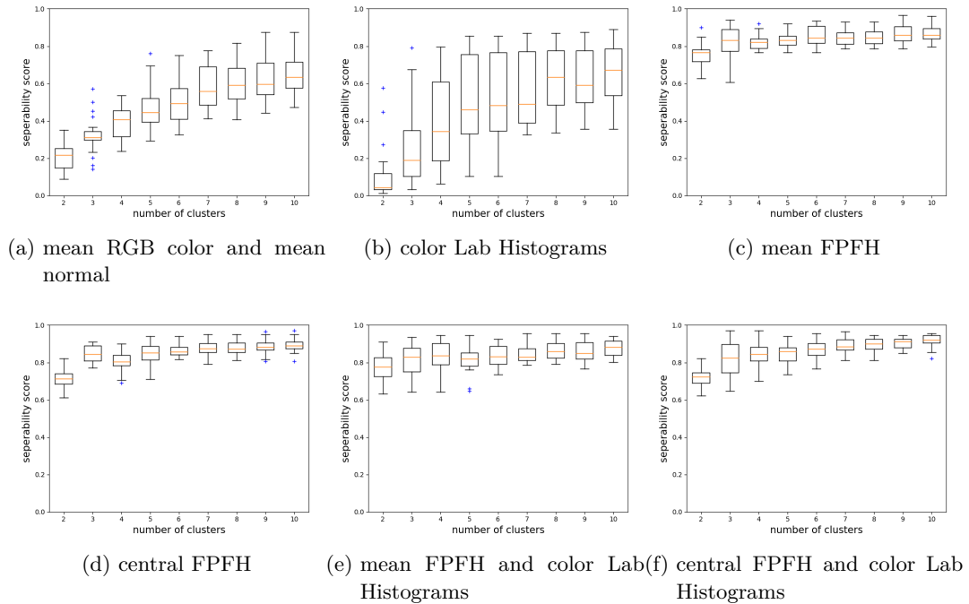
Figure 6.9: Box plots of separability scores on dataset collected in experiment conducted on the second workbench setup 6.1b
