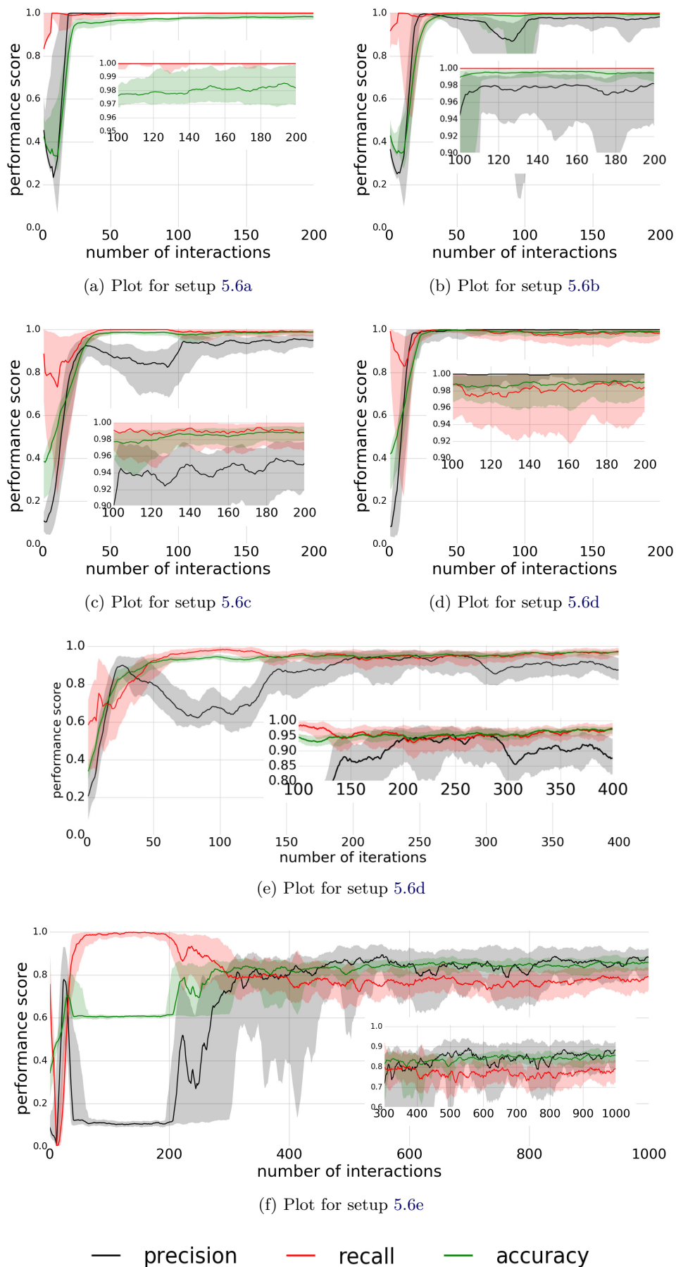
Figure 5.8: Plots of precision, recall, and accuracy for each setup presented in figure 5.6
