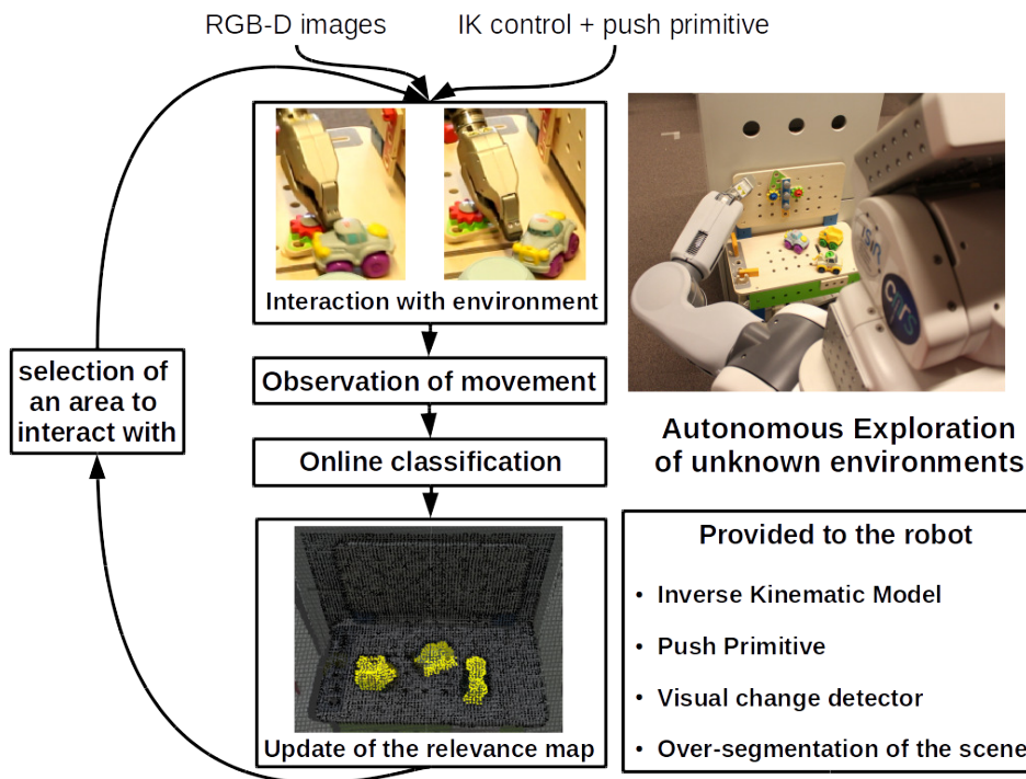
Figure 5.1: Schema presenting the general approach presented in this chapter
