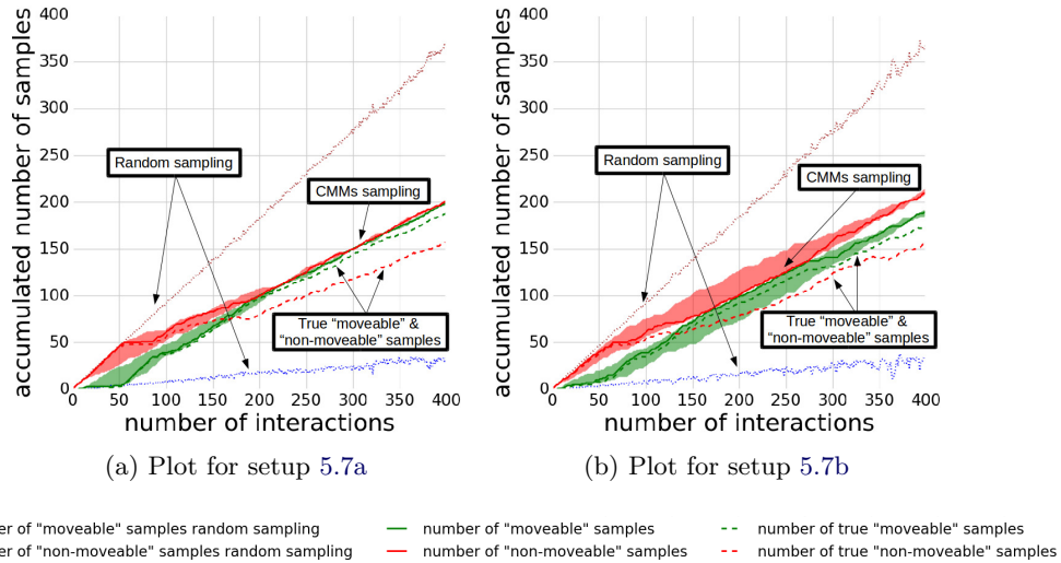
Figure 5.14: Plots of the number of samples gathered for each class at each iteration during the experiments for each setup presented in figures 5.7.
