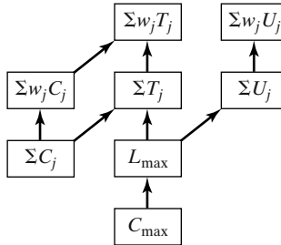
Figure 1.5: Complexity Hierarchies (Pinedo, 2012)
