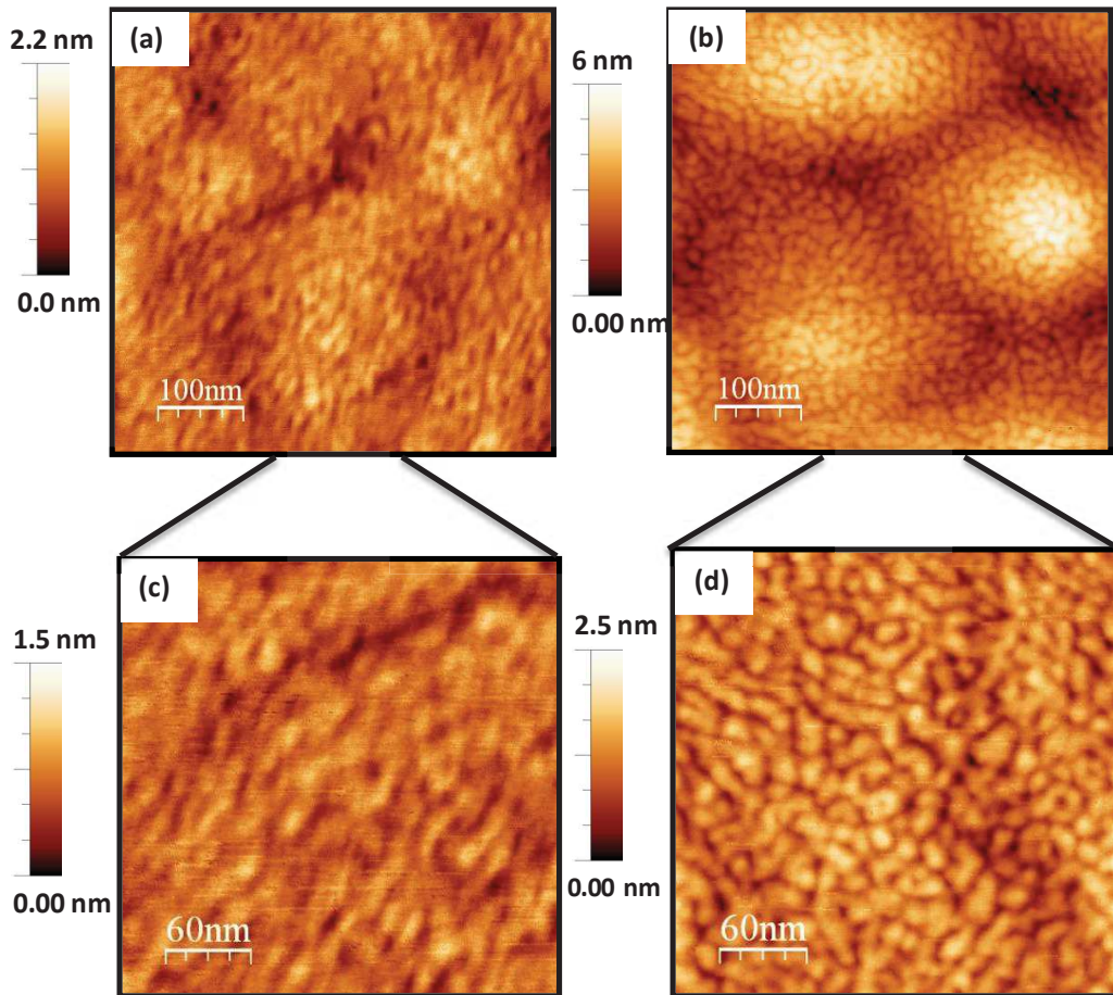
Figure III-2. AFM images of Al_{0.1}Ga_{0.9}N nanostructures with a deposited thickness of a) 7.5 MLs and b) 10.5 MLs. c) and d) are zooms of images a) and b) respectively.
