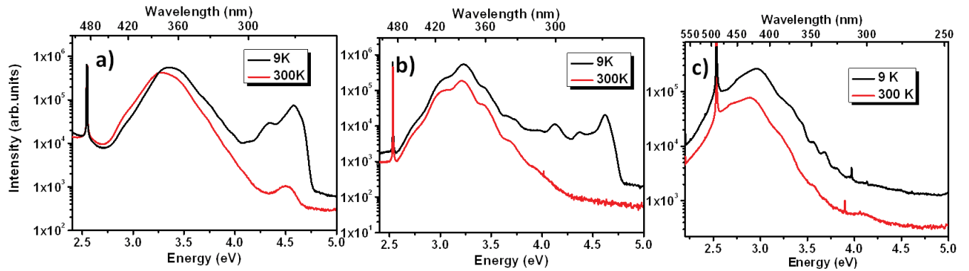
Figure II-14. Low and room temperatures PL spectra of: a) GaN QDs / Al_{0.5}Ga_{0.5}N (sample D), b) GaN QDs / Al_{0.6}Ga_{0.4}N (sample E), and c) GaN QDs / Al_{0.7}Ga_{0.3}N (sample F), grown using ammonia source.
