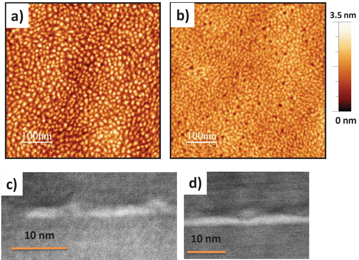
Figure IV-5. AFM and cross sectional TEM images of Al_{0.1}Ga_{0.9}N QDs (a and c, respectively), and Al_{0.2}Ga_{0.8}N QDs (b and d, respectively).
