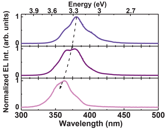
Figure V-3. Room temperature electroluminescence spectra for GaN / Al_{0.5}Ga_{0.5}N QD-based LEDs (for an injection current density of \sim 30 A / cm^2 ) for different QD active regions (with a deposited amount between 6 and 8 MLs): going from higher QD height (top spectrum) to smaller QD height (bottom spectrum)
