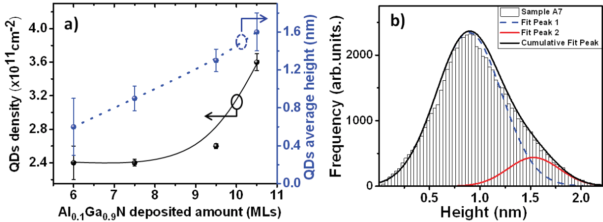
Figure III-3. a) Nanostructures average height and density variation as a function of the deposited amount. b) Height distribution of Al_{0.1}Ga_{0.9}N nanostructures determined by AFM (sample A7), and fitting with two Gaussian functions.
