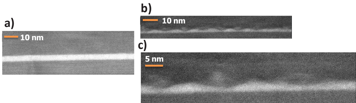
Figure III-16. Cross – section high angle annular dark-field imaging in scanning transmission electron microscopy mode (HAADF-STEM) of Al_{0.1}Ga_{0.9}N QDs with a) an annealing at low temperature ( 740^{\circ}C ), and b) an annealing at high temperature (above 800^{\circ}C ). c) High magnification of image b).
