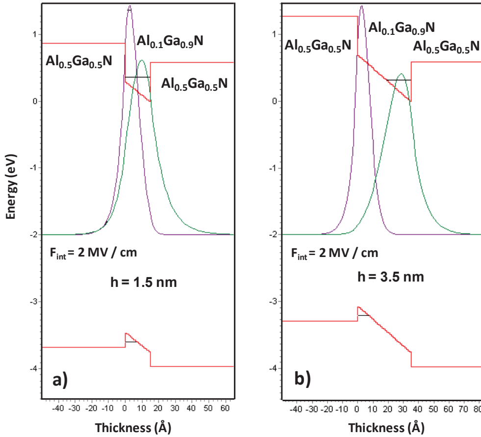
Figure IV-4. Band structures with the electron and hole wave functions and the first energy levels in Al_{0.1}Ga_{0.9}N QW / Al_{0.5}Ga_{0.5}N (0001) system with F_{int} = 2 MV / cm and QW height equal to a) 1.5 nm and b) 3.5 nm.
