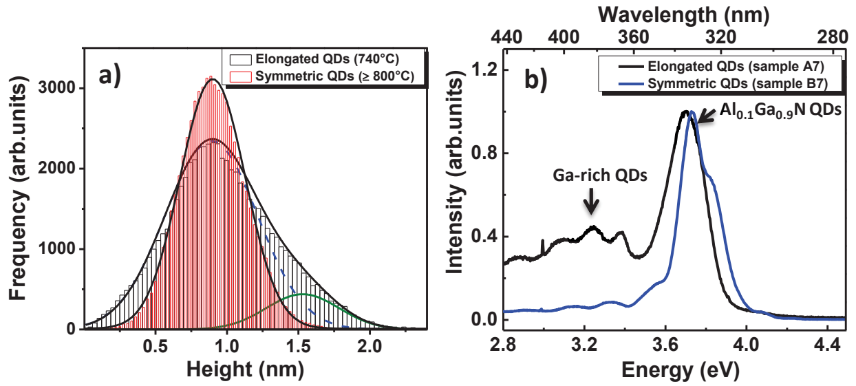
Figure III-17. a) Height distribution of Al_{0.1}Ga_{0.9}N QDs determined by AFM for symmetric QDs (annealed above 800^{\circ}C (HA-plane) and presented by red and white bars) and elongated QDs (annealed at 740^{\circ}C (LT-plane) and presented by black and white bars). Elongated QDs were fitted using two Gaussians curves and symmetric QDs were fitted using one Gaussian curve. b) PL spectrum for symmetric and elongated QDs samples at 300 K.
