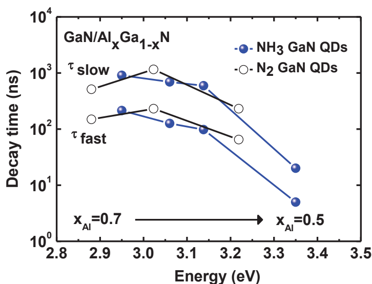
Figure II-20. Fast and slow decay times at low temperature as a function of the GaN QD emission energy. A blue (UV) shift is induced for lower x_{Al} in the Al_xGa_{1-x}N matrix.
