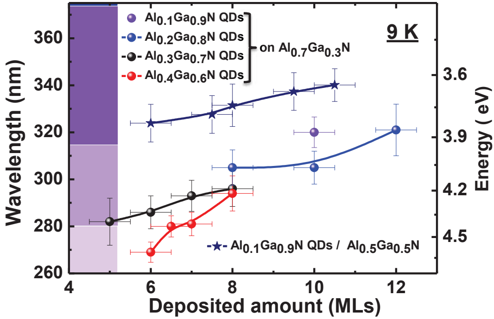
Figure IV-10. Variation of the emission wavelength (i.e. energy) as a function of the QD deposited amount and composition. All the samples presented here were grown on Al_{0.7}Ga_{0.3}N (0001) templates except Al_{0.1}Ga_{0.9}N QDs which were grown on both Al_{0.5}Ga_{0.5}N and Al_{0.7}Ga_{0.3}N (0001) templates.
