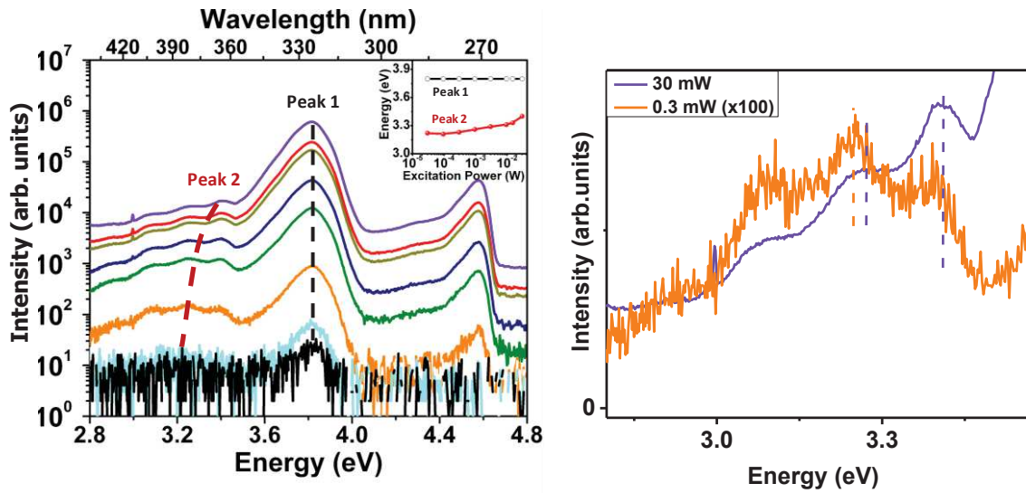
Figure III-11. Low temperature power dependent PL spectra, for Al_{0.1}Ga_{0.9}N (n.c.) QDs with 7.5 MLs (sample A7): a) between 30 mW and 9.5 \mu W , and b) by zooming on the additional low energy band emission for excitation powers of 30 mW and 0.3 mW. The inset in Figure III-11(a) shows the variation of the PL energy as function of the incident power.
