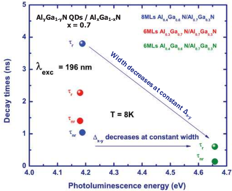
Figure IV-16. Radiative and non radiative decay times at 8 K of different Al_yGa_{1-y}N QD active regions as a function of the emission energy.
