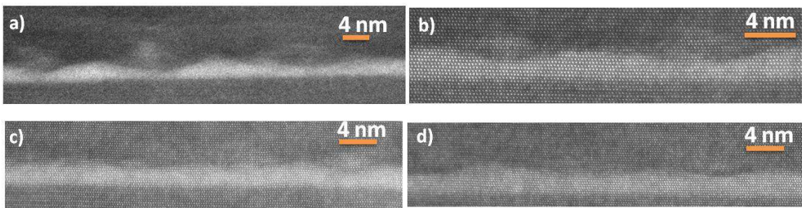
Figure IV-9. HAADF-STEM images for a) Al_{0.1}Ga_{0.9}N QDs (layer 1), b) Al_{0.2}Ga_{0.8}N QDs (layer 2), c) Al_{0.3}Ga_{0.7}N QDs (layer 3) and d) Al_{0.4}Ga_{0.6}N QDs (layer 4), grown on Al_{0.7}Ga_{0.3}N (0001).
