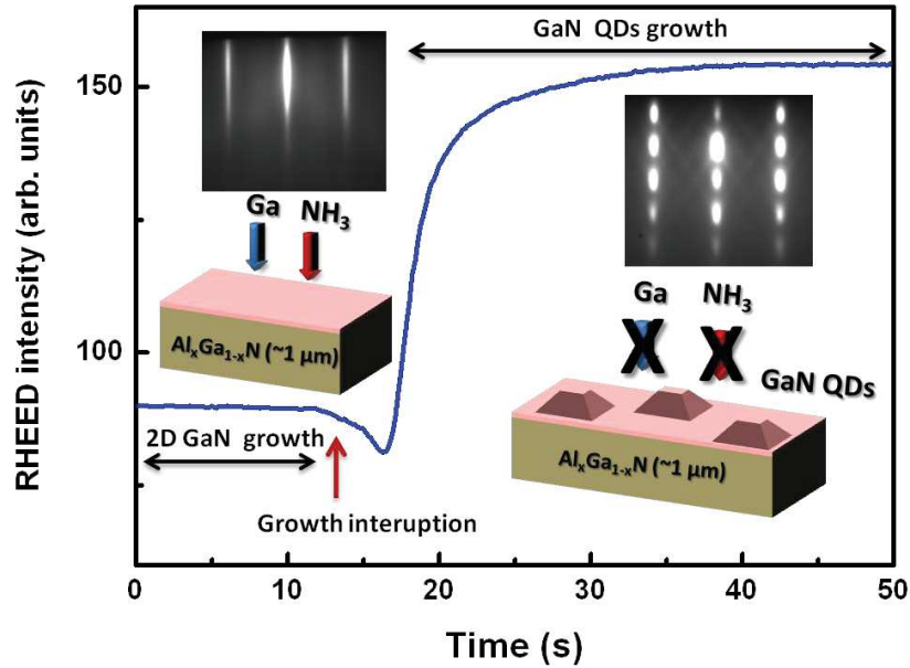
Figure II-9. Variation of the RHEED intensity during the growth of GaN QDs by \text{NH}_3 -MBE. The inset shows a schematics of the 2D-3D morphology of GaN and RHEED images for 2D and 3D GaN surface morphologies.
