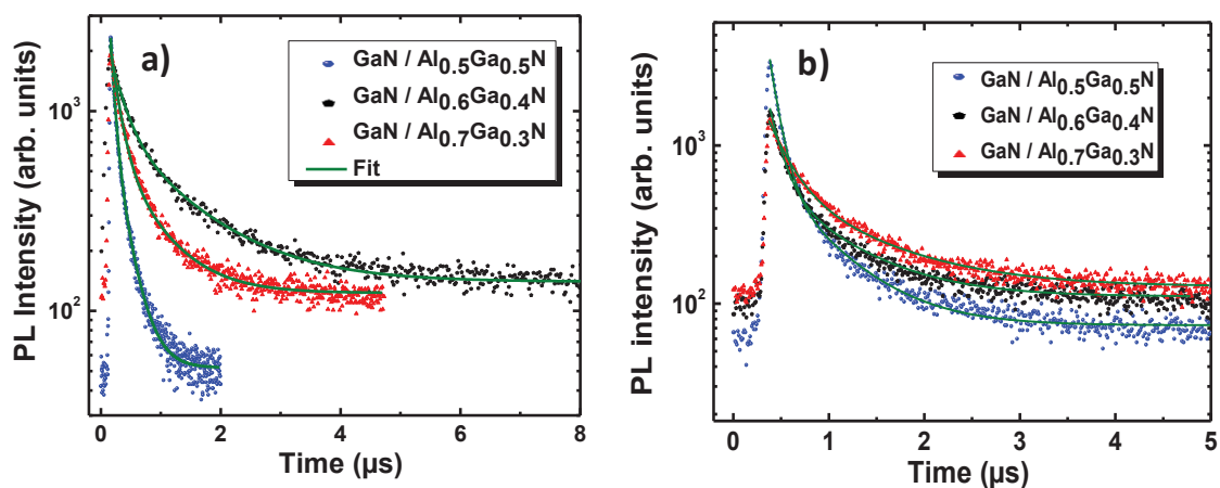
Figure II-19. Time resolved photoluminescence spectra at low temperature (18 K) for GaN QD / \text{Al}_x\text{Ga}_{1-x}\text{N} (0001) structures grown by a) PAMBE and b) \text{NH}_3 -MBE with x_{Al} = 0.5, 0.6 and 0.7 .
