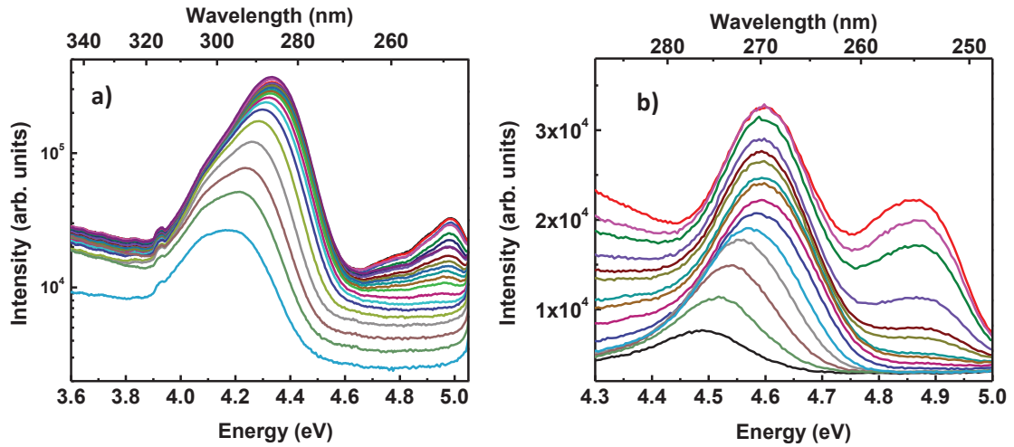
Figure IV-11. Temperature dependent PL spectrums between 9 K and 300 K for a) Al_{0.3}Ga_{0.7}N QDs and b) Al_{0.4}Ga_{0.6}N QDs grown in an Al_{0.7}Ga_{0.3}N (0001) matrix. The PL emission at high energy ( \sim 4.9 eV) is originating from the Al_{0.7}Ga_{0.3}N barrier.
