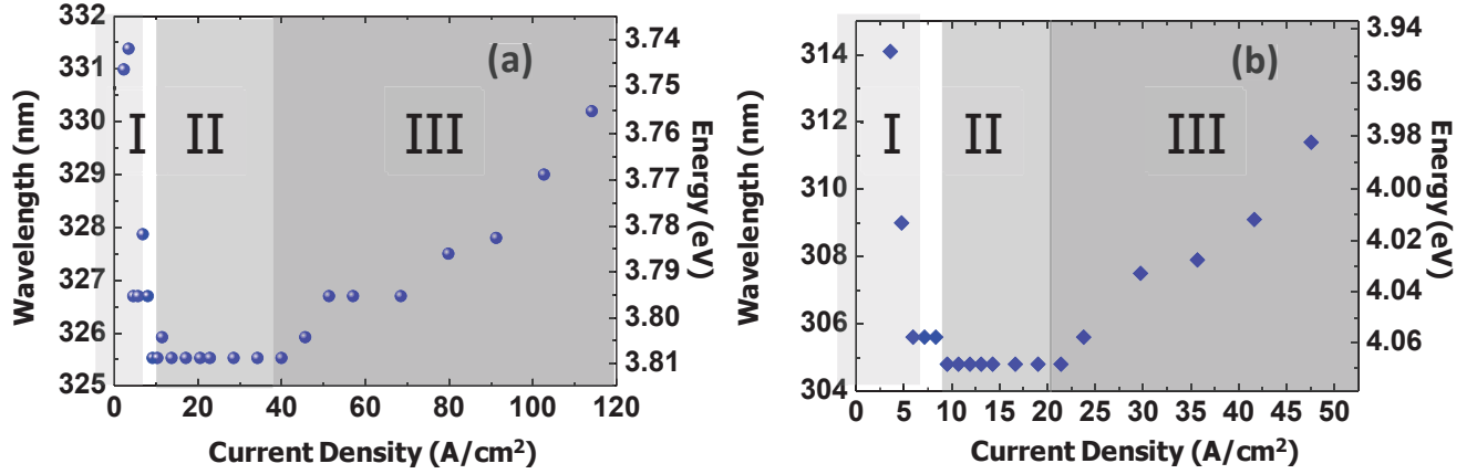
Figure V-9. Variation of the electroluminescence energy of Al_yGa_{1-y}N / Al_{0.6}Ga_{0.4}N (0001) QD-based LEDs as a function of the injected current density for a) Al_{0.1}Ga_{0.9}N (A1) and b) Al_{0.2}Ga_{0.8}N (B1) QD active regions.
