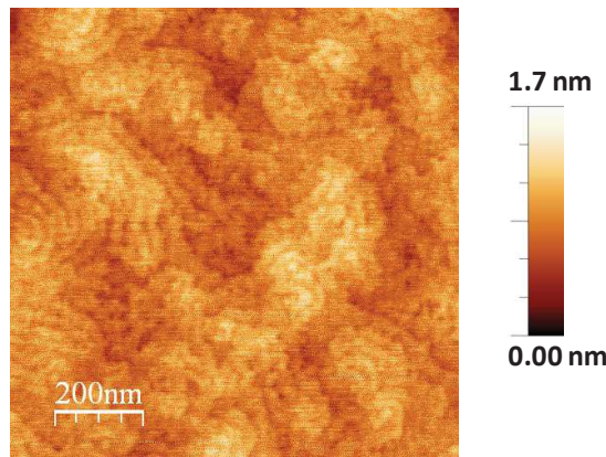
Figure II-11. AFM image of an Al_{0.7}Ga_{0.3}N (0001) template grown using an ammonia source.
