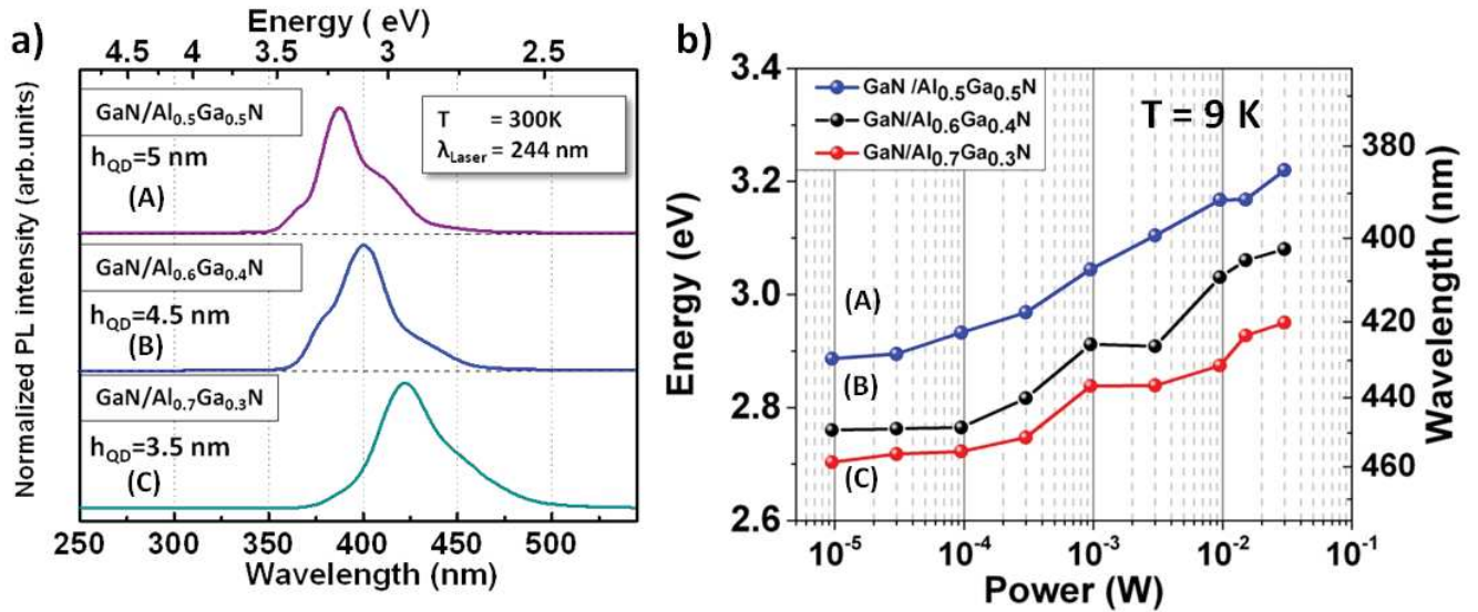
Figure II-7. a) PL spectra at room temperature and b) power dependence PL energy, at 9 K, for GaN / Al x Ga 1-x N (0001) QDs with x_{Al} equals to 0.5 (sample A), 0.6 (sample B) and 0.7 (sample C).
