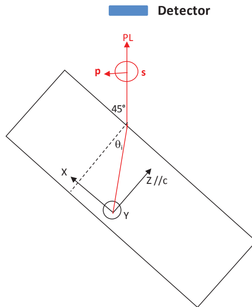
Figure 2. Schematic presenting the photoluminescence with a setup under oblique observation ( \theta \approx 45^\circ ). The X, Y, Z axes are those of the crystal with Z//c (i.e. the growth direction). The luminescence is composed of a wave s (with E perpendicular to the incidence plane), and a wave p (with E parallel to the incidence plane). The transitions involving the X and Z parts of the wave functions will be observed in p geometry and in s geometry for part Y .
