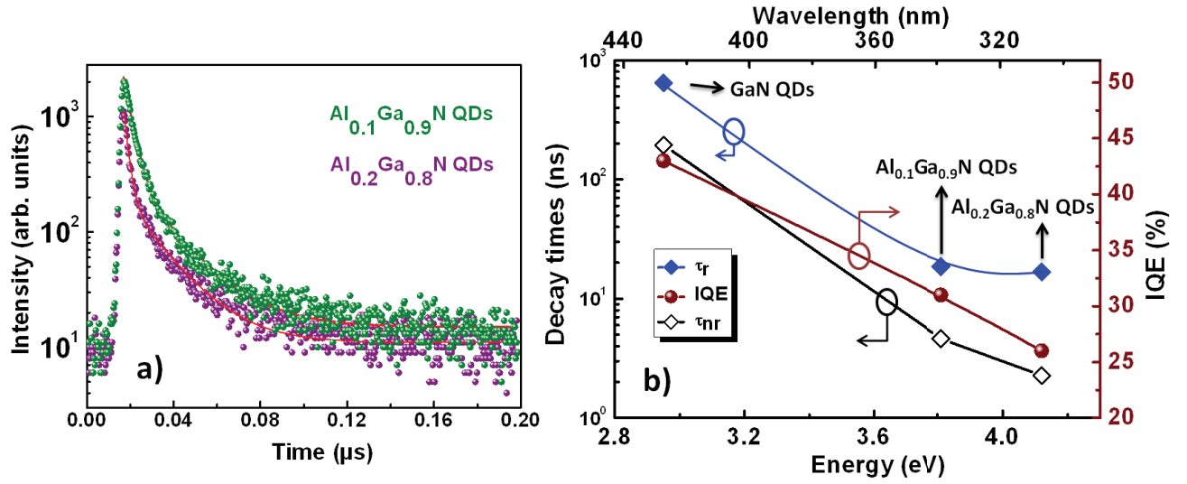
Figure IV-15: TRPL spectra at low temperature for Al_{0.1}Ga_{0.9}N and Al_{0.2}Ga_{0.8}N QDs grown on Al_{0.7}Ga_{0.3}N (0001) template. b) Internal quantum efficiency (IQE) (deduced using eq. IV-3), radiative (equal to \tau_{slow} ) and non radiative (deduced using eq. IV-2) decay times for Al_yGa_{1-y}N ( 0 \leq y \leq 0.2 ) QDs.
