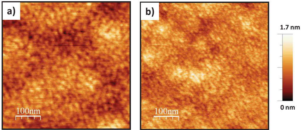
Figure IV-8. AFM images of (0001) a) Al_{0.3}Ga_{0.7}N QDs and b) Al_{0.4}Ga_{0.6}N QDs.
