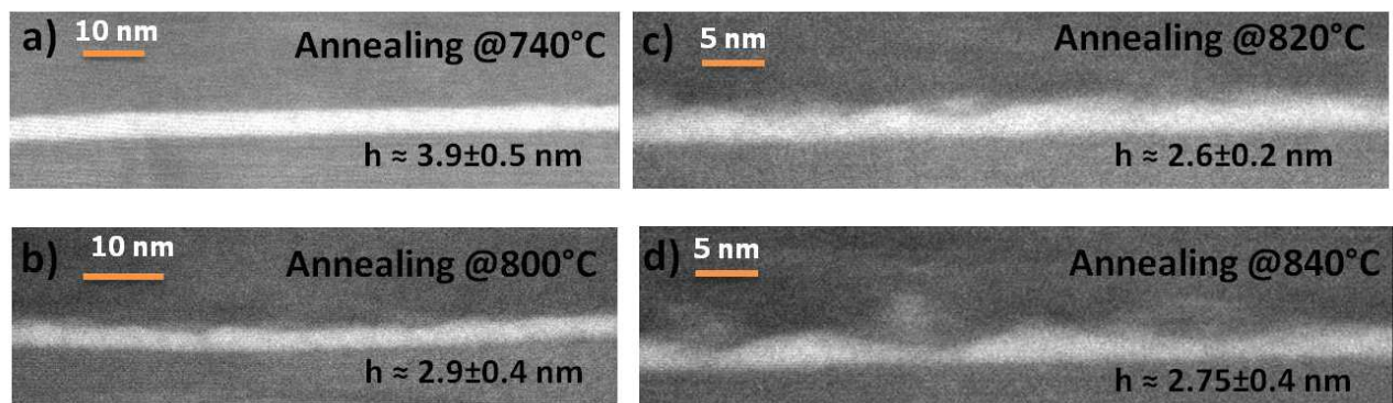
Figure III-21. Cross –section HAADF-STEM images of Al_{0.1}Ga_{0.9}N QDs with an annealing at a) 740°C, b) 800°C, c) 820°C, and d) 840°C.
