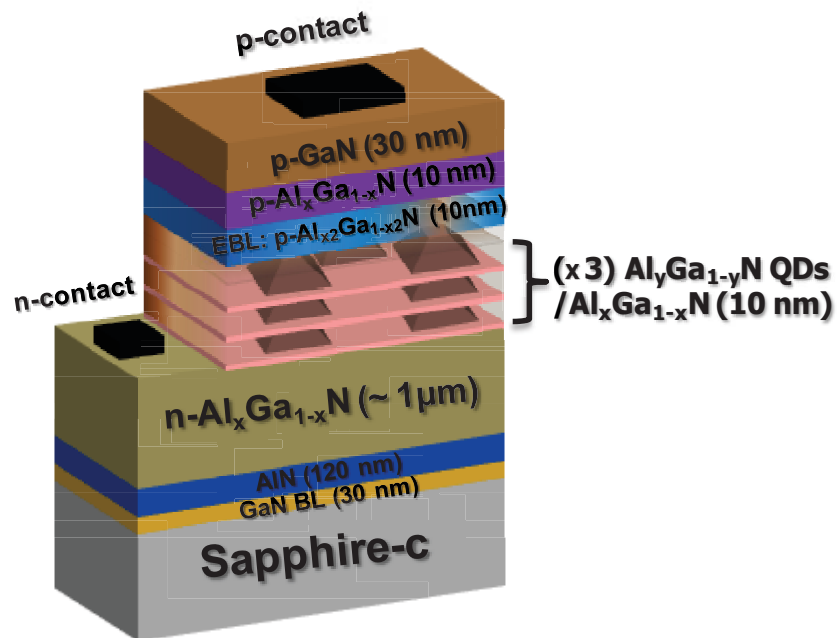
Figure V-2. Schematics presenting the main structure of an (Al,Ga)N QD-based UV LED.
