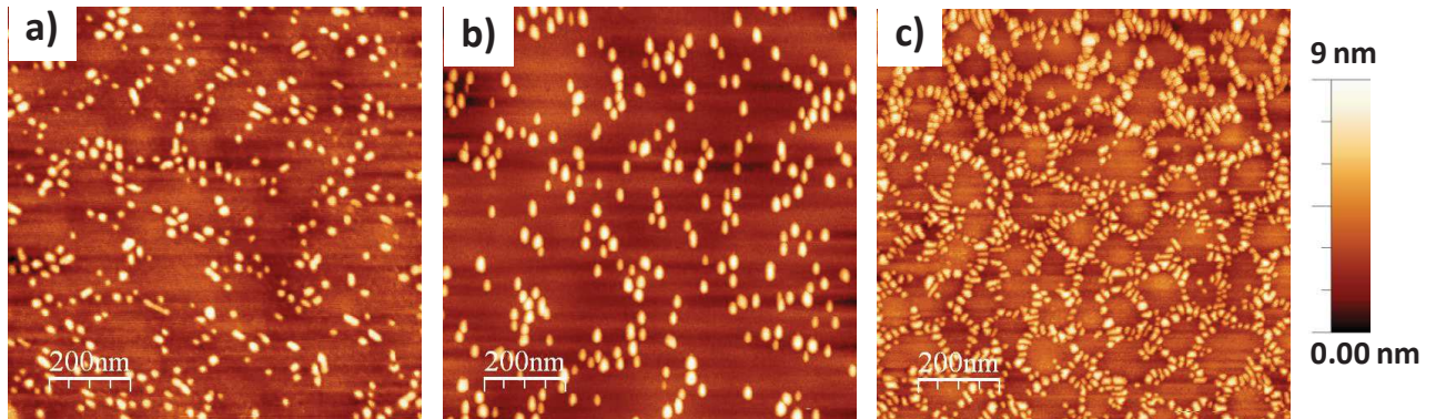
Figure II-10. AFM images of GaN QDs grown using an ammonia source on Al_xGa_{1-x}N (0001) with x equals to a) 0.5 (sample D), b) 0.6 (sample E) and c) 0.7 (sample F).
