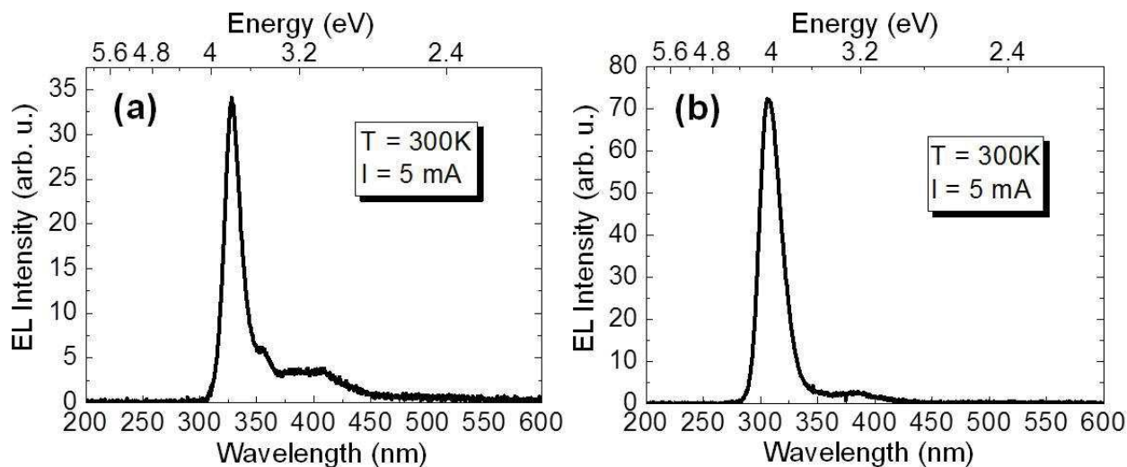
Figure V-7. Electroluminescence spectra over a broad spectral range for a) Al_{0.1}Ga_{0.9}N / Al_{0.6}Ga_{0.4}N (A1) and b) Al_{0.2}Ga_{0.8}N / Al_{0.6}Ga_{0.4}N (B1) active regions of QD-based LEDs. An injection current of 5 mA (i.e. 5.7 A / cm^2 ) was used.
