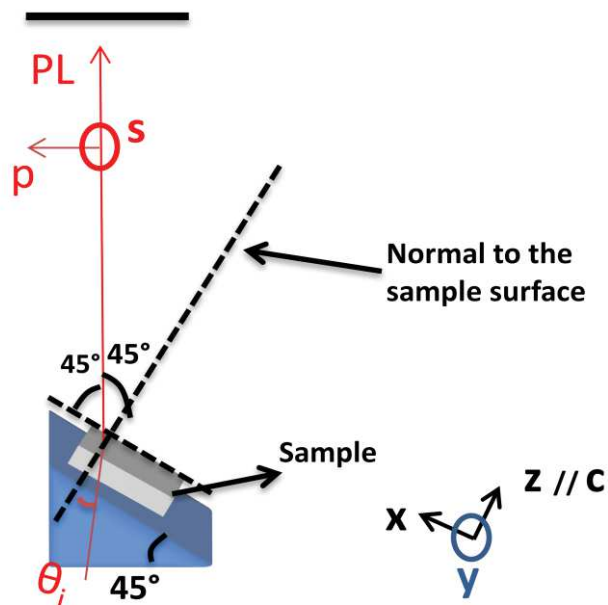
Figure 3. Different schematic representation of the photoluminescence setup under oblique observation ( \theta \approx 45^\circ ).
