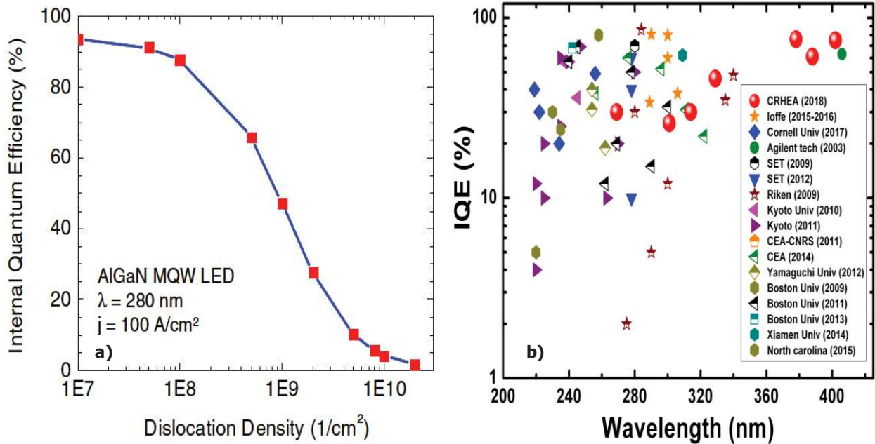
Figure I-11. a) Simulated IQE as a function of the dislocation density for a UV LED emitting at 280 nm [46]. b) State of the art of IQE values for UV sources. The IQE values are estimated from temperature dependent PL measurements to fairly compare the results from the different groups.
