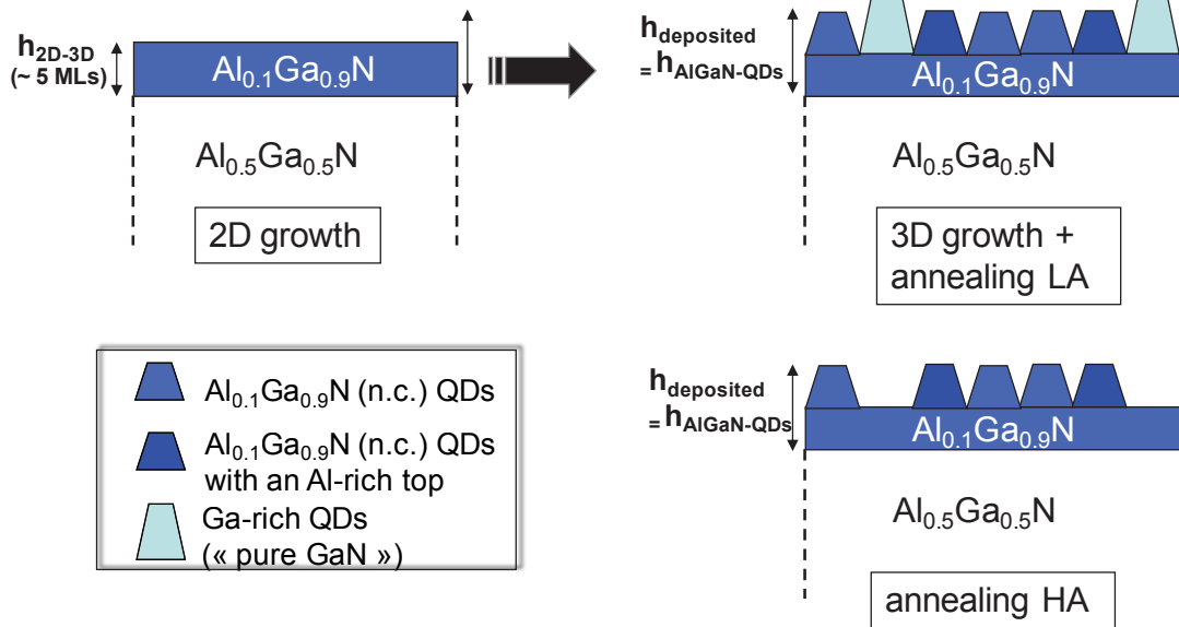
Figure III-18. Schematics presenting the different steps of Al_{0.1}Ga_{0.9}N QDs (10 MLs) growth with the different annealing processes: a) initial growth of an Al_{0.1}Ga_{0.9}N 2D layer (before the 2D-3D transition); b) QDs formed at low annealing (LA) temperature ( \approx 740^{\circ}C ); c) QDs formed at high annealing (HA) temperatures ( \geq 800^{\circ}C ).
