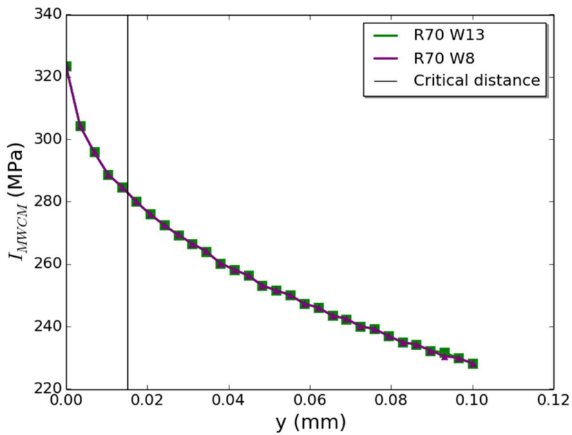
Figure 5-9: Evolution of the multiaxial fatigue index under the contact at x/a = -1 for both specimen widths (\sigma_{B,max}/p_0 = 0,36; Q/fP = 0,43) .
