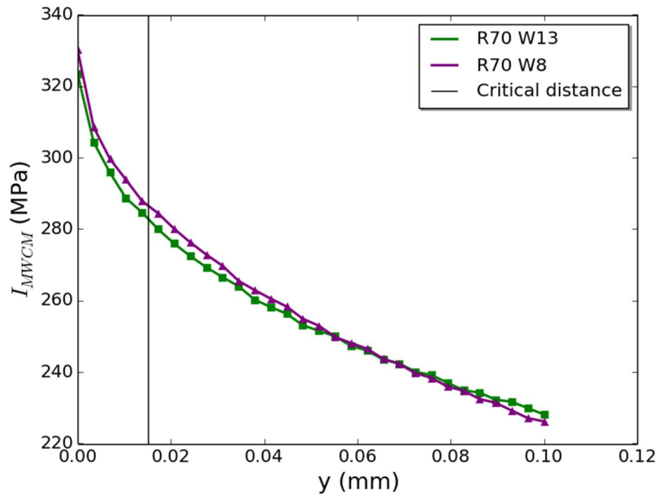
Figure 5-4: Evolution of the stress under the contact at x/a = -1 for both specimens widths (For W_{13} : \sigma_{B,max}/p_0 = 0,36 ; Q/fP = 0,43 . For W_8 : \sigma_{B,max}/p_0 = 0,24 ; Q/fP = 0,63 ).
