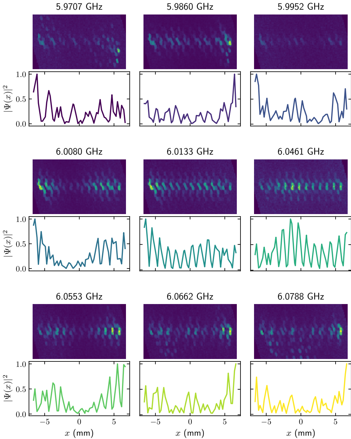
Figure 5.15: Profile of the edge states along the domain wall for ArmchairSi . The modes are organized by ascending frequency. For this system, the periodicity of the domain wall is twice the periodicity of the lattice
