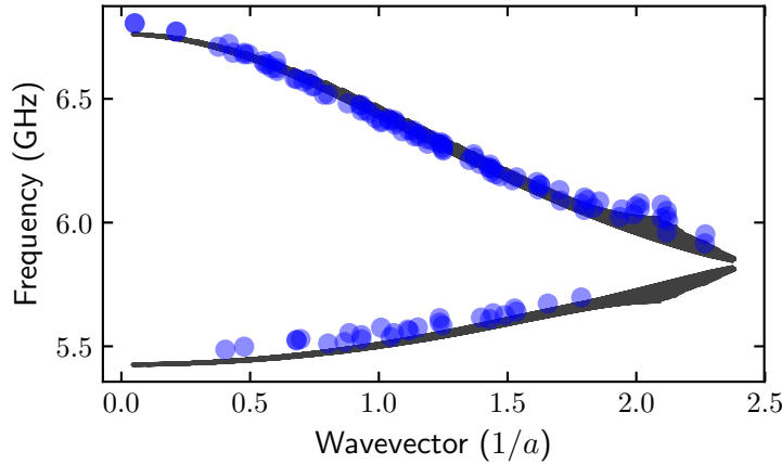
Figure 3: Dispersion relation of the resonant modes of a honeycomb lattice of superconducting resonators. The experimental data points come from the measurement of ZigzagSi . They are in good agreement with the predictions of an ab initio model of the lattice.
