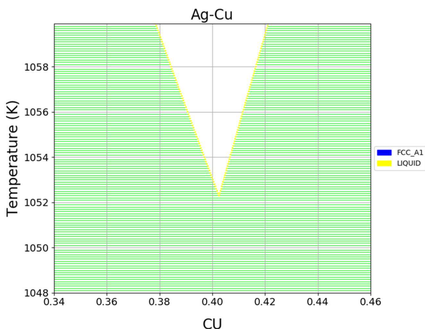
Figure 66 Eutectic point calculated for the Ag-Cu alloy
