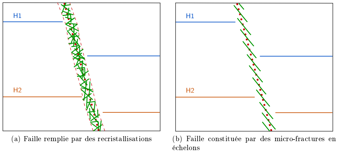
FIGURE 6.3 – Zone faillées
