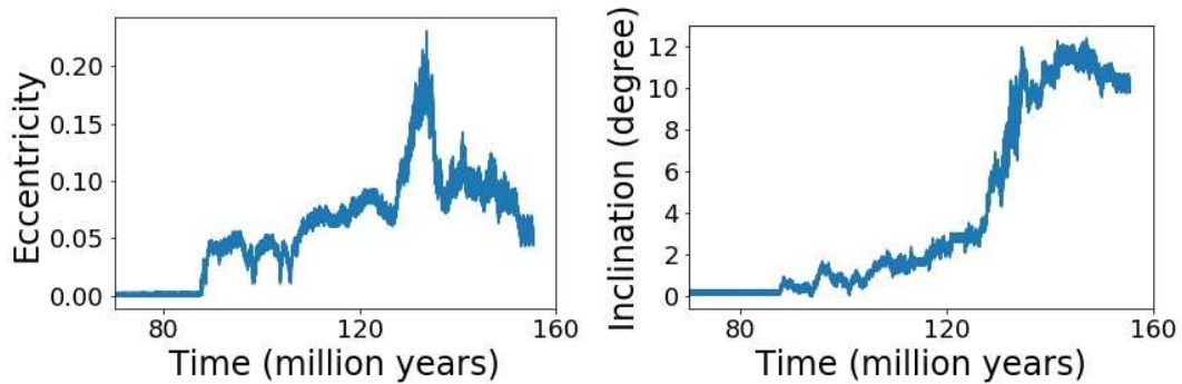
FIGURE 5.18: Example of a simulation showing post-resonance eccentricity and inclination compatible with Iapetus' actual orbit. Here, the resonance is crossed 90 millions years after the start of the simulation. As Iapetus evolve chaotically during the crossing, its eccentricity raises over 0.2, while the tilt also increases to over 10 degrees. On such an orbit Iapetus is expected to get ejected, but at the end, before getting out of the resonance, the eccentricity decreases to 0.05 while the tilt stays well over the value we observe today. This simulation was done with Q=1500
