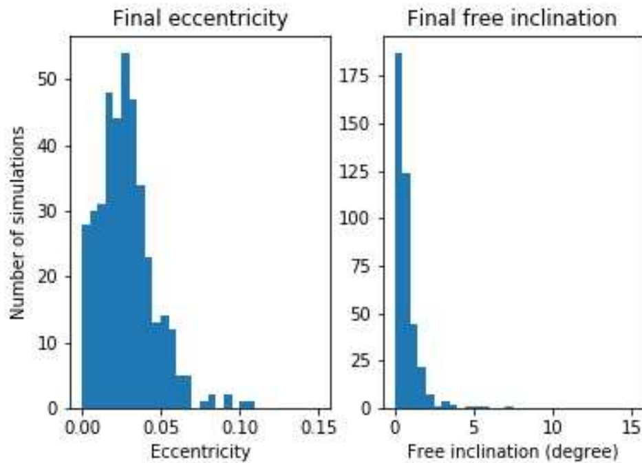
FIGURE 5.11: Post-resonant eccentricities and inclinations using Q=100 . Out of 400 simulations, 5 end with the ejection of Iapetus, 1 shows a smooth evolution of its inclination and 5 show a smooth evolution of its eccentricity.
