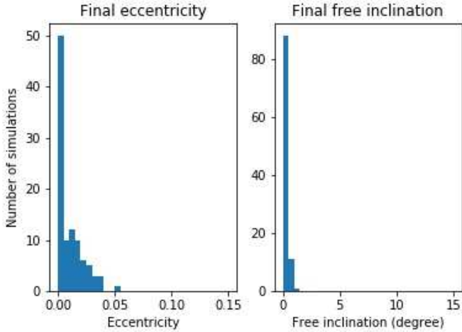
FIGURE 5.6: Post-resonant eccentricities and inclinations using Q=20 .
