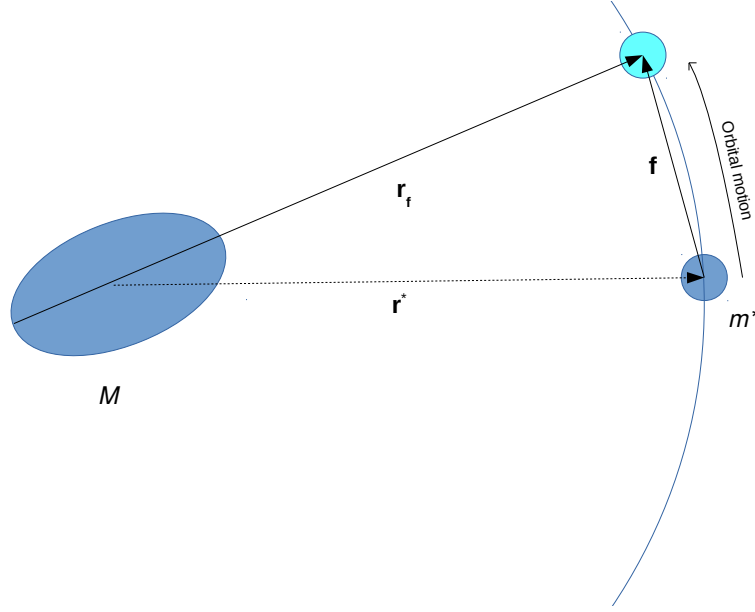
FIGURE 1.6: The lag \mathbf{f} is usually not constant in the case of an eccentric orbit for instance but some approximation can be made \mathbf{f} = \Delta t r |\Omega_p - n|
