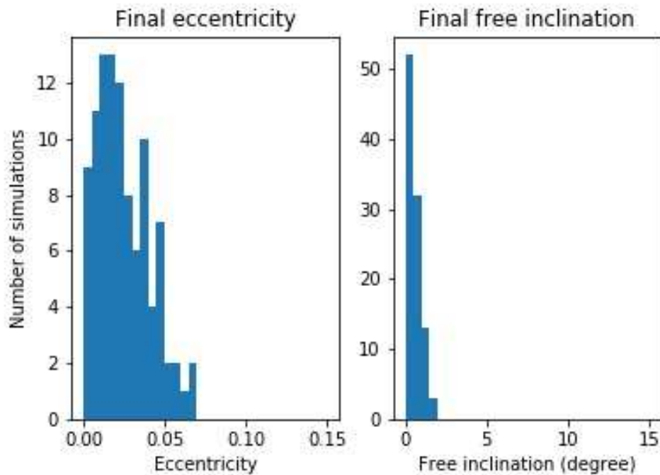
FIGURE 5.8: Post-resonant eccentricities and inclinations using Q=75
