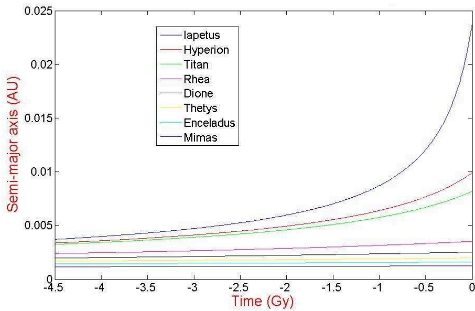
FIGURE 1.9: Semi-major axis evolution of the satellites of Saturn under Fuller's model. No mutual gravitational influence between satellites was introduced.
