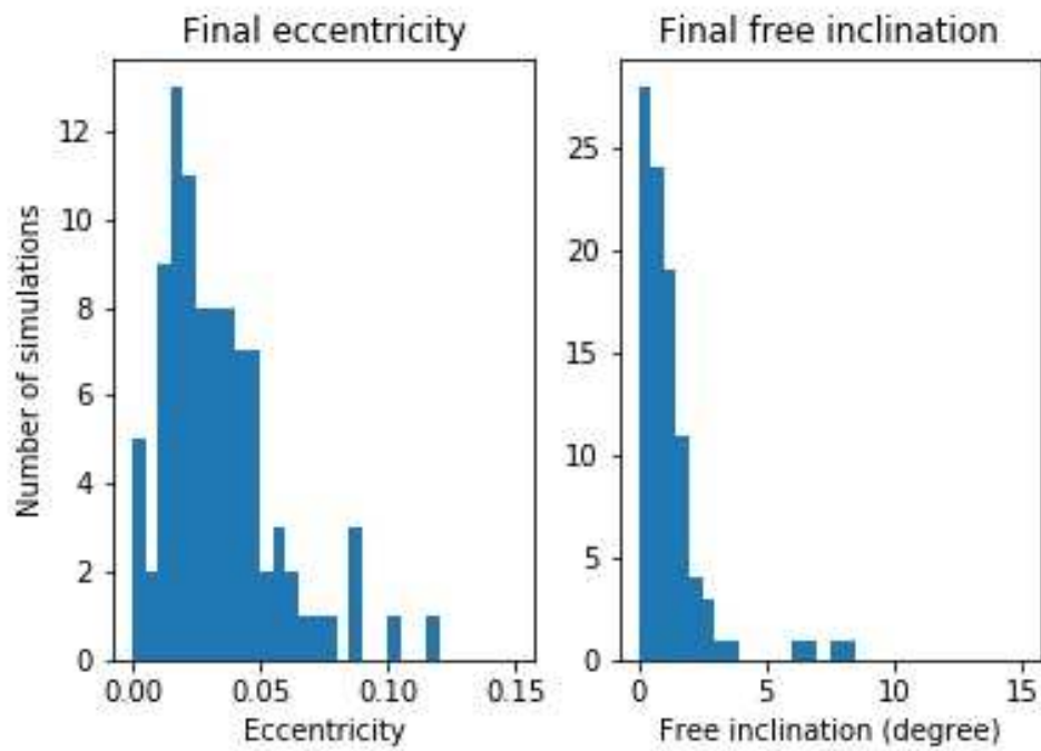
FIGURE 5.23: Post-resonant eccentricities and inclinations using Q=200 . Out of 100 simulations, 22 end with the ejection of Iapetus.
