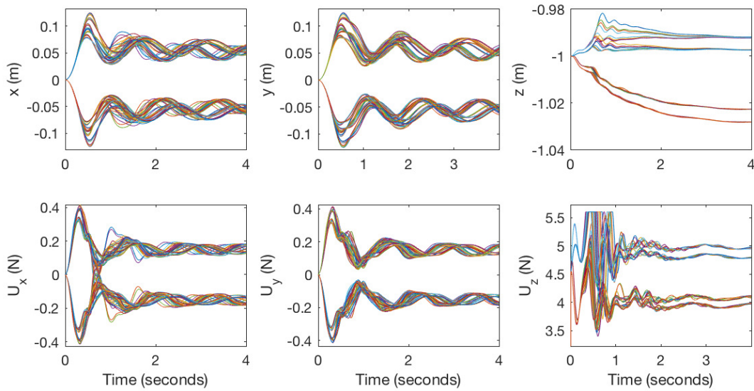
Figure 5.22: Positions (x, y, z) and their respective qc-SMC inputs considering fixed D_i , quadrotor model influenced by coefficients incertitude, and combinations of wind speed steps with reduced amplitude.
