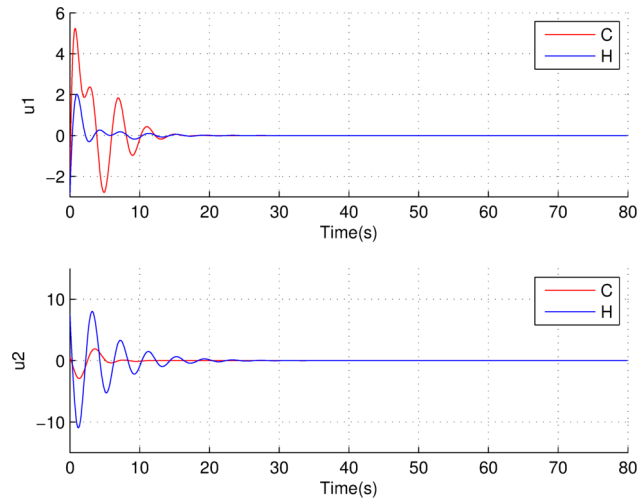
(a) Inputs u_1 and u_2
