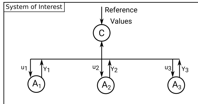
Figure 3.5: Centralized Paradigm: one controller and multiple actuators.
