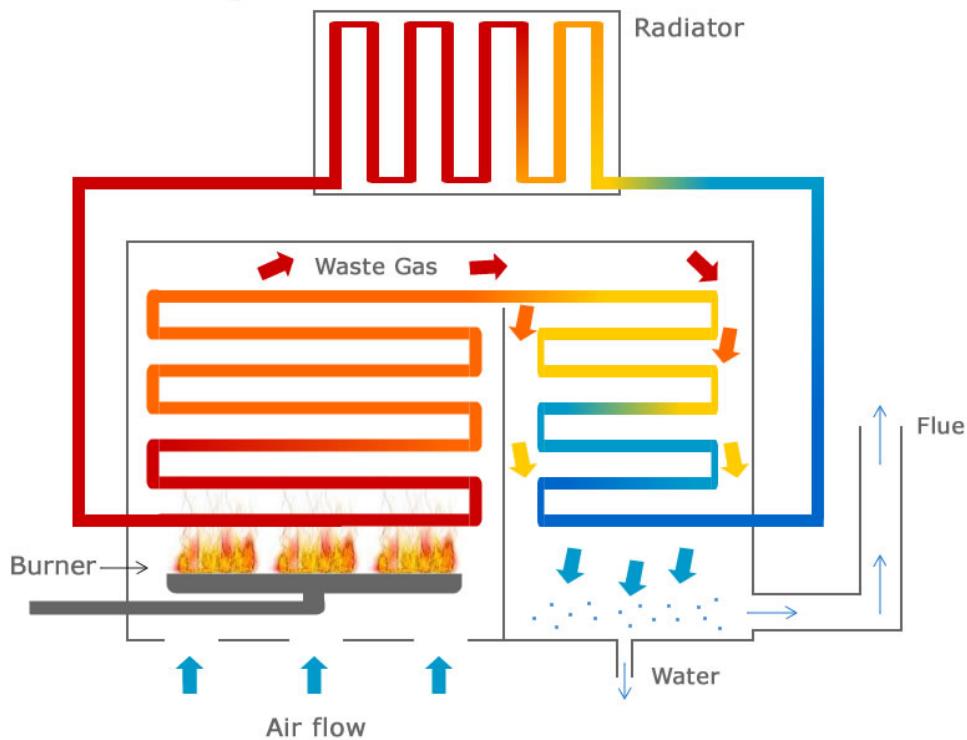
Figure 3.2: Water Heater Scheme 1 .
