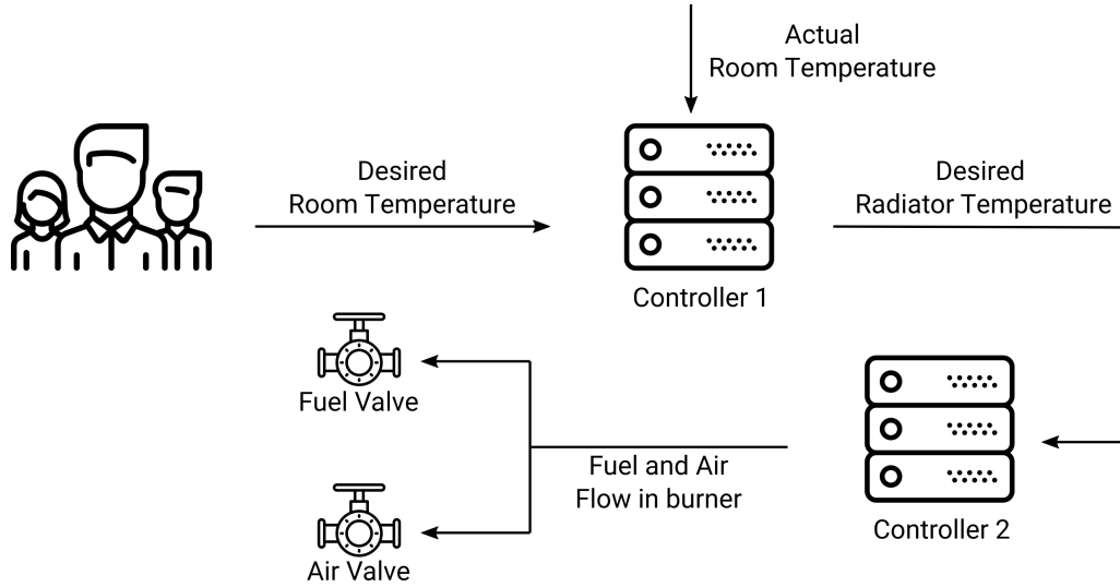
Figure 3.4: Boiler-Room control chain: from high-level to low-level control.
