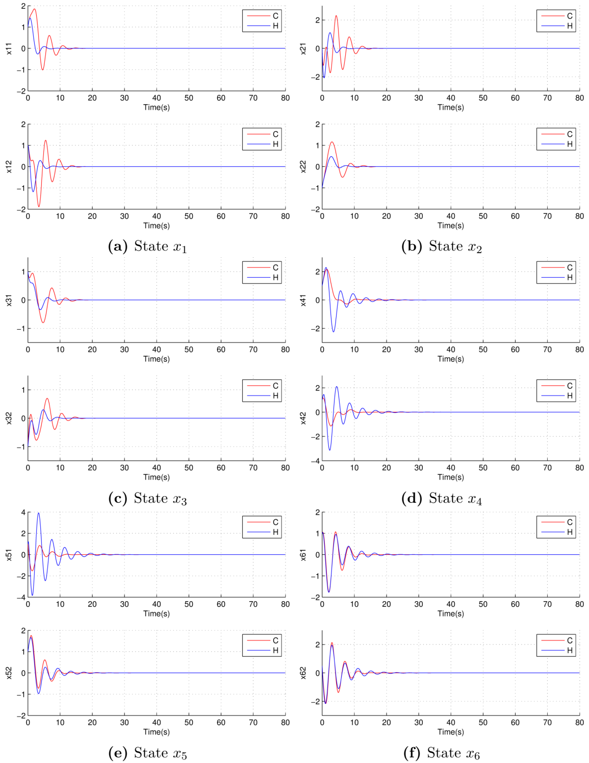
Figure 3.8: The states x_i of the simulated system.
