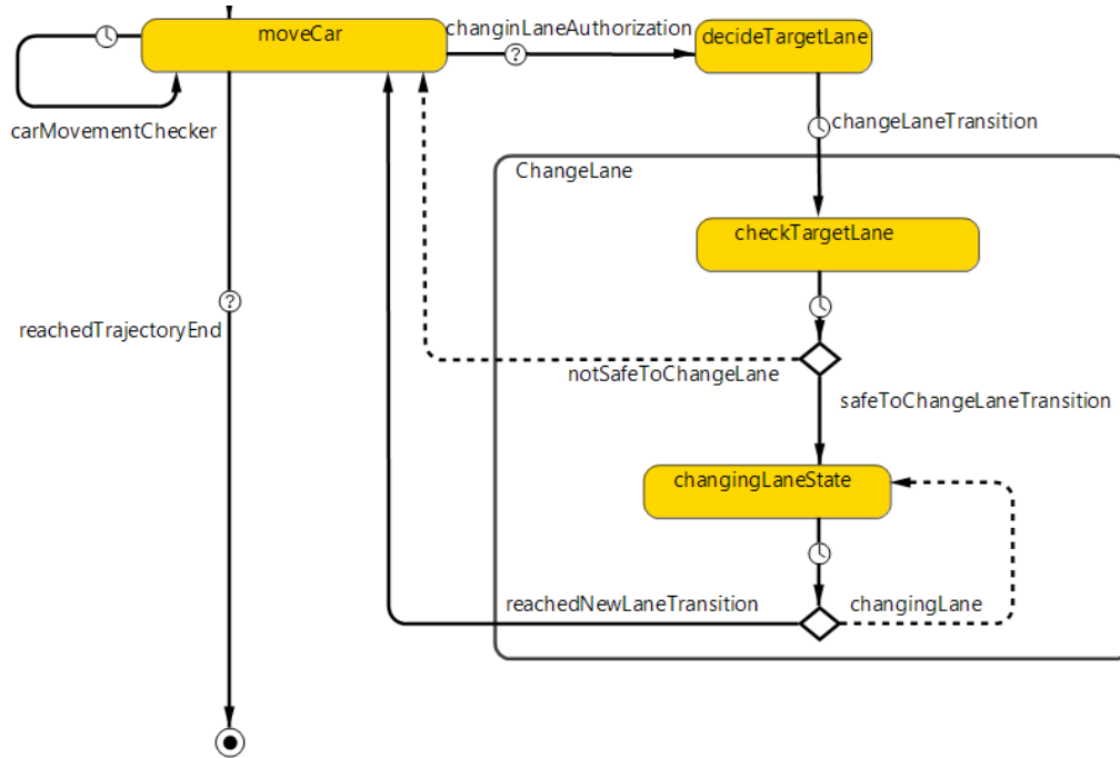
Figure 6.13: The state chart that describes the logic given to agents in Anylogic.
