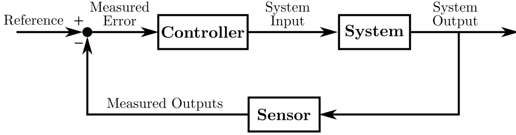
Figure 3.1: Typical system control: a controller computes the system input based on the error between the measured system output and the reference.
