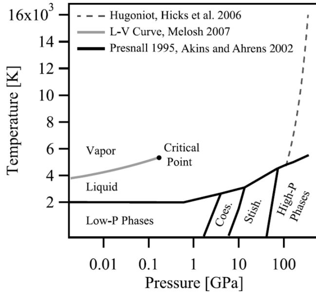
Figure 2.8: Phase diagram for fused silica taken from Ref. [174] indicating fused silica phases such as low-pressure phase, liquid and vapor phases, coesite, stishovite and high-pressure phases.
