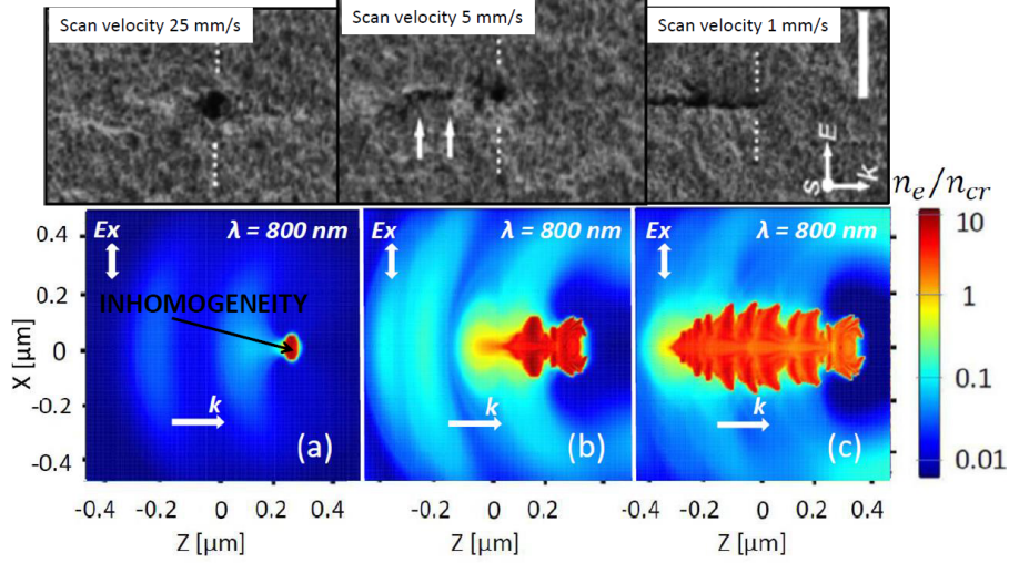
Figure 4.8: Electron density snapshots are calculated by coupled 2D-FDTD demonstrating the evolution from a single inhomogeneity of radius R = 5 \text{ nm} localized in (0.3, 0) \mu\text{m} to nanoplasmic structure taken at (a) 40 fs before the pulse peak, (b) at the pulse peak, (c) 40 fs after the pulse peak. Laser irradiation conditions: pulse duration \theta = 120 \text{ fs} (FWHM), irradiation wavelength \lambda = 800 \text{ nm} , pulse energy E = 300 \text{ nJ} . Here and further, electron density is normalized to its critical value at 800 nm n_{cr} = 1.74 \times 10^{27} \text{ m}^{-3} and \vec{k} is the incident laser wave vector. SEM images are taken from Ref. [18] at different scan velocities. Experimental details: pulse energy 50 nJ, pulse duration 100 fs at central wavelength 800 nm, repetition rate 250 KHz and focusing conditions NA = 1.1 . Scale bar 1 \mu\text{m} .
