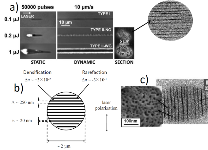
Figure 1.1: a) Ultrashort laser-induced modifications in fused silica taken from Refs. [4,5]. b) Composition of self-organized nanogratings (illustration from Ref. [6]). c) [taken from Ref. [7]] shows nanogratings consisting of nanopores.
