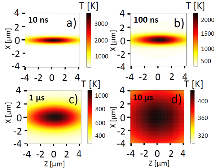
Figure 6.8: Spatial temperature dynamics during fast cooling of fused silica. Temperature snapshots are taken (a) 10 ns, (b) 100 ns, (c) 1\mu\text{s} and 10\mu\text{s} after laser irradiation. The laser pulse energy is 4\mu\text{J} . Laser irradiation conditions: pulse duration \theta = 80 fs (FWHM), irradiation wavelength \lambda = 800 nm, beam waist w_0 = 1\mu\text{m} .
