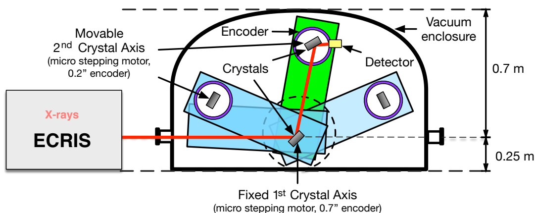
Figure 1.4 – Schematic of the top view of the DCS. Both crystals are installed in a single table that rotates around the 1 st crystal axis. The detector is mounted also in the table and is with a rotation trajectory is concentric with the 2 nd crystal axis.
