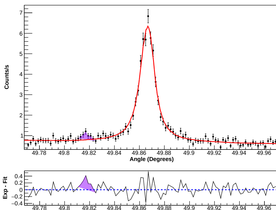
Figure B.1 – Example of a dispersive spectrum of the 1s2s^22p^1P_1 \rightarrow 1s^22s^2^1S_0 transition. The red full curve is the fit from simulation performed with the obtained energy and natural width. The purple shadow area highlights the observed small peak and at the bottom the fit residuals are shown.
