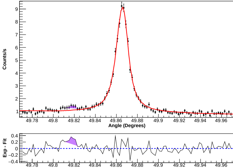
Figure B.3 – Example of a dispersive spectrum of the 1s2s^22p^1P_1 \rightarrow 1s^22s^2^1S_0 transition. The red full curve is the fit from simulation performed with the obtained energy and natural width. The purple shadow area highlights the observed small peak and at the bottom the fit residuals are shown.
