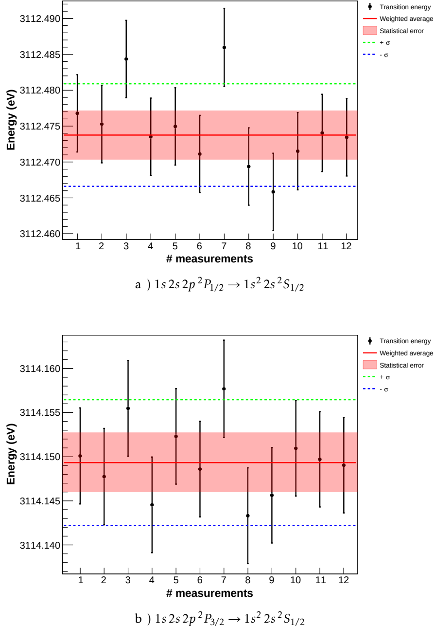
Figure 4.17 – Li-like argon 1s2s2p^2P_J \rightarrow 1s^22s^2S_{1/2} , J = 1/2, 3/2 doublet transition energy values of the different pair of dispersive and non-dispersive spectra recorded during the experiment. Error bars correspond to statistical uncertainty obtained from Eq. (4.3) quadratically combined with the uncertainties in the temperature and angle measurement. Red full curve corresponds to the weighted average mean, obtained considering only the statistical uncertainty in each point. The pink shaded area corresponds to the statistical uncertainty and the dashed blue and green lines ( \pm\sigma ) represent the total uncertainty obtained by the quadratically combination of the statistical uncertainty and all the contributions given on Table 3.1. Every pair of points correspond to one-day data taking.
