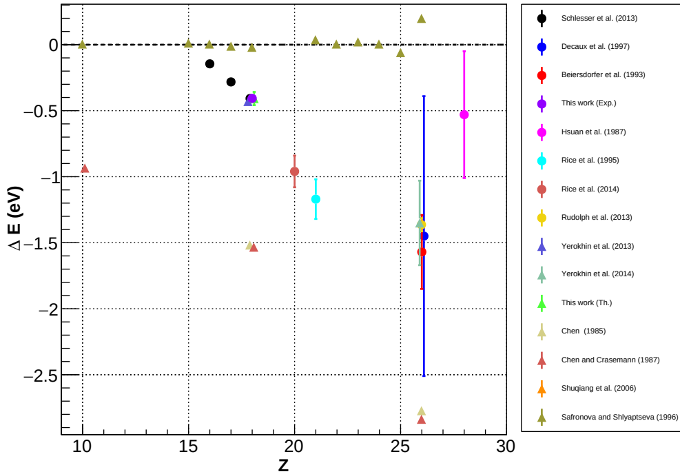
Figure 4.10 – Comparison between experimental and theoretical values for the 1s2s^2 2p^1 P_1 \rightarrow 1s^2 2s^2 ^1S_0 transition energies, as a function of Z . Round dots represents experimental results and triangular ones theoretical results. All values are compared to the energies in Ref. [285]. Experimental results references: Schlesser et al. (2013) [138], Beiersdorfer et al. (1993) [282], Decaux et al. (1997) [283], Rudolph et al. (2013) [11], Hsuan et al. (1987) [273], Rice et al. (1995) [260], Rice et al. (2014) [259]. Theoretical results references: Yerokhin et al. (2015) [231], Yerokhin et al. (2014) [286], Chen and Crasemann (1987) [280], Chen (1985) [287], Safronova and Shlyaptseva (1996) [279]. For the same Z , some values have been shifted in Z so one can notice the different points. The value of Shuqiang et al. (2006) [288] for Z = 29 is out of the selected energy range difference.
