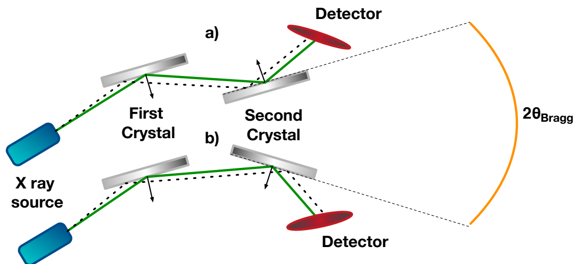
Figure 1.3 – Illustration of the two measuring modes of the DCS. The non-dispersive mode (a) where the crystals are geometrically parallel (also called parallel mode) and the dispersive mode (b), where the crystals deflect the x rays in the same direction (also called antiparallel mode).
