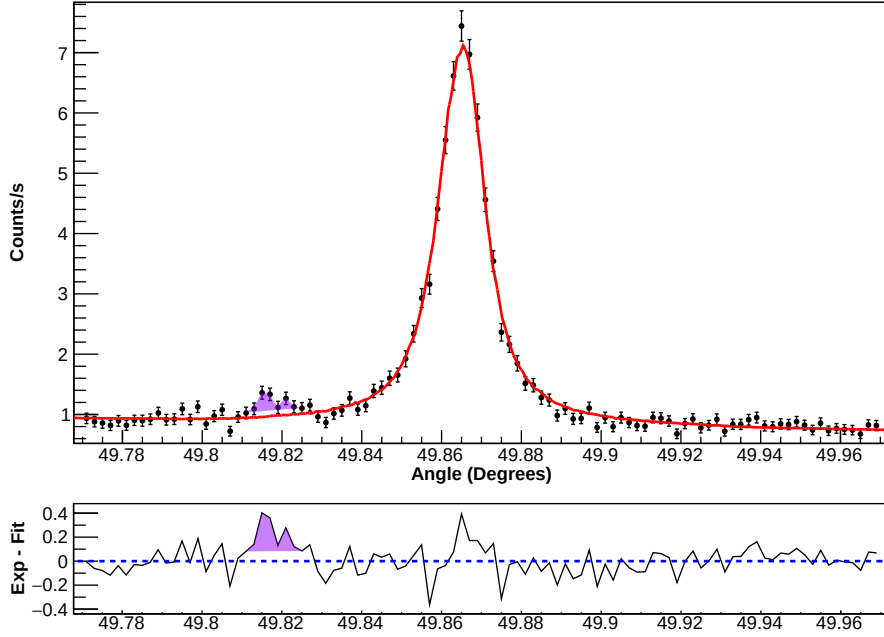
Figure B.2 – Example of a dispersive spectrum of the 1s2s^22p^1P_1 \rightarrow 1s^22s^2^1S_0 transition. The red full curve is the fit from simulation performed with the obtained energy and natural width. The purple shadow area highlights the observed small peak and at the bottom the fit residuals are shown.
