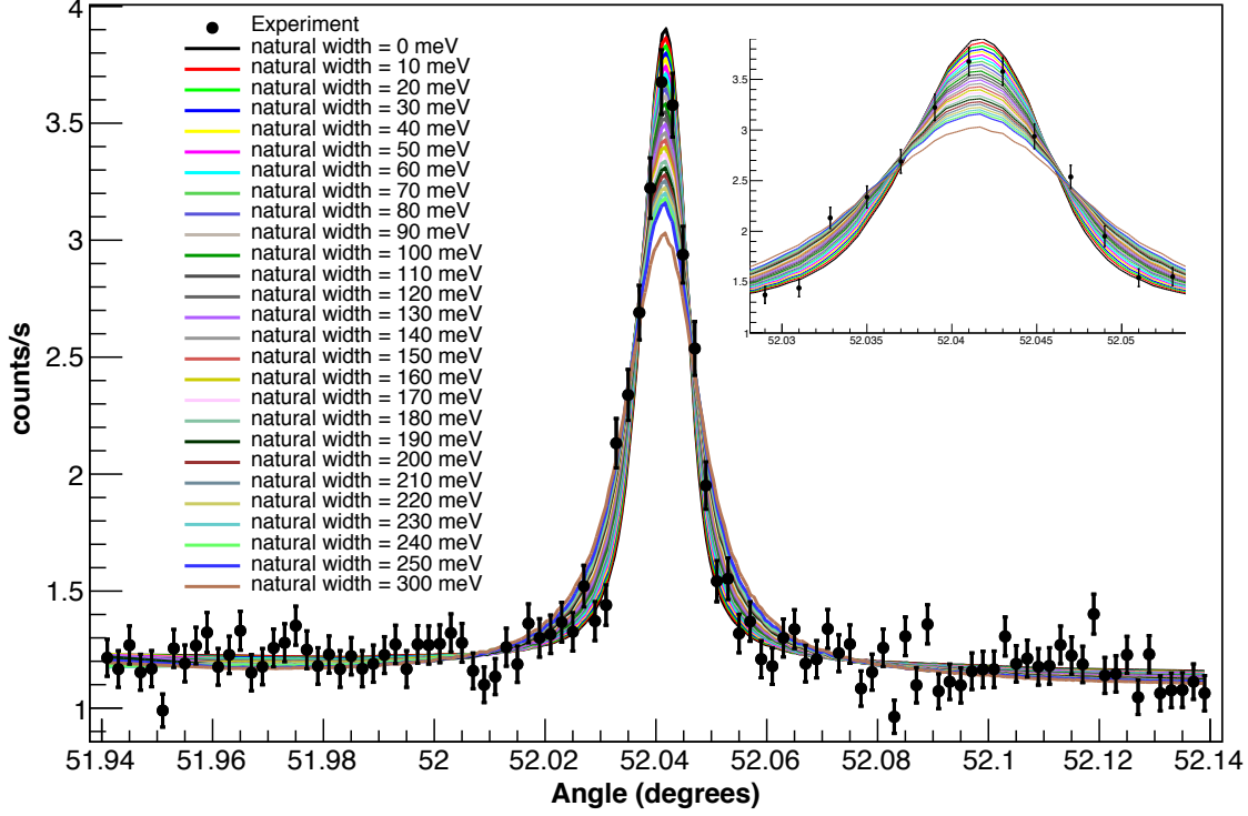
Figure 2.1 – Example of fit to the dispersive spectrum of the 1s2s^1P_1 \rightarrow 1s^2^1S_0 transition by interpolated simulations spectra for a set of Lorentzian widths. In the legend, the color and Lorentzian width of each fit is shown ranging from \Gamma_L = 0 meV to \Gamma_L = 300 meV. The error bar in each point is the \sqrt{n}/t , being n the number of counts and t the time spent in the bin.
