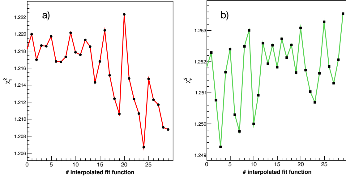
Figure 2.4 – \chi^2_r value as function of the fit number of each simulated spectrum of both dispersive (a) and non-dispersive modes for the fits shown on Fig. 2.3.
