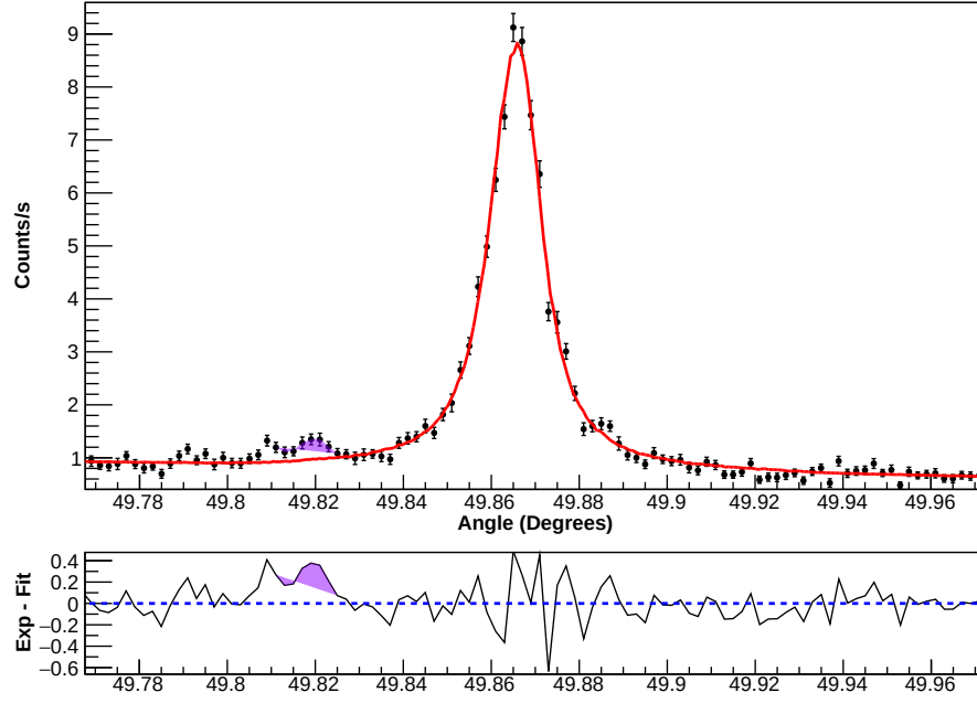
Figure B.4 – Example of a dispersive spectrum of the 1s2s^22p^1P_1 \rightarrow 1s^22s^2^1S_0 transition. The red full curve is the fit from simulation performed with the obtained energy and natural width. The purple shadow area highlights the observed small peak and at the bottom the fit residuals are shown.
