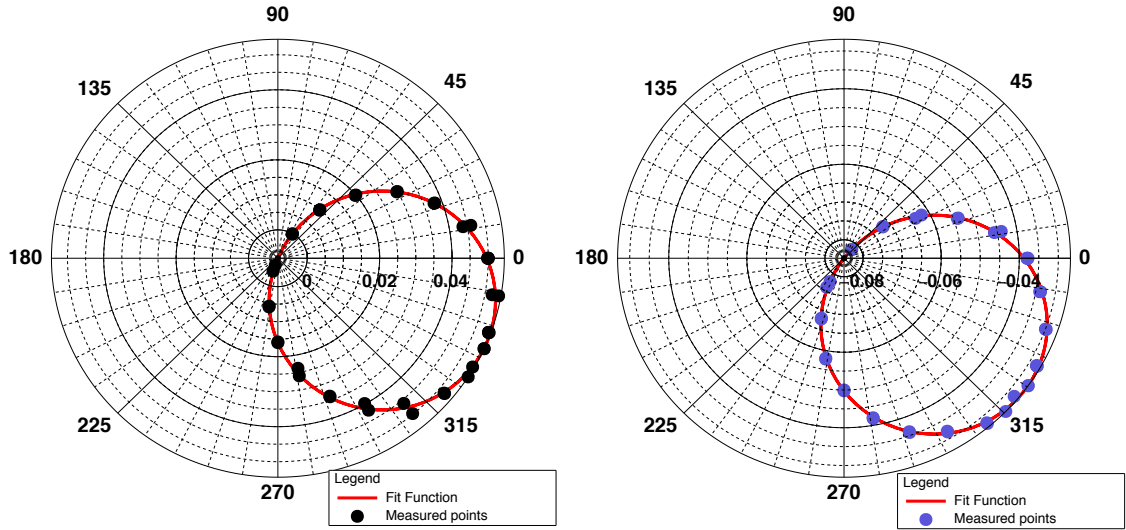
Figure 3.2 – Polar plot of the vertical tilt measured the Zerotrionic sensor as a function of the crystals supports horizontal angle correspondent to the data of Fig 3.1, being the left plot (black dots) corresponding to the first crystal support and the plot on the right (blue dots) corresponding to the second crystal support. The fit function from Eq. (3.1) is also plotted.
