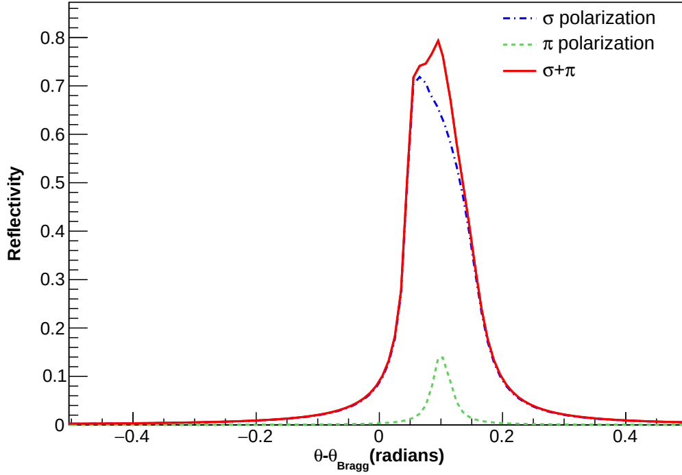
Figure 1.6 – Reflectivity curve (diffraction profile) of Si(111) crystals calculate with Xcristal from the XOP [217–219] for the 1s\,2p\,^1P_1 \rightarrow 1s^2\,^1S_0 transition energy of 3139.5821 eV taken from Artemyev et al. (2005) [125]. The \sigma (blue dashed line) and \pi (green dotted line) polarizations profiles and the unpolarized profile (red full line), obtained by the sum of \sigma + \pi profiles, are shown.
