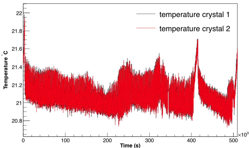
Figure 1.11 – Record of the temperature of crystal 1 thermistor in thermal contact with crystal 2 thermistor, at atmospheric pressure and laboratory temperature during almost 6 days recording. Black line corresponds to the crystal 1 thermistor and red line corresponds to the crystal 2 thermistor.
