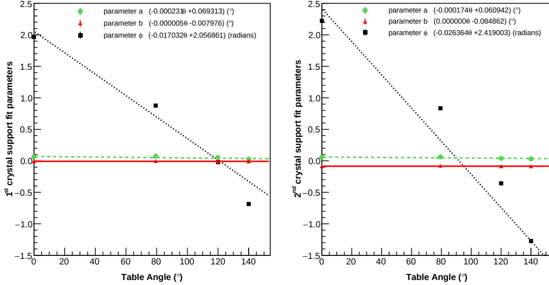
Figure 3.3 – Best fit coefficients for fits performed to the verticality of the crystals supports (see Fig. 3.1) as a function of the table angle for both supports, left plot corresponding to the measurements on the first crystal support and the right plot corresponding to the measurements on the second crystal support). The measurements have been performed at four different table positions: at 0^{\circ} , 79.493^{\circ} , 120^{\circ} and 140^{\circ} . A linear fit is performed at each fit coefficient and its equation is also presented in the legend of each plot.
