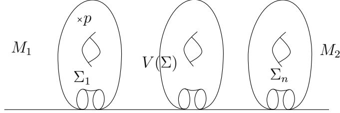
FIGURE 1.3 – The splitting M = M_1 \cup_{V(\Sigma)} M_2 .
