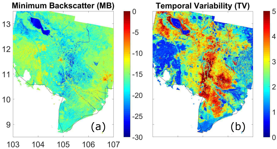
FIGURE 3.14: (a) Minimum backscatter and (b) Temporal variability of the VH polarization over the Vietnam Mekong Delta and Cambodia, calculated from 12 other SAR Sentinel-1 observations in 2016.
