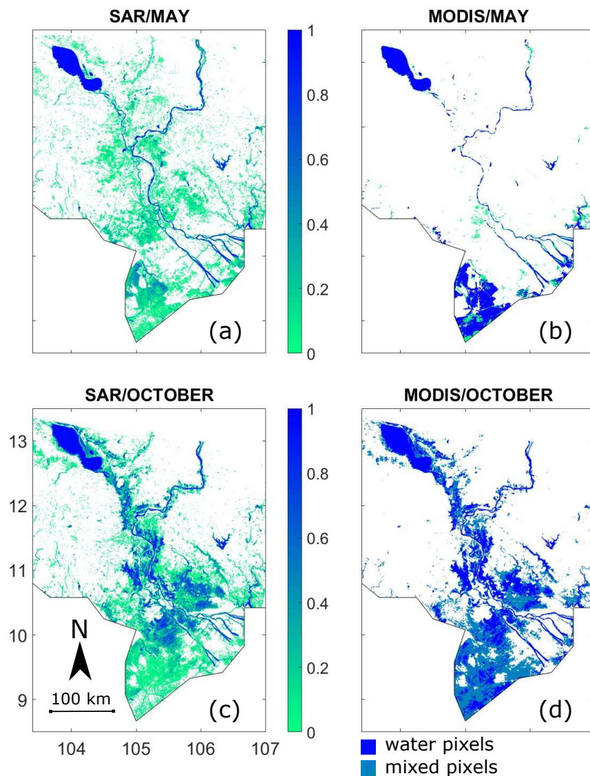
Figure 12. (a,c) SAR and (b,d) MODIS surface water maps at 500 m resolution over the Mekong Delta in May (a,b) and October (c,d) 2015.
