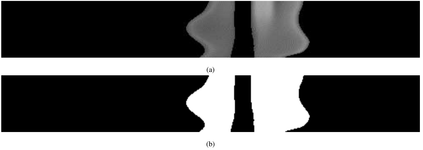
Figure 4.25: Joint reconstruction (a) and segmentation (b) of the metallic part from 500 projections by JMAP
