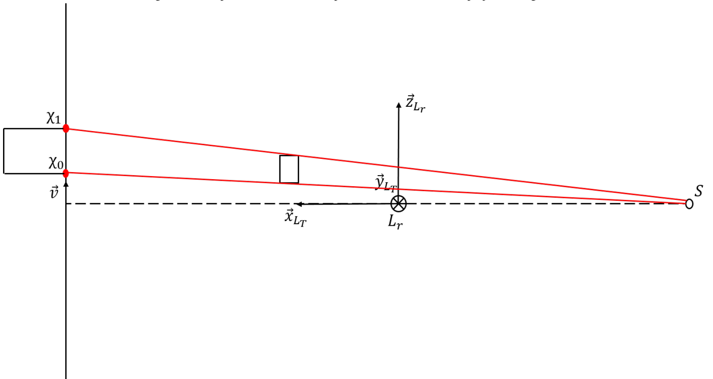
Figure B.4: Rectangular axial footprint of a voxel
