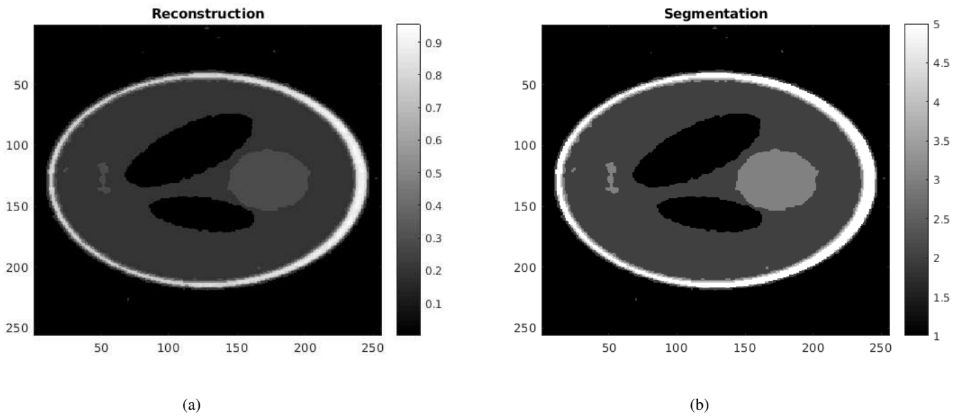
Figure 4.7: Joint reconstruction (a) and segmentation (b) of Shepp-Logan phantom obtained by JMAP with the unmatched RD/VD pair
