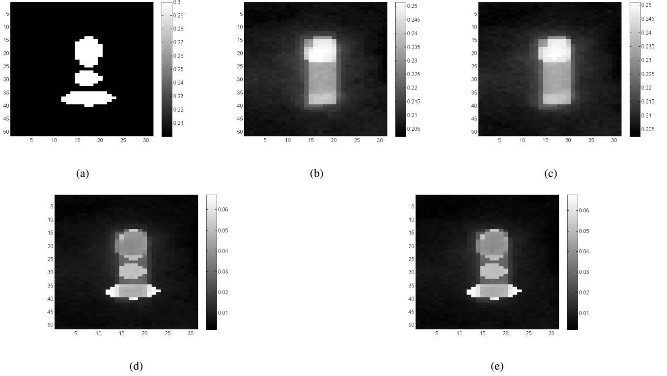
Figure 3.21: Zoom on a region-of-interest with little details for : the real volume (a), the reconstruction by PDFW [OMBF18] with the unmatched RD/VD pair (b), and the reconstruction by PDFW [OMBF18] with the matched SF pair (c). The differences with respect to the original volume are shown in (d) for the unmatched RD/VD pair, and in (e) for the matched SF pair.
