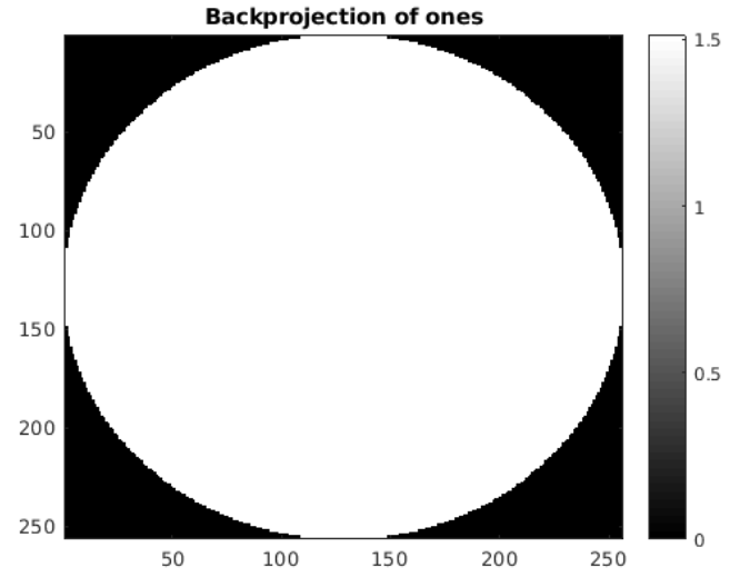
Figure 6.3: Diagonal coefficients of \mathbf{H}^T\mathbf{H} . These coefficients are the size of a volume, of which the middle slice is shown.
