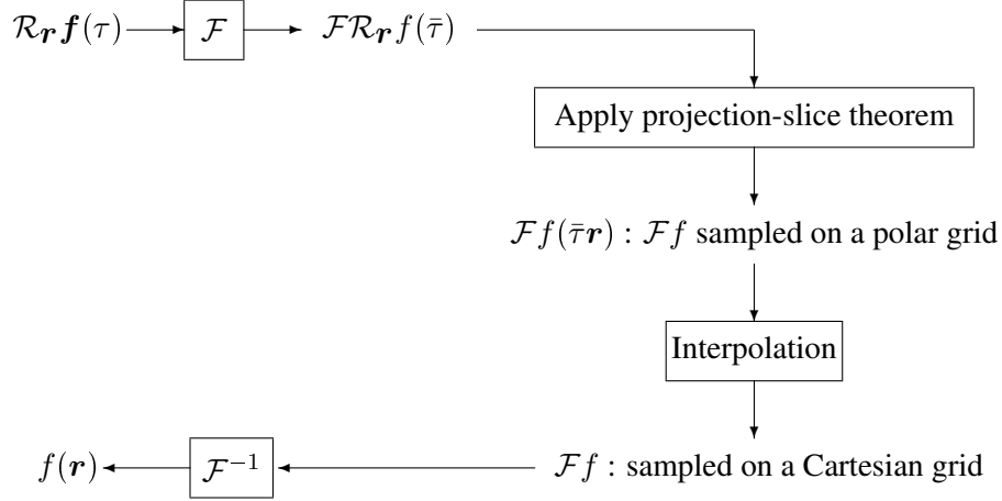
Figure 2.4: Radon transform inversion by the use of projection-slice theorem
