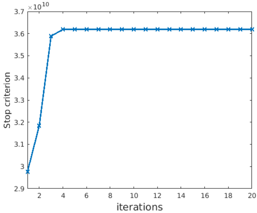
Figure 5.21: Convergence for JMAP with the error-splitting forward model and Gauss-Markov-Potts prior for the reconstruction of the metallic part from 500 projections
