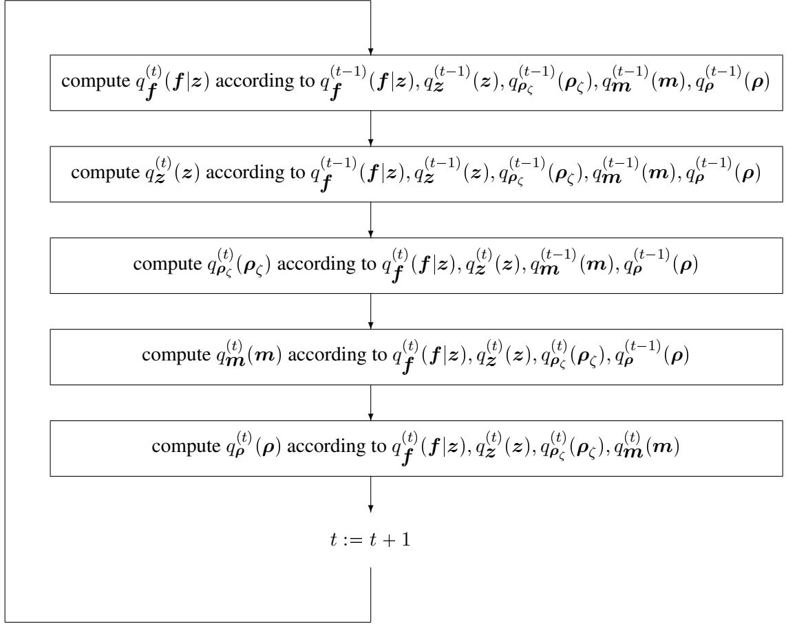
Figure 6.1: Iterative algorithm to compute approximating distribution q(\mathbf{f}, \rho_{\zeta}, \mathbf{z}, \mathbf{m}, \rho)
