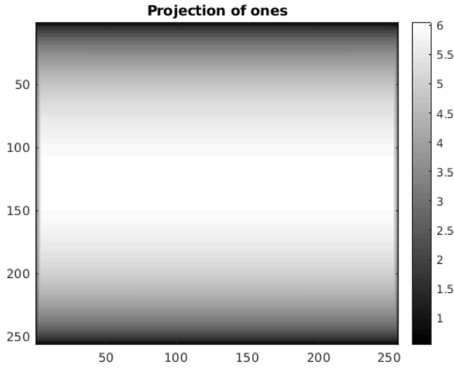
Figure 6.2: Diagonal coefficients of \mathbf{H}\mathbf{H}^T . These coefficients are the size of projections, of which one image is shown.
