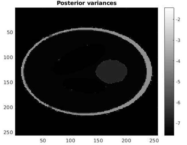
Figure 6.9: Variances obtained by the VBA algorithm jointly with the reconstruction. The variances are shown in logarithmic scale.
