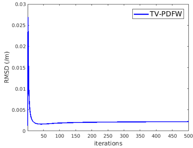
Figure 5.10: Convergence to the reference volume for IQI reconstruction by PDFW [OMBF18]
