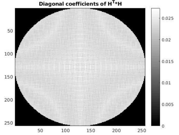
Figure 6.3: Diagonal coefficients of \mathbf{H}^T\mathbf{H} . These coefficients are the size of a volume, of which the middle slice is shown.
