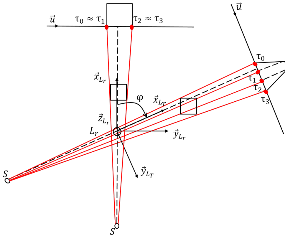
Figure B.3: Trapezoidal transaxial footprint of a voxel at different projection angles
