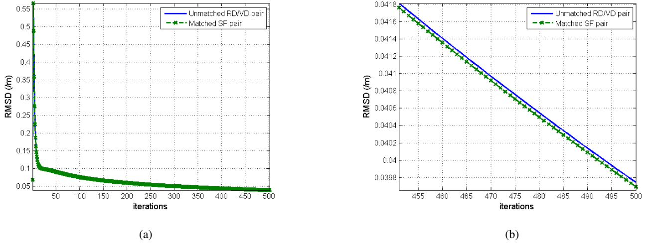
Figure 3.20: Evolution of the Root-Mean Square Difference (RMSD) between the estimate \mathbf{f}^{(t)} and the real volume during PDFW (a) with the RD/VD and SF pairs. A zoom on the last iterations is provided in (b).
