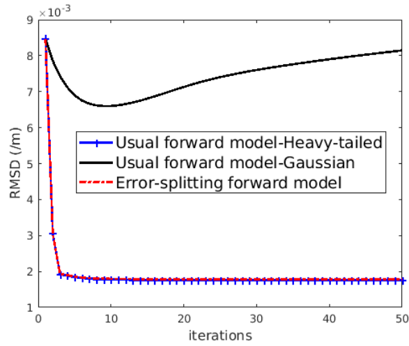
Figure 5.16: Convergence to the reference volume for CMTE reconstruction by JMAP from 300 projections with Gauss-Markov-Potts prior and : the usual forward model modelling \zeta as heavy-tailed, the usual forward model modelling \zeta as Gaussian, and the error-splitting forward model
