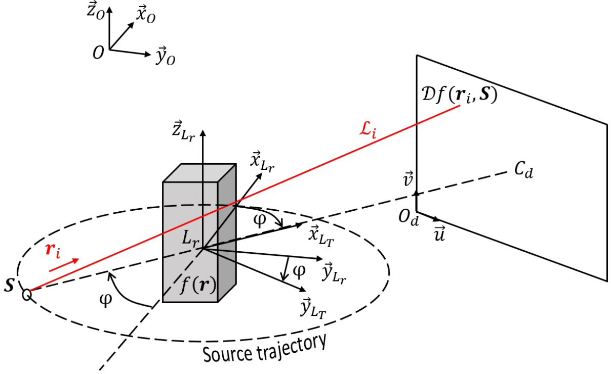
Figure 2.2: Divergent-beam transform
