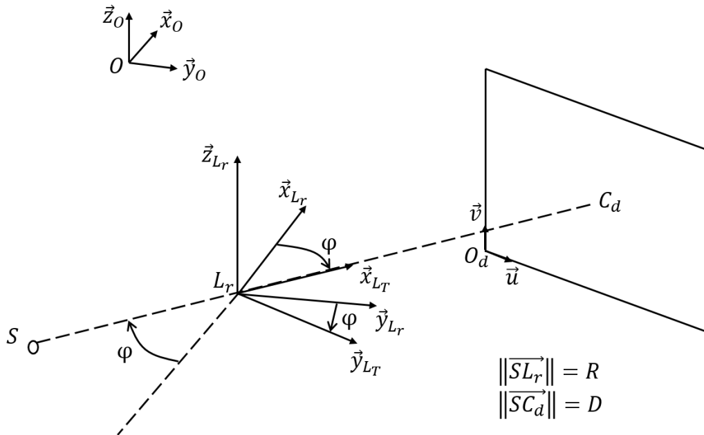
Figure B.1: Geometrical model
