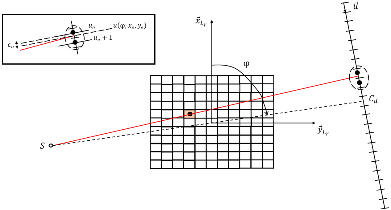
Figure 3.2: Voxel-driven backprojector
