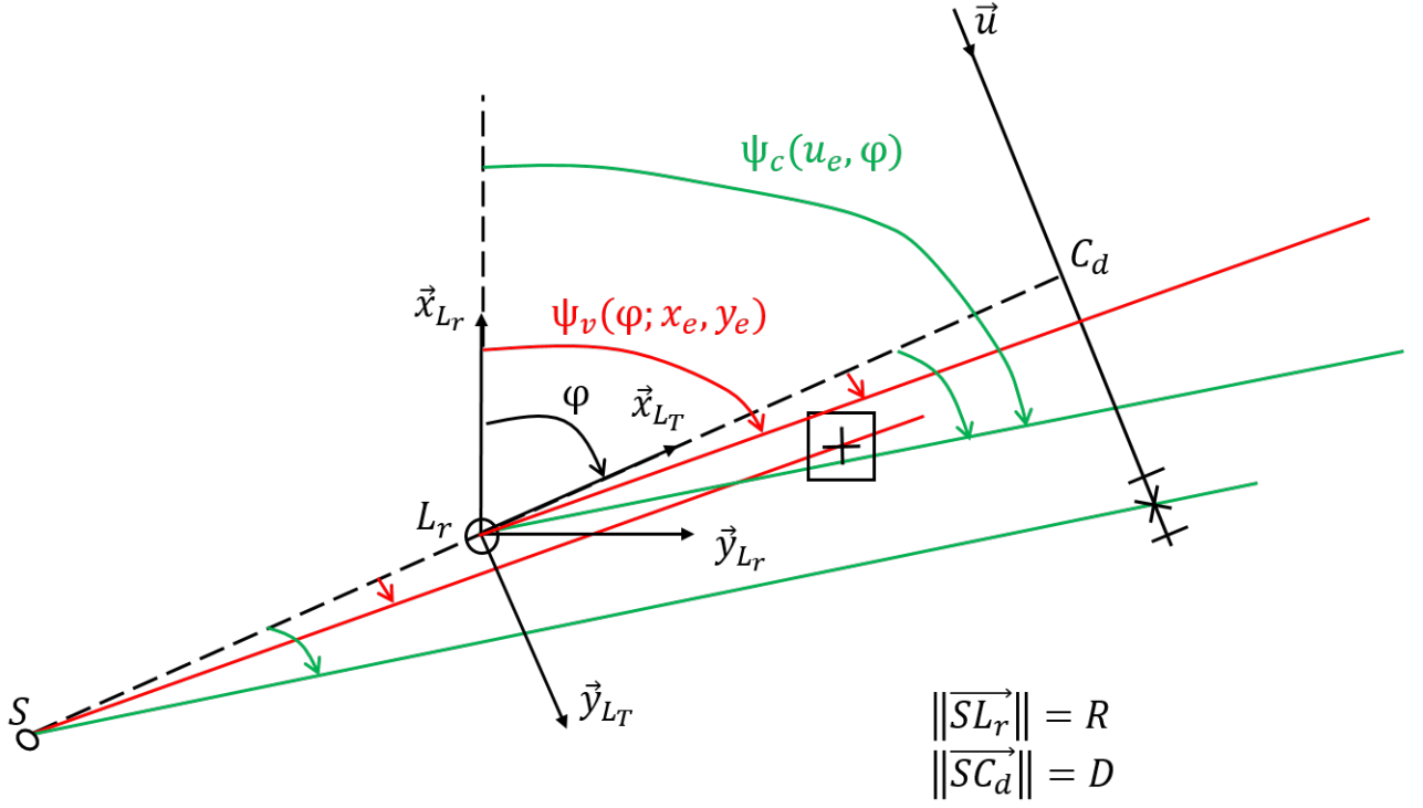
Figure B.5: Azimuthal angles of the ray connecting the source to the center of a cell (u_e, v_e) and of the ray connecting the source to the center of a voxel (x_e, y_e, z_e)
