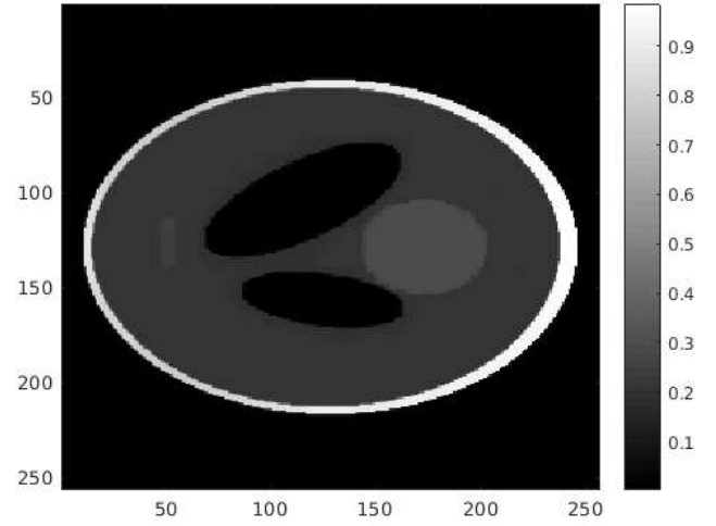
Figure 3.14: Reconstruction of Shepp-Logan phantom by PDFW [OMBF18] with the matched SF pair
