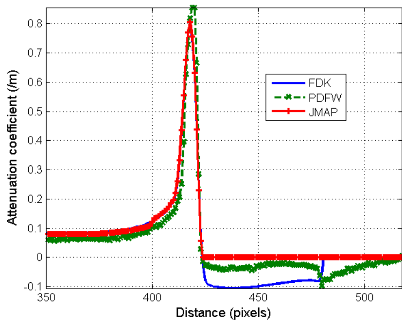
Figure 4.23: Second profile of CMTE for each reconstruction by filtered backprojection [FDK84], PDFW [OMBF18] and JMAP
