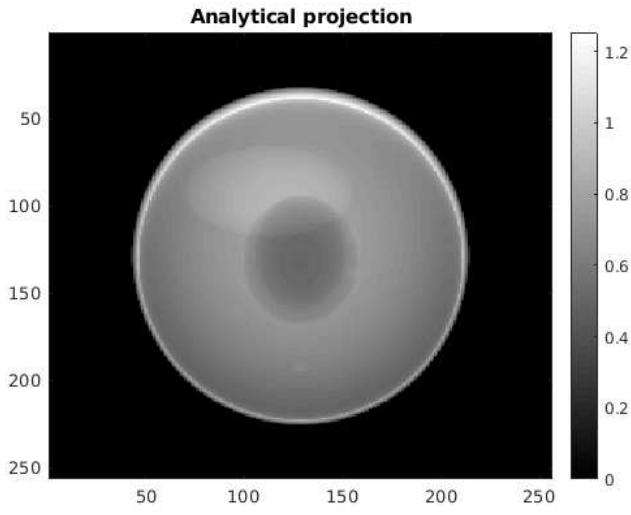
Figure B.9: Analytical projections of the Shepp-Logan phantom
