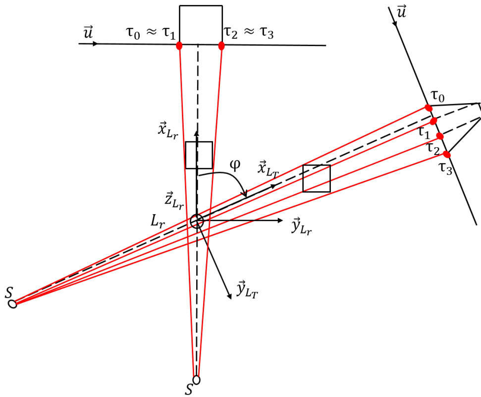
Figure 3.3: Trapezoidal shape of the transaxial footprint of a voxel at different projection angles
