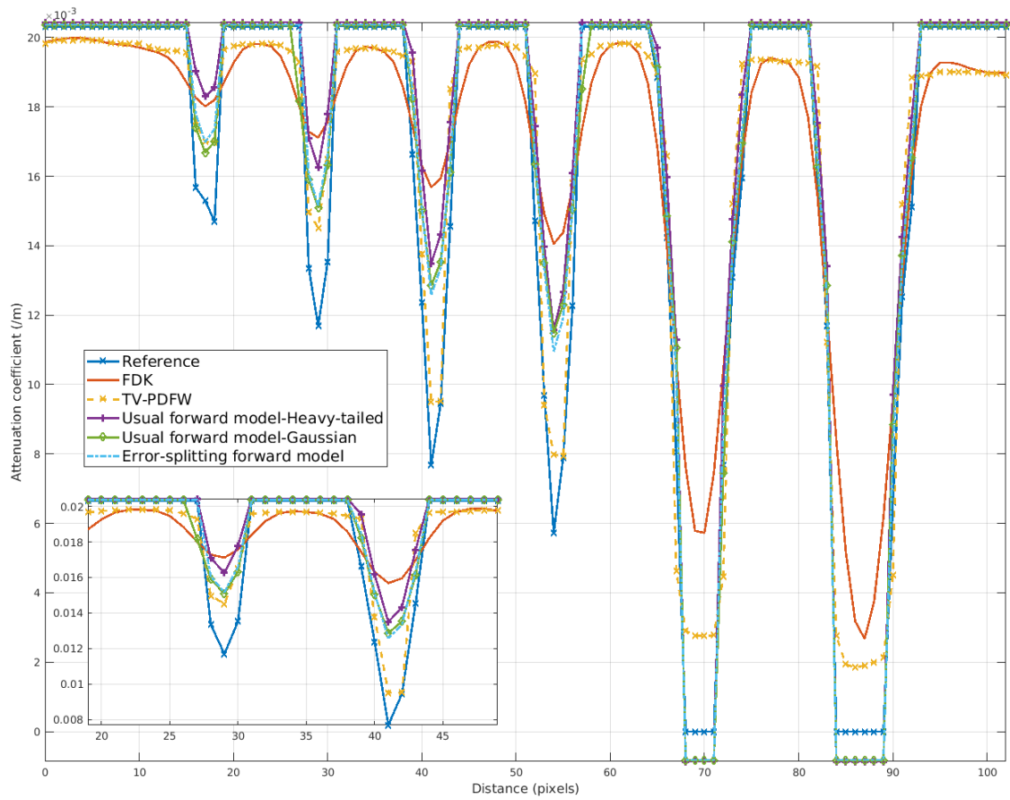
Figure 5.8: Accuracy : profiles of the holes of IQI volume for each reconstruction, with Gauss-Markov-Potts prior for JMAP
