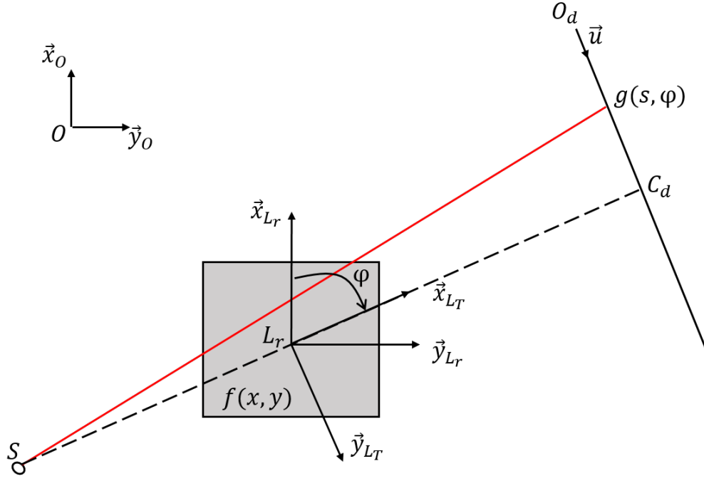
Figure 2.3: Fan-beam CT
