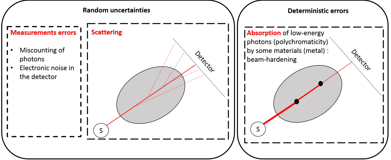
Figure 1.2: Summary of the deviations in the projections with respect to ideal linear projections \mathbf{H}\mathbf{f}
