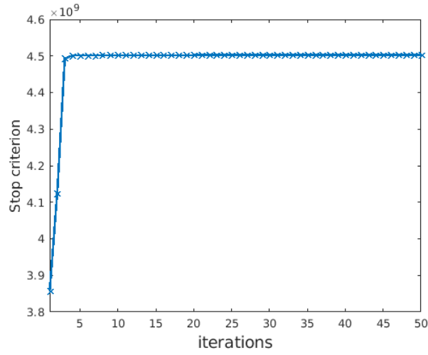
Figure 5.14: Convergence for JMAP with the error-splitting forward model and Gauss-Markov-Potts prior for CMTE reconstruction from 300 projections
