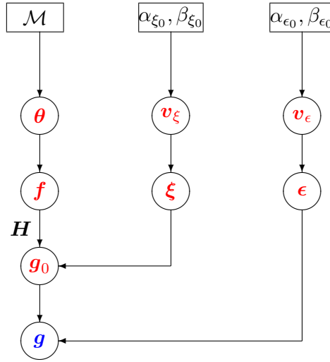
Figure 5.3: General hierarchical model including the error-splitting forward model
