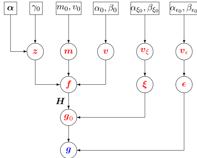
Figure 5.4: Hierarchical model combining the error-splitting forward model and Gauss-Markov-Potts prior on the volume
