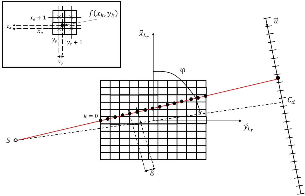
Figure 3.1: Ray-driven projector
