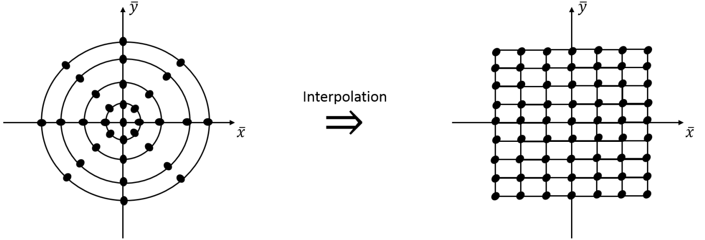
Figure 2.5: Interpolation step from polar to Cartesian grid in Fourier domain [Rod02]
