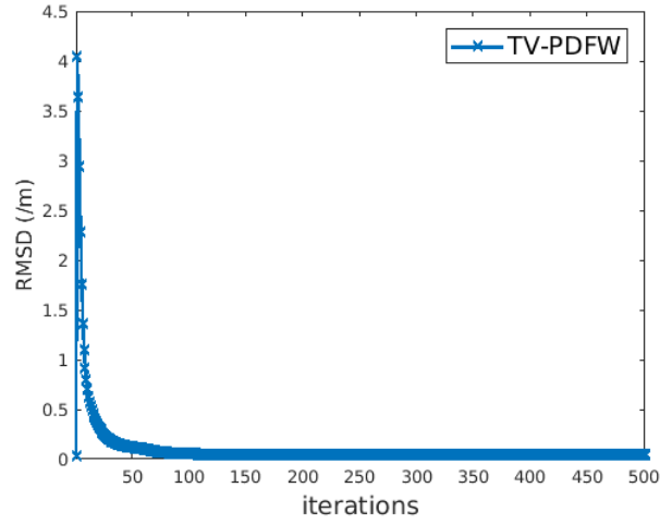
Figure 5.15: Convergence to the reference volume for CMTE reconstruction by PDFW [OMBF18]
