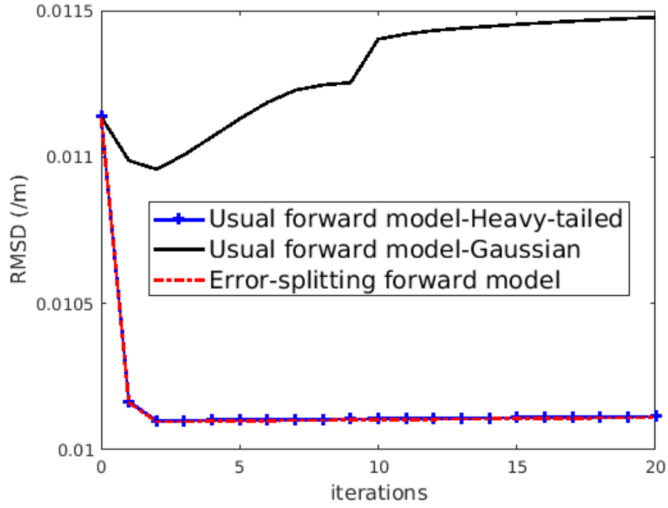
Figure 5.20: Convergence to the reference volume for the metallic part reconstruction by JMAP from 500 projections with Gauss-Markov-Potts prior and : the usual forward model modelling \zeta as heavy-tailed, the usual forward model modelling \zeta as Gaussian, and the error-splitting forward model
