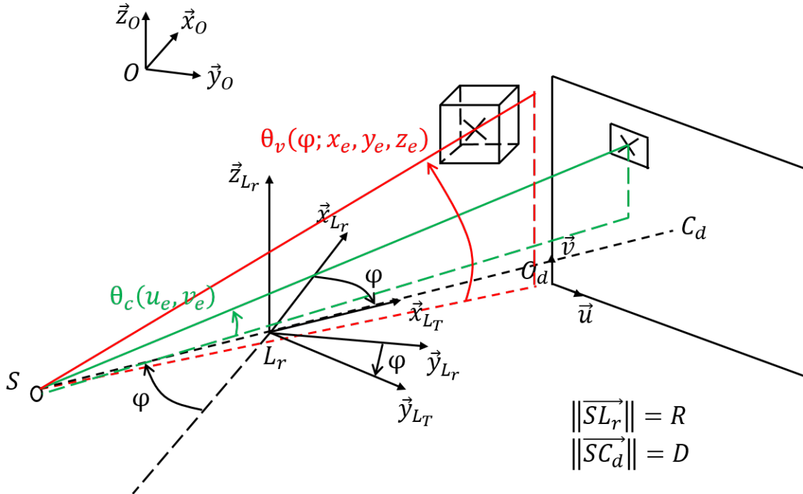
Figure B.6: Polar angles of the ray connecting the source to the center of a cell (u_e, v_e) and of the ray connecting the source to the center of a voxel (x_e, y_e, z_e)
