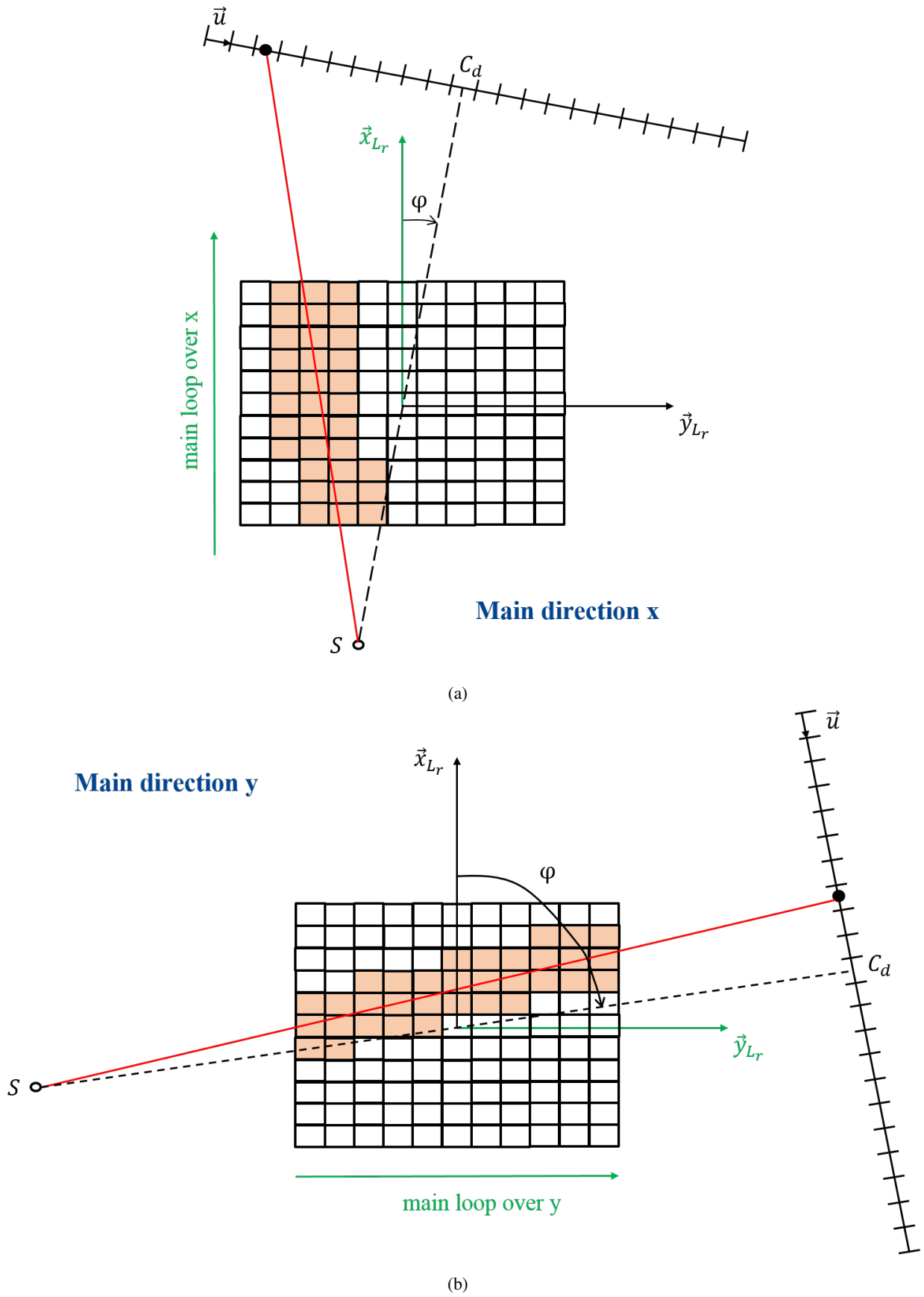
Figure 3.5: Voxels considered by the GPU SF projector depending on whether the main direction is x (a) or y (b)
