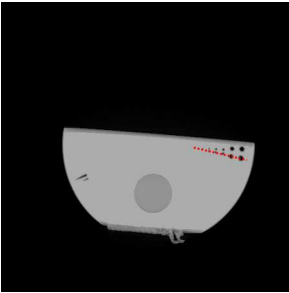
Figure 4.16: Convergence of JMAP for the joint reconstruction and segmentation of IQI volume from 300 projections
