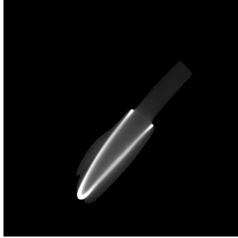
Figure 5.12: Reference for CMTE, reconstructed from 1500 projections (algorithm 12 in chapter 4) (middle slice)
