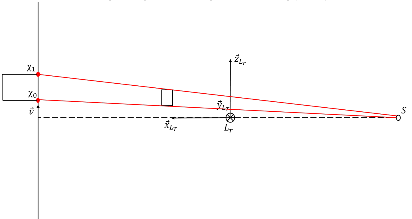
Figure 3.4: Rectangular shape of the axial footprint of a voxel
