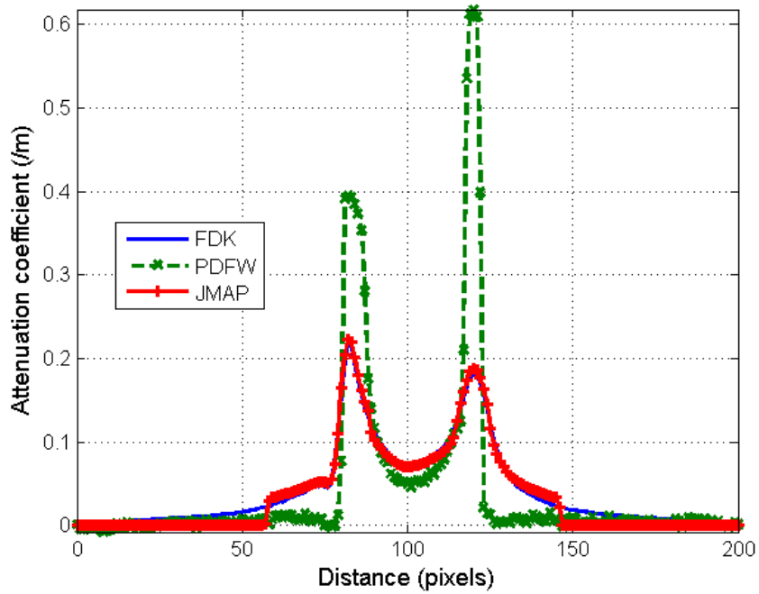
Figure 4.22: First profile of CMTE for each reconstruction by filtered backprojection [FDK84], PDFW [OMBF18] and JMAP
