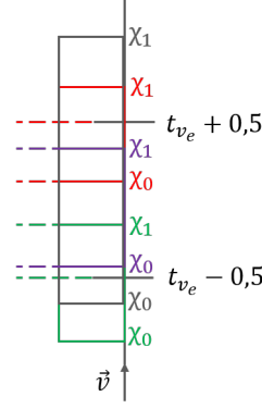
Figure B.8: Different overlaps of the axial footprint of a voxel with a cell
