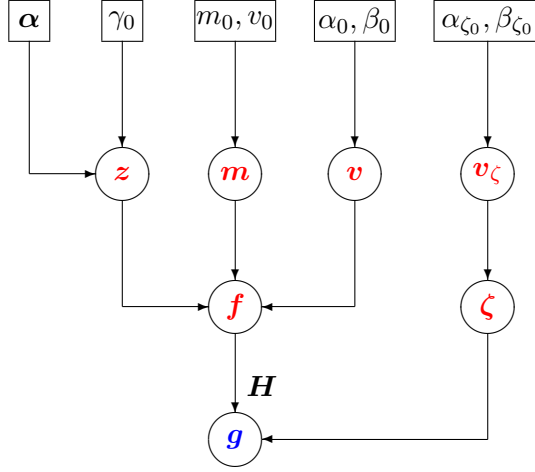
Figure 4.2: Hierarchical model with Gauss-Markov-Potts prior
