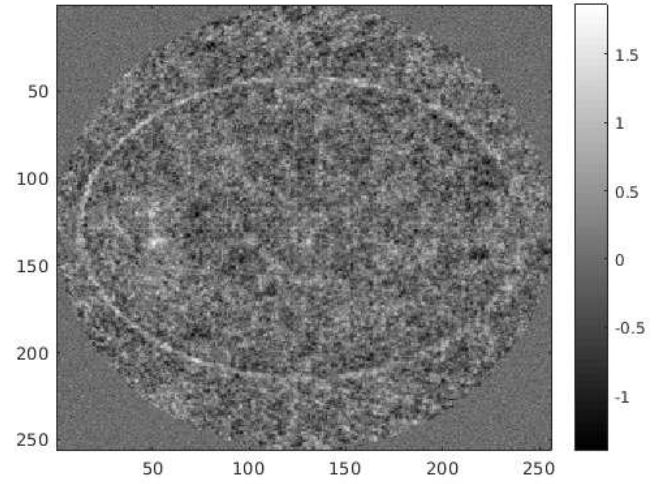
Figure 3.18: Estimated dual variable z (see algorithm 7) in PDFW [OMBF18] with the matched SF pair. The variable is size of the volume.
