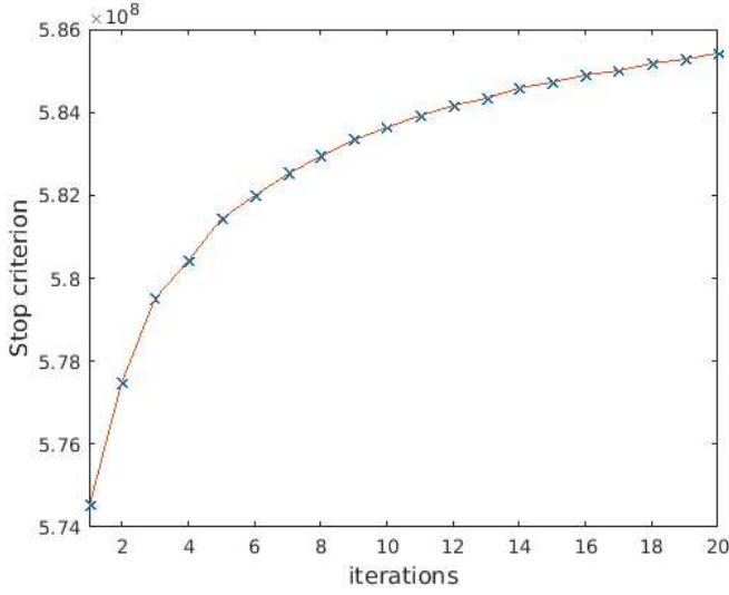
Figure 6.8: Convergence of the VBA algorithm
