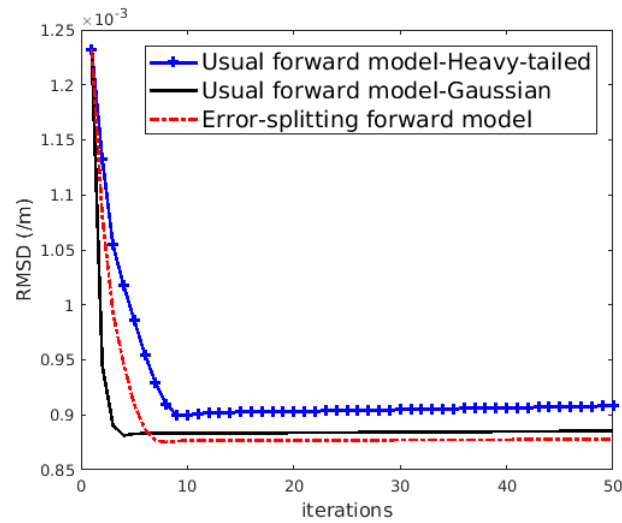
Figure 5.11: Convergence to the reference volume for IQI reconstruction by JMAP from 300 projections with Gauss-Markov-Potts prior and : the usual forward model modelling \zeta as heavy-tailed, the usual forward model modelling \zeta as Gaussian, and the error-splitting forward model
