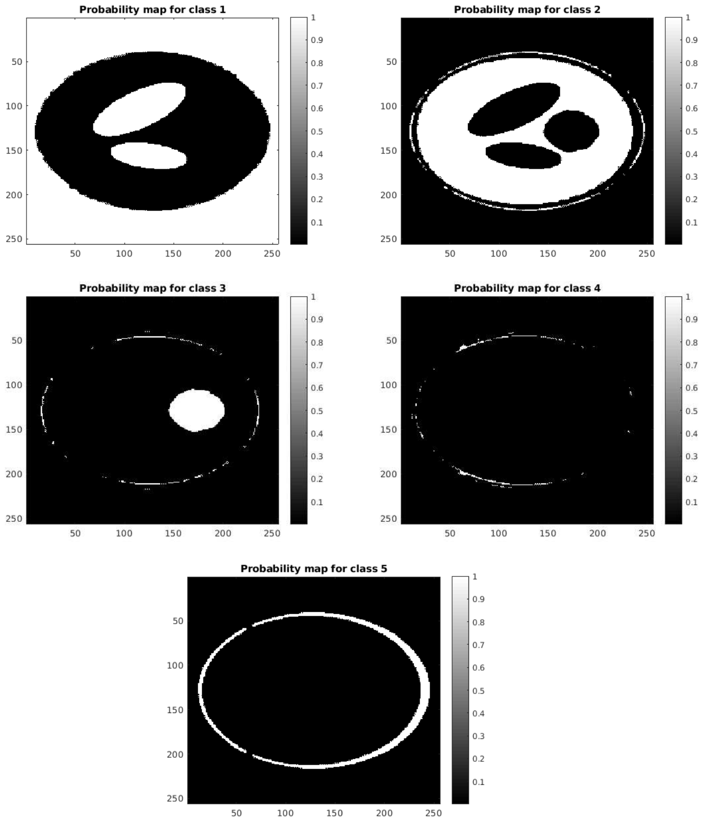
Figure 6.7: Probability maps for each voxel to be in each class, estimated by the VBA algorithm
