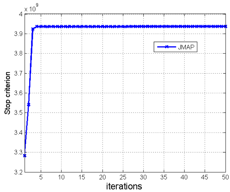
Figure 4.21: Convergence of JMAP for the joint reconstruction and segmentation of CMTE from 300 projections
