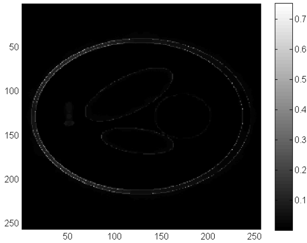
Figure 3.15: Difference between the original volume and the reconstruction by PDFW, with the unmatched RD/VD pair
