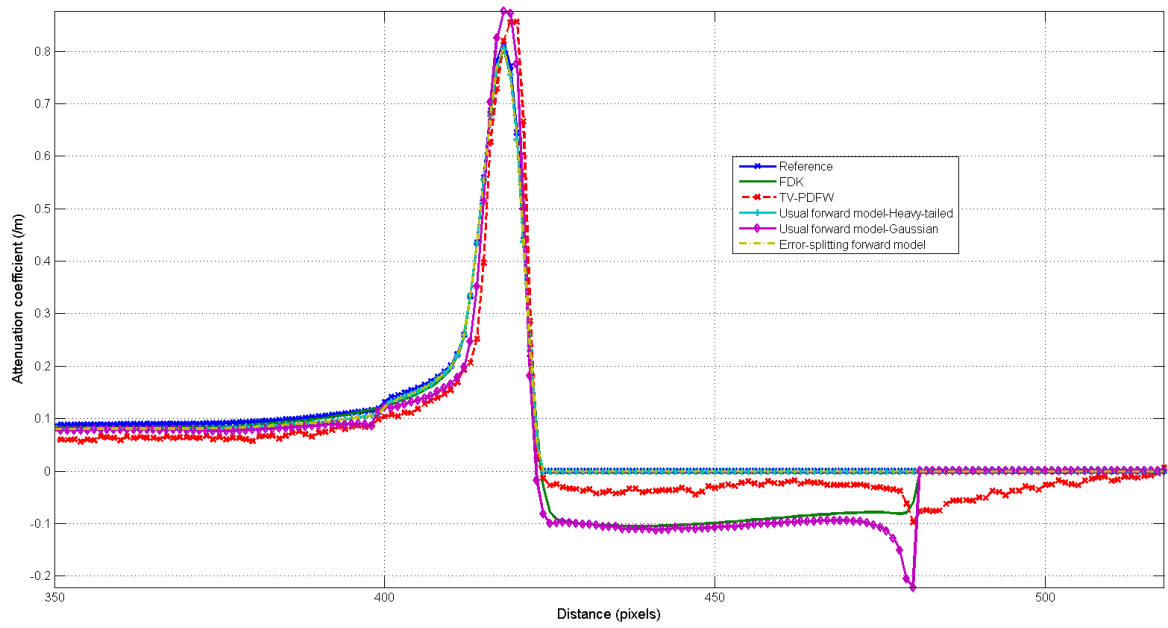
Figure 5.17: Profile of the CMTE volume for each reconstruction, with Gauss-Markov-Potts prior for JMAP
