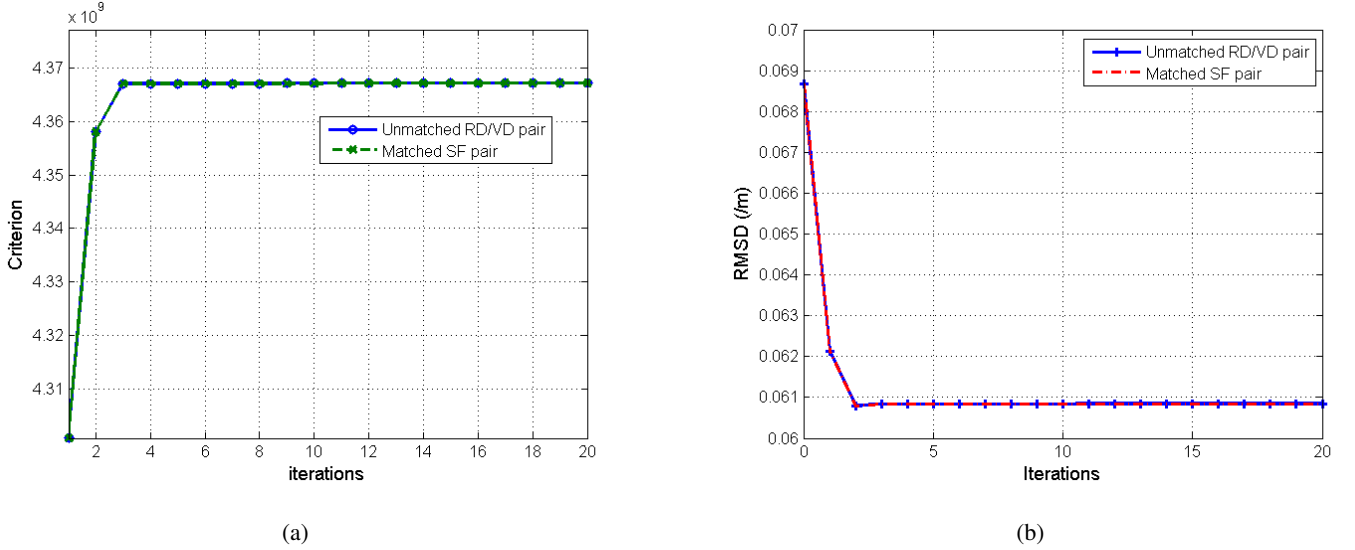
Figure 4.9: Convergence metrics for JMAP (stopping criterion (a) and RMSD with respect to the real phantom (b)), with the unmatched RD/VD pair and the matched SF pair
