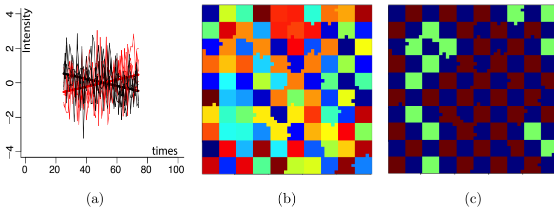
Figure 3.6: Local and global segmentation of shrunken Chessboard image sequence: (a) the shrunken true and observed observed TCs; (b) local clustering of shrunken chessboard with 2 clusters: the color map of 89 local clusters from local clustering; (c) global clustering of shrunken chessboard with 2 global clusters: the color map of 3 global clusters from global clustering.
