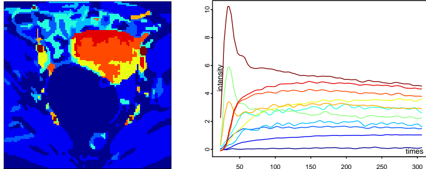
Figure 4.1: Synthetic DCE image sequence: (left) The ground-truth segmentation of \mathcal{X} ; (right) The true enhancement curves, i^x(t) , associated to the 11 clusters using corresponding colors.
