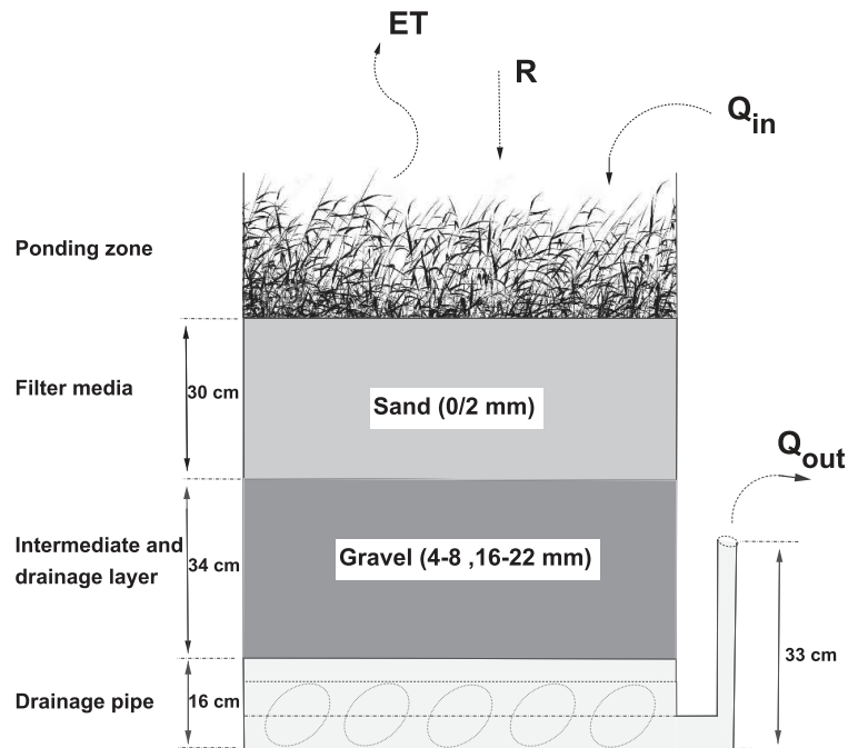
Figure 5.9: Numerical diagram of the CW : rainfall (R), inflow (Q in ), evapotranspiration rate (ET) and the outflow from drainage pipe (Q out )
