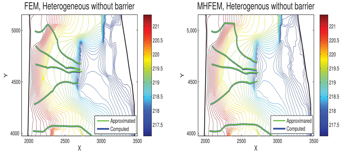
Figure 3.17: Piezometric head and streamlines (blue lines) computed with a leakage coefficient of 9 \text{ m}^{-1} \text{ d}^{-1} and approximated streamlines (green lines) computed with (C_\lambda, \delta_{C_\lambda}) = (6 \text{ m}^{-1} \text{ d}^{-1}, 3 \text{ m}^{-1} \text{ d}^{-1}) . Heterogeneous transmissivity, case without barrier.
